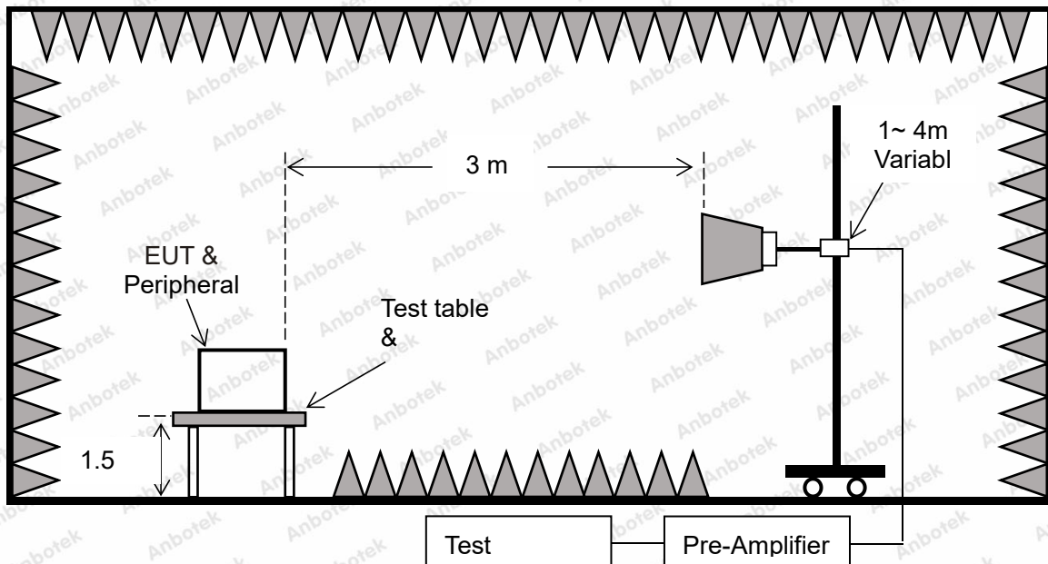
Figure 3. Above 1 GHz
