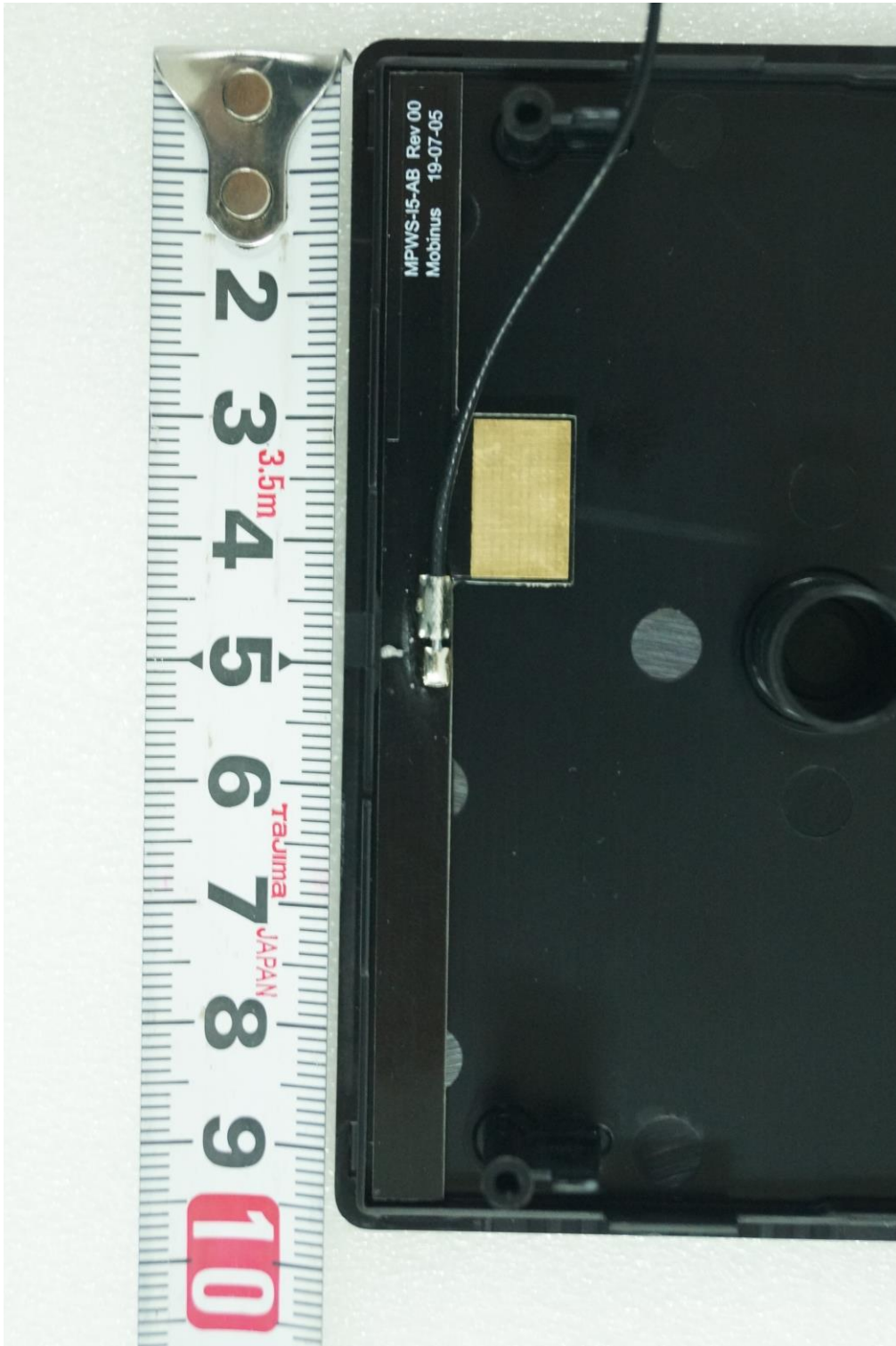
< Antenna view >
