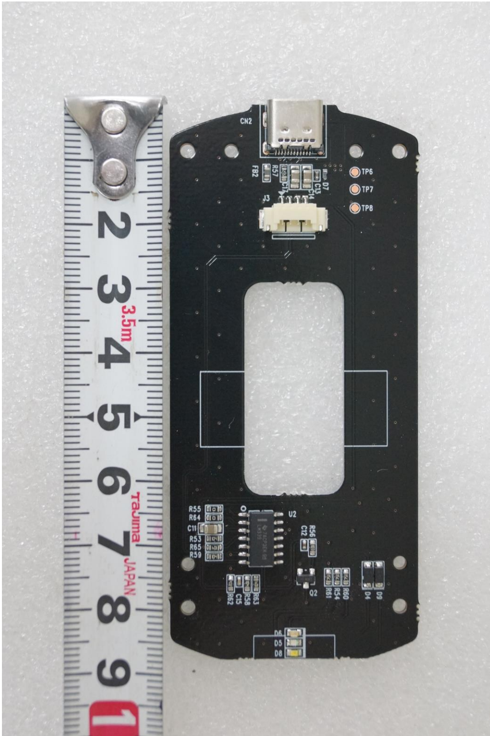
< Charging cradle main board Top view >
