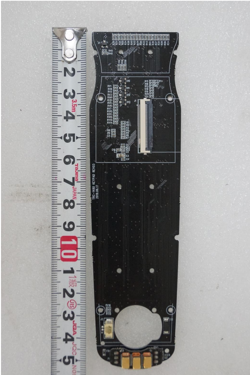
< Keypad board bottom view >
