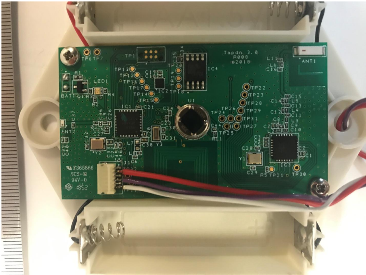
Figure 2. EUT, PCB, Front
