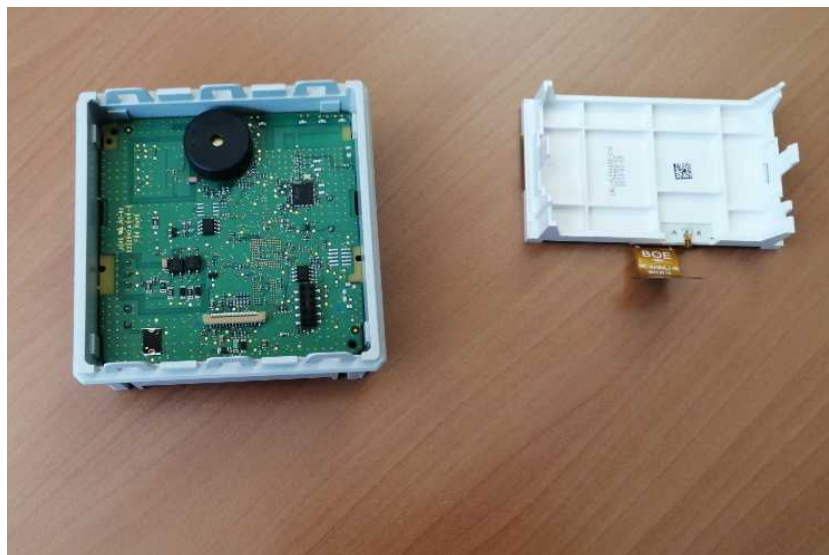
Photo 2 - unmounted PCB
