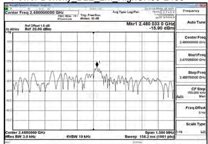
Power Density_BLE_2M_HighCH39-2480
