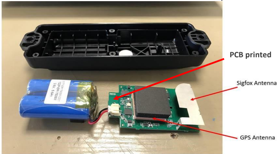
2) Disassembled View
