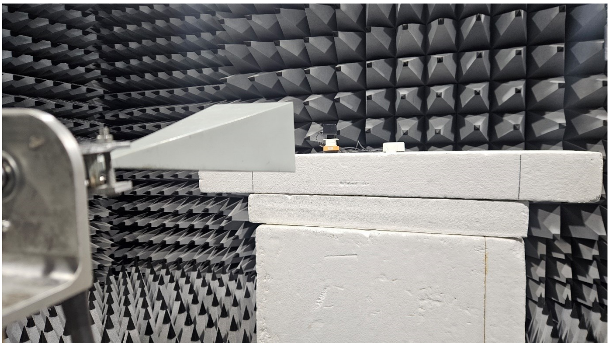
Radiated Emissions 18GHz to 26.5GHz
