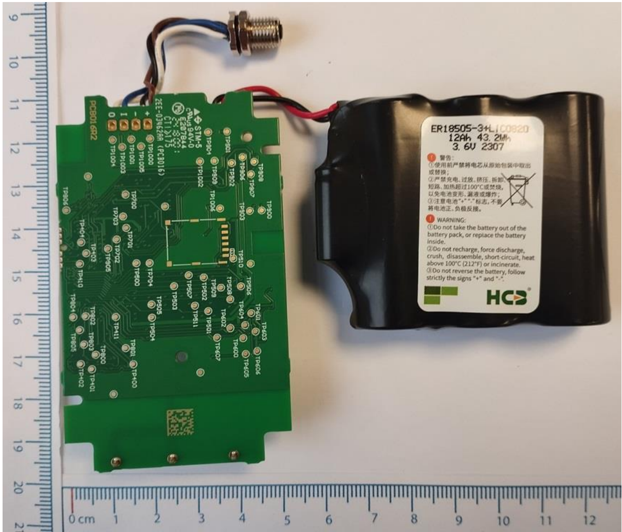
Figura 6: Side B - Hati Battery- External DC power supply connector Hati
