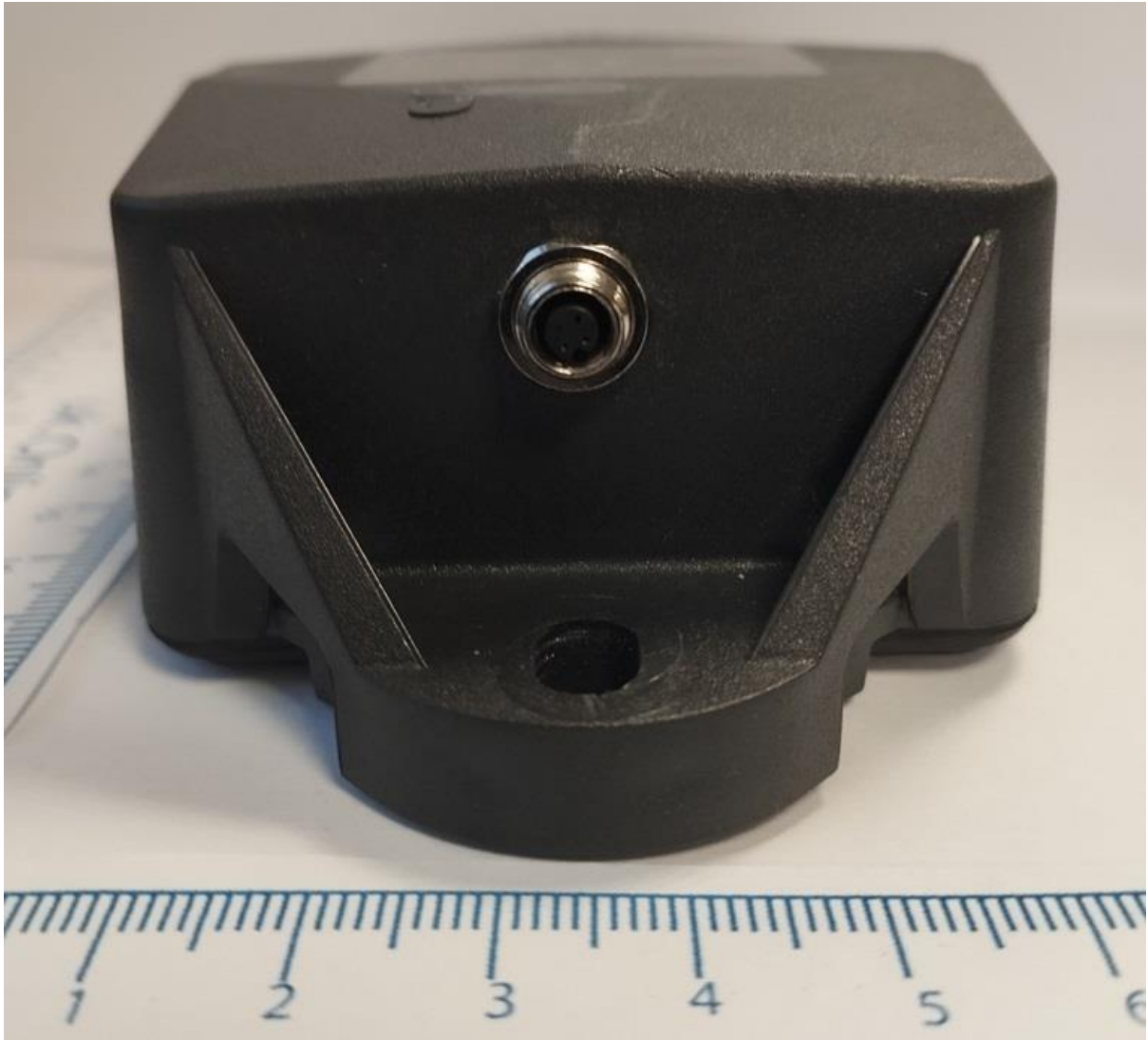
Figure 12: Bottom View - Cover View – showing External DC power supply connector.
