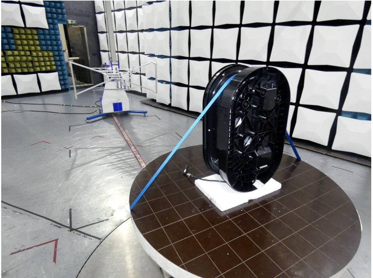
Photo 2: Test setup for radiated measurements in semi anechoic chamber 30 MHz – 1 GHz
