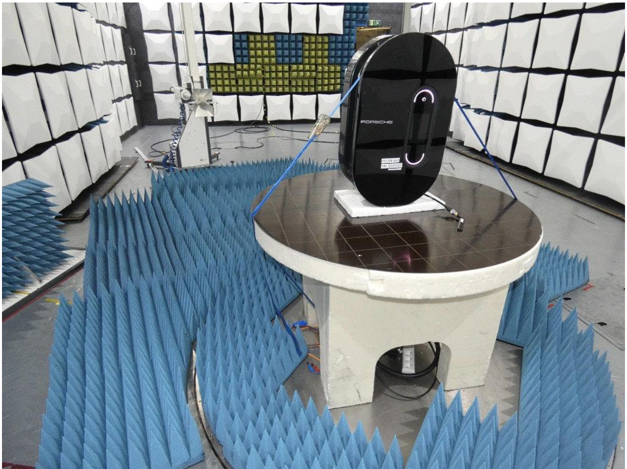
Photo 3: Test setup for radiated measurements in semi anechoic chamber 1 GHz – 18 GHz
