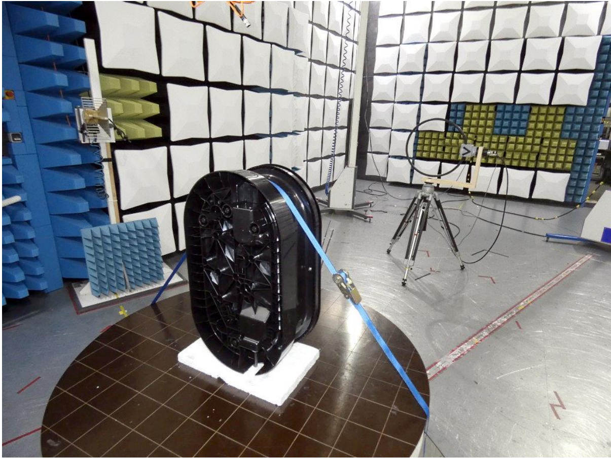
Photo 1: Test setup for radiated measurements 9 kHz – 30 MHz
