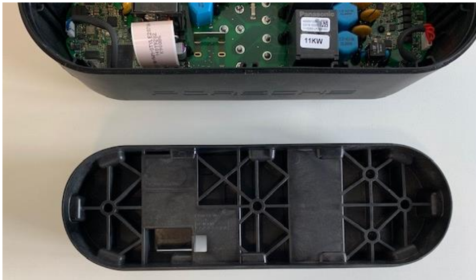
Top view holding frame: Model IC-CPD
