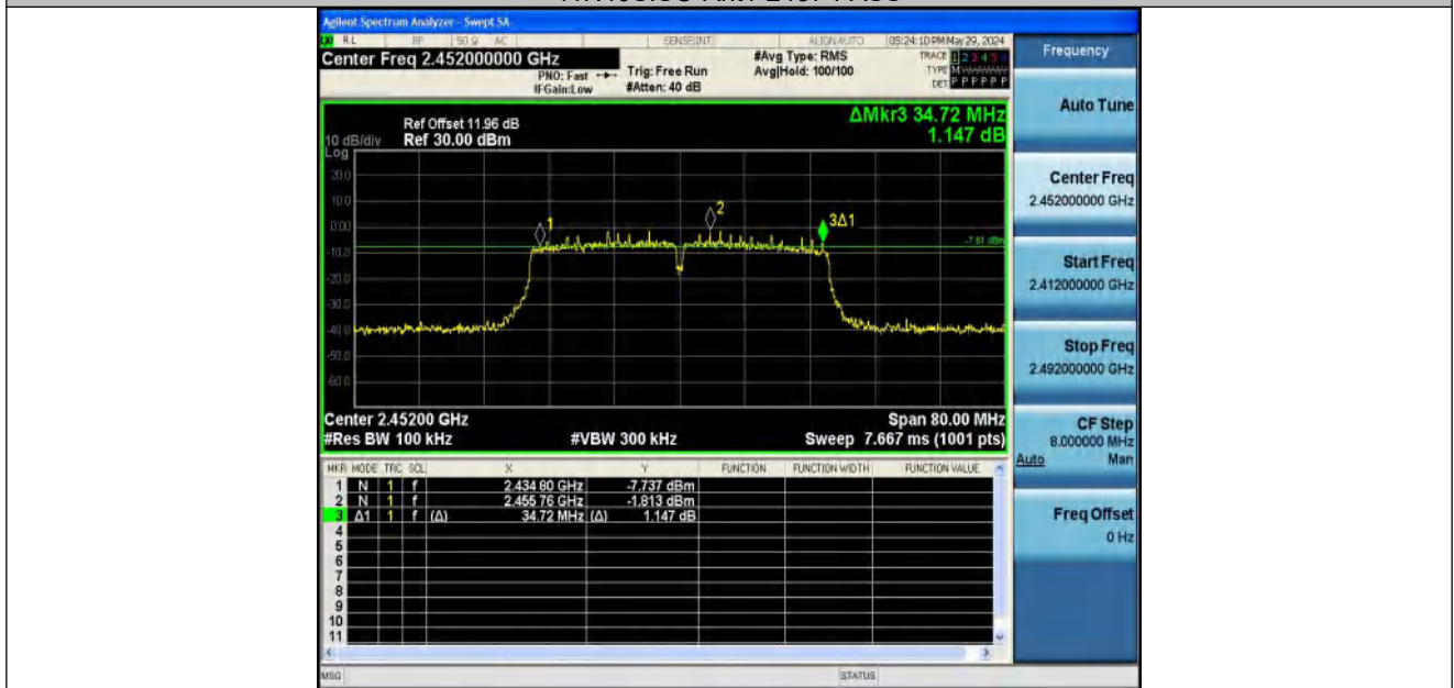
11N40SISO-Ant1-2452-PASS
