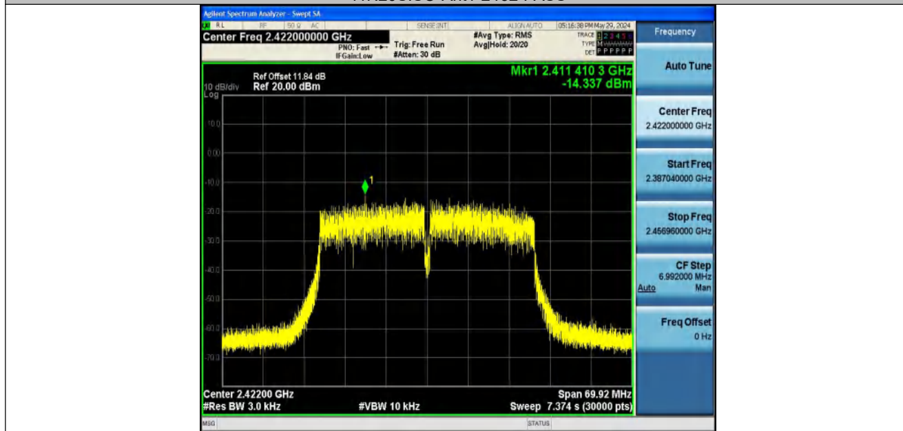
11N40SISO-Ant1-2422-PASS
