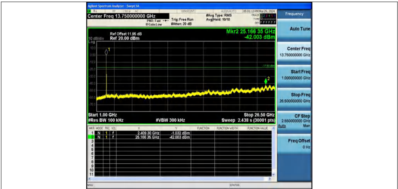
11N20SISO-Ant1-2412-1000~26500-PASS
