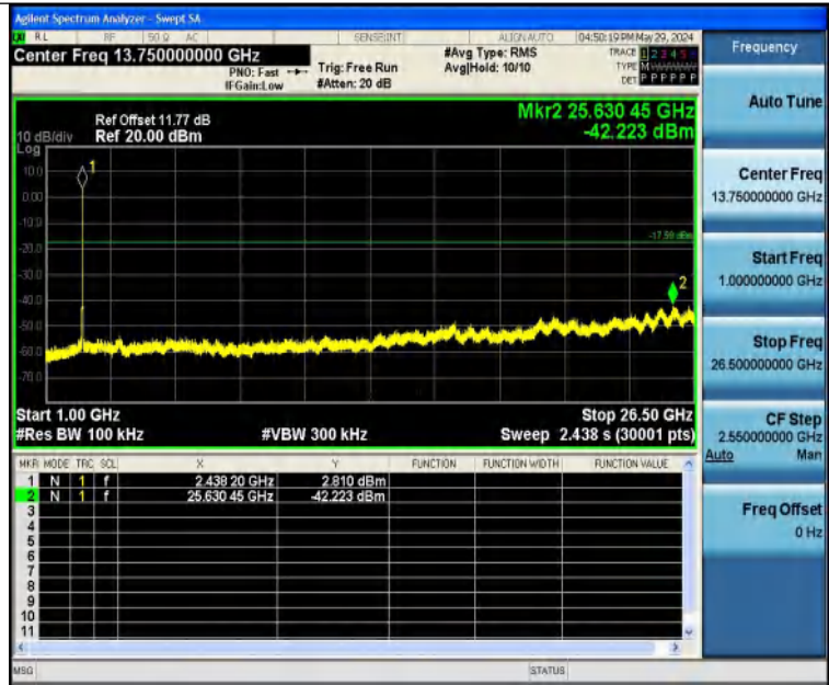
11G-Ant1-2437-1000~26500-PASS
