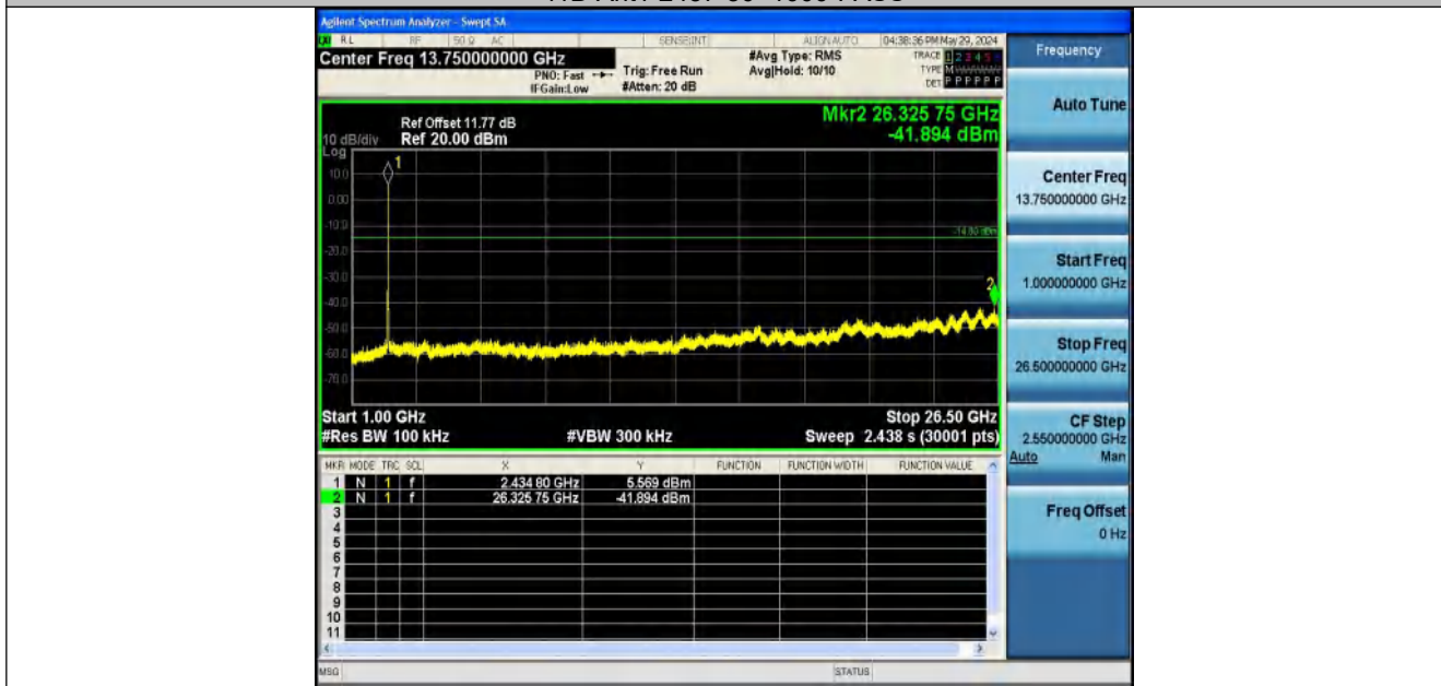
11B-Ant1-2437-1000~26500-PASS
