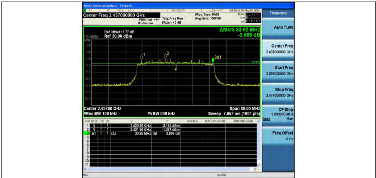
11N40SISO-Ant1-2437-PASS
