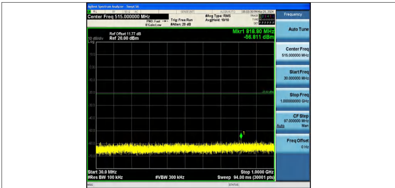
11N20SISO-Ant1-2437-30~1000-PASS
