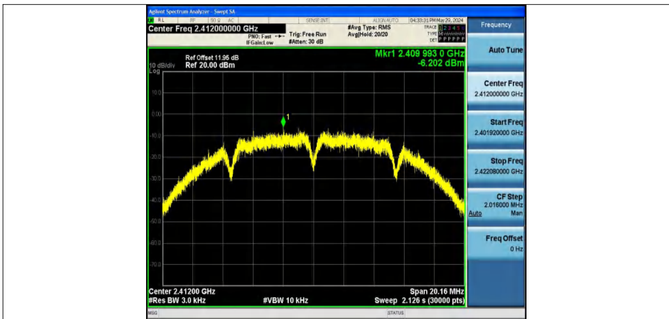
11B-Ant1-2412-PASS
