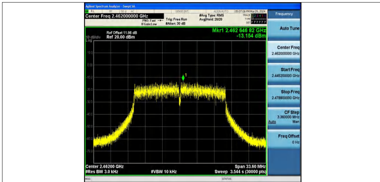
11N20SISO-Ant1-2462-PASS
