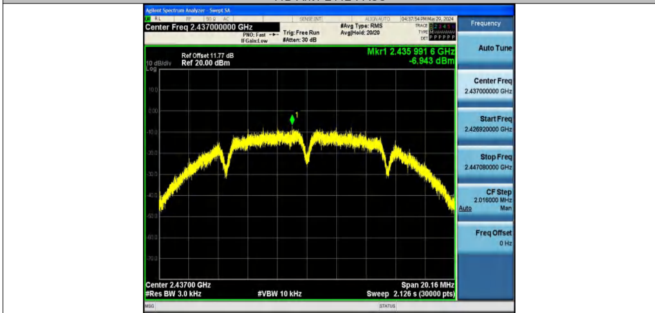
11B-Ant1-2437-PASS
