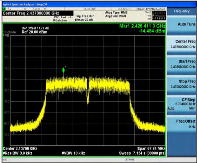
11N40SISO-Ant1-2437-PASS
