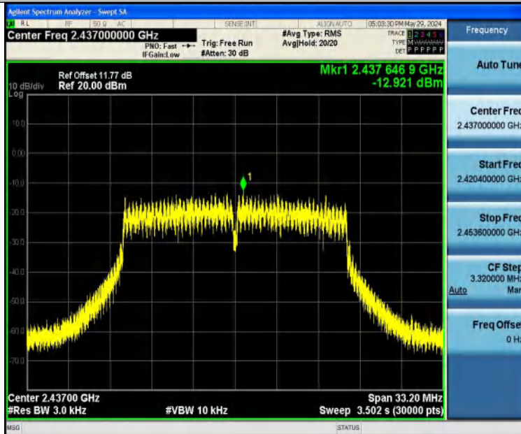
11N20SISO-Ant1-2437-PASS
