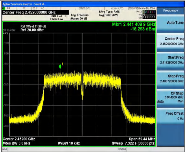
11N40SISO-Ant1-2452-PASS
