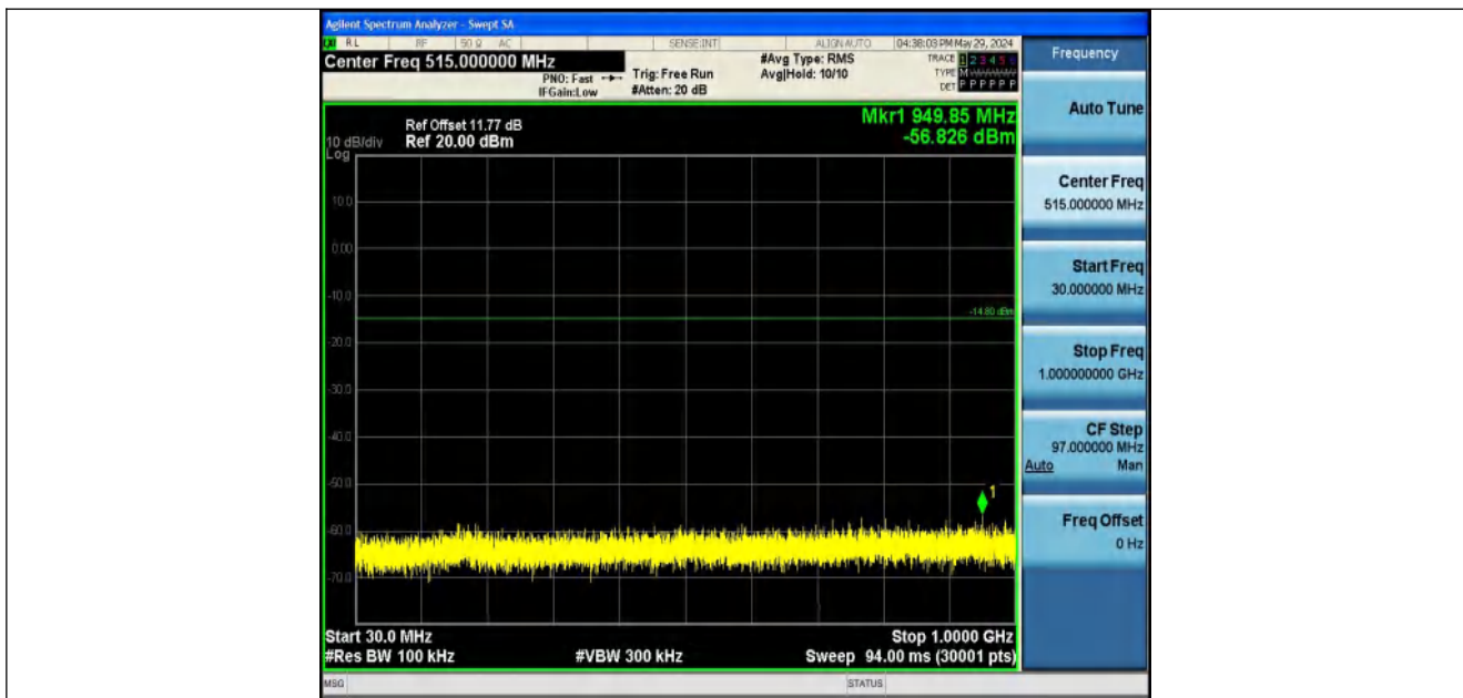
11B-Ant1-2437-30~1000-PASS
