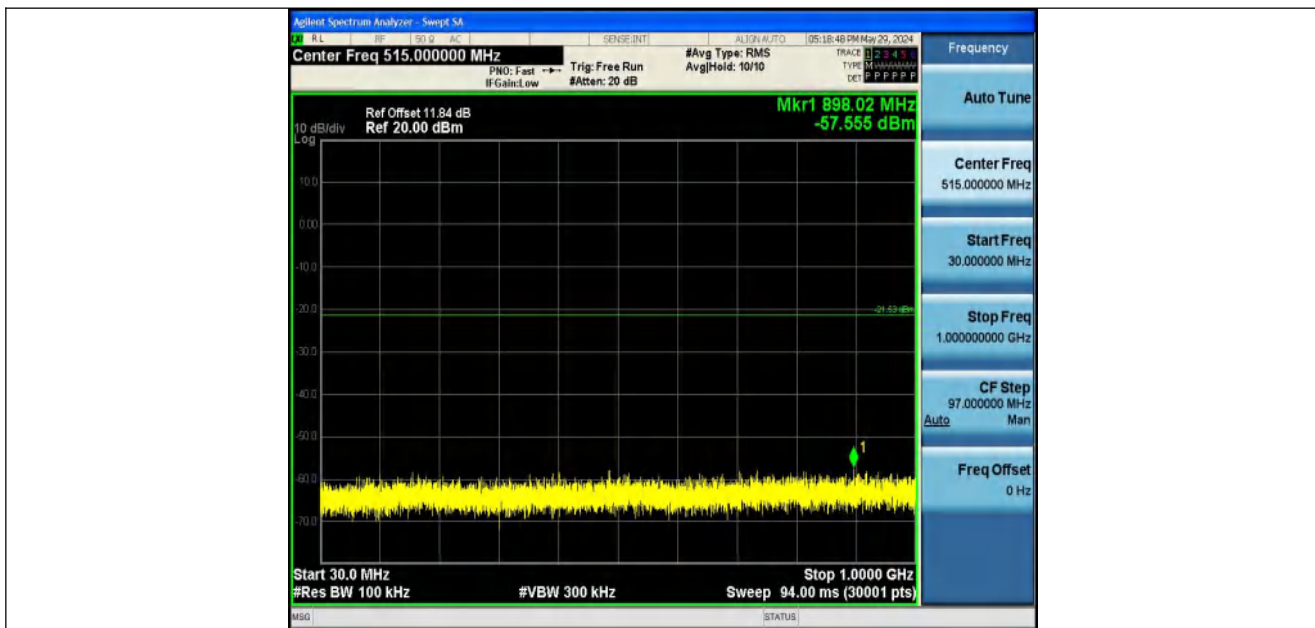
11N40SISO-Ant1-2422-30~1000-PASS
