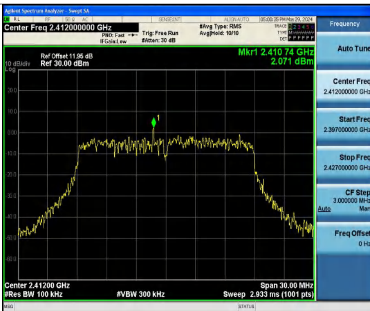
11N20SISO-Ant1-2412-0~Reference-PASS
