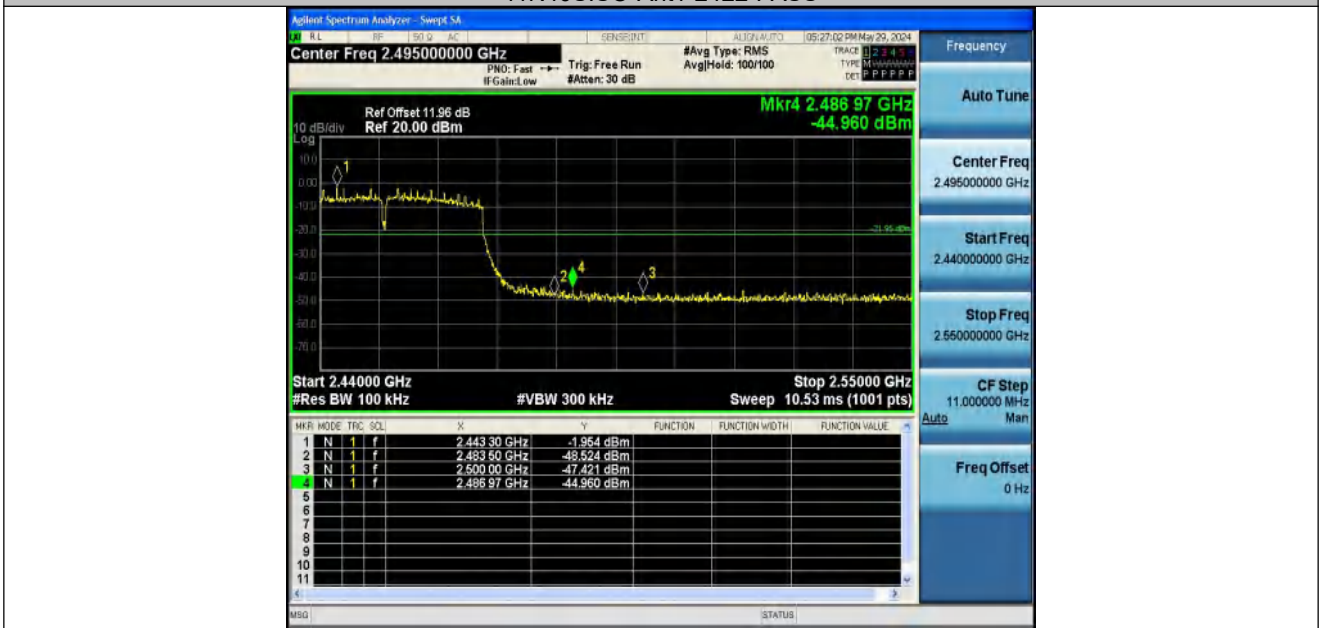
11N40SISO-Ant1-2452-PASS
