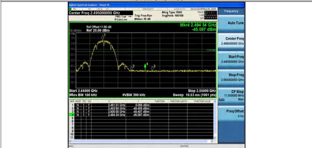
11B-Ant1-2462-PASS
