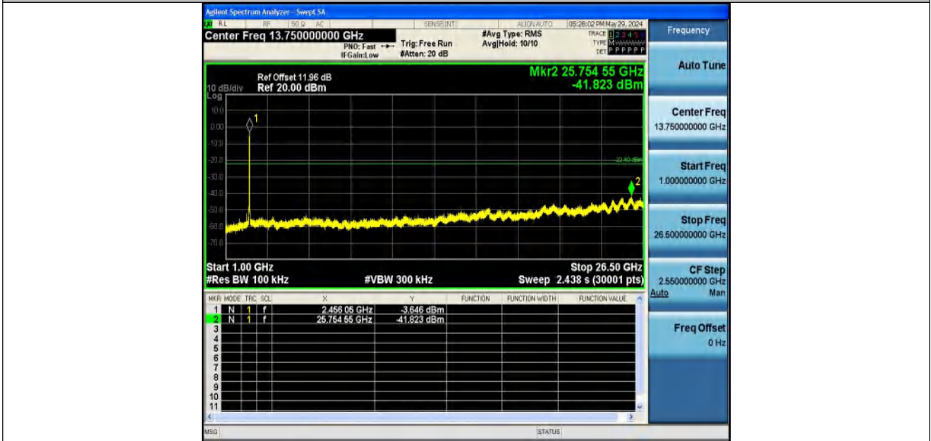
11N40SISO-Ant1-2452-1000~26500-PASS
