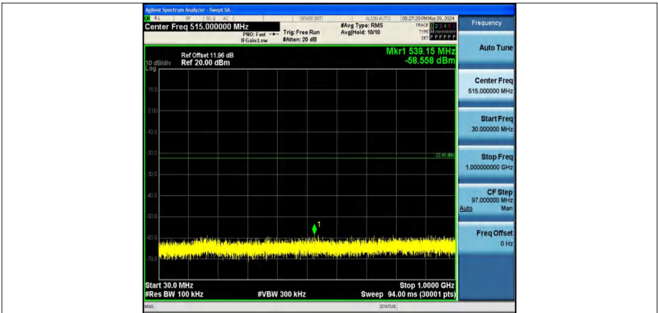
11N40SISO-Ant1-2452-30~1000-PASS
