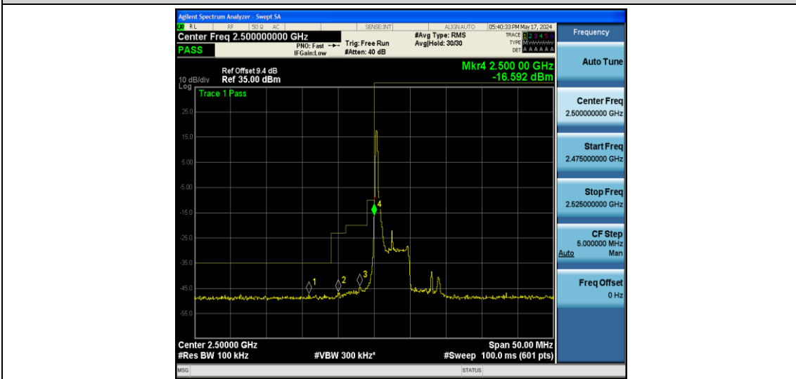
Band7-5MHz-16QAM-20775-1RB#24
