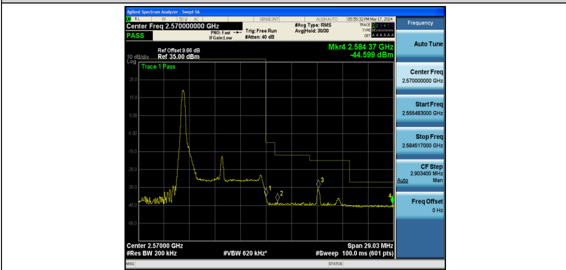
Band7-10MHz-16QAM-21400-1RB#49
