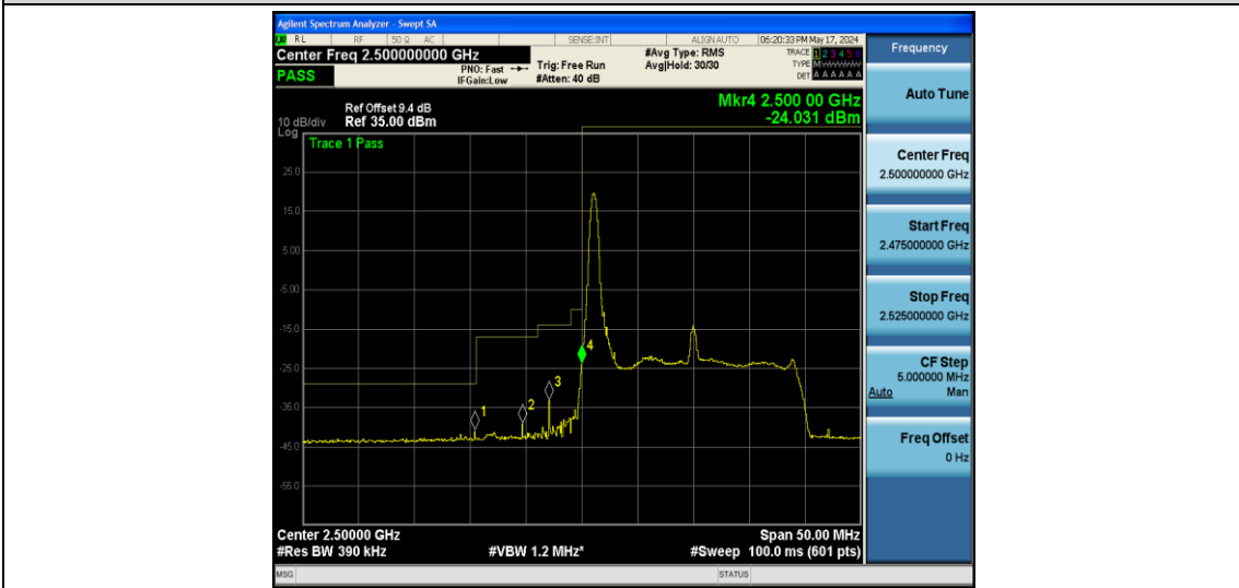
Band7-20MHz-QPSK-20850-1RB#99
