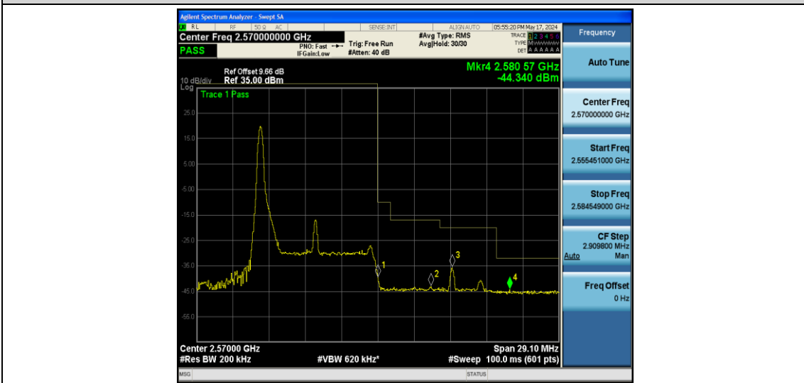
Band7-10MHz-QPSK-21400-1RB#49
