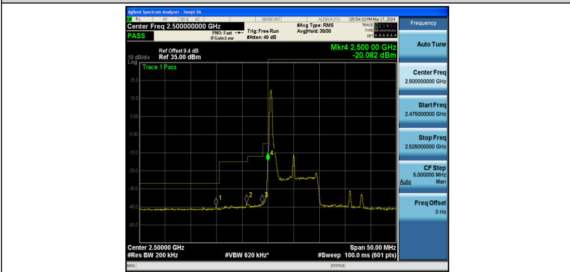
Band7-10MHz-16QAM-20800-1RB#49
