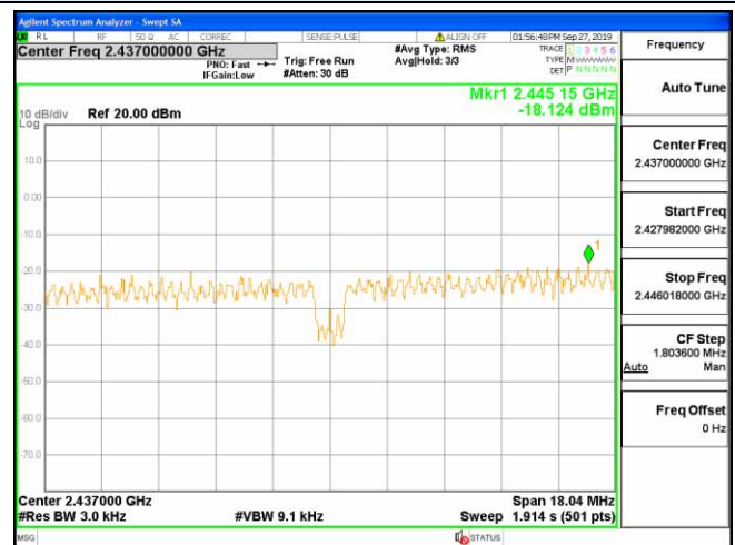
Channel 6 / 2437 MHz
