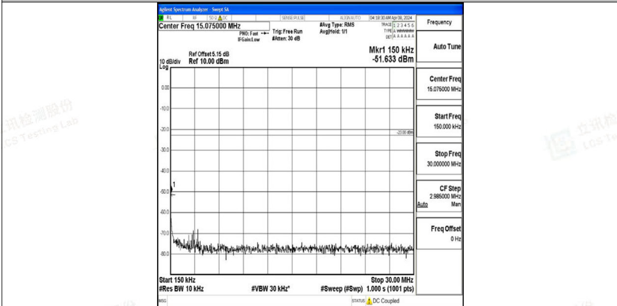
Band12_10MHz_QPSK_23095_1RB#0_0.15~30_0.15~30
