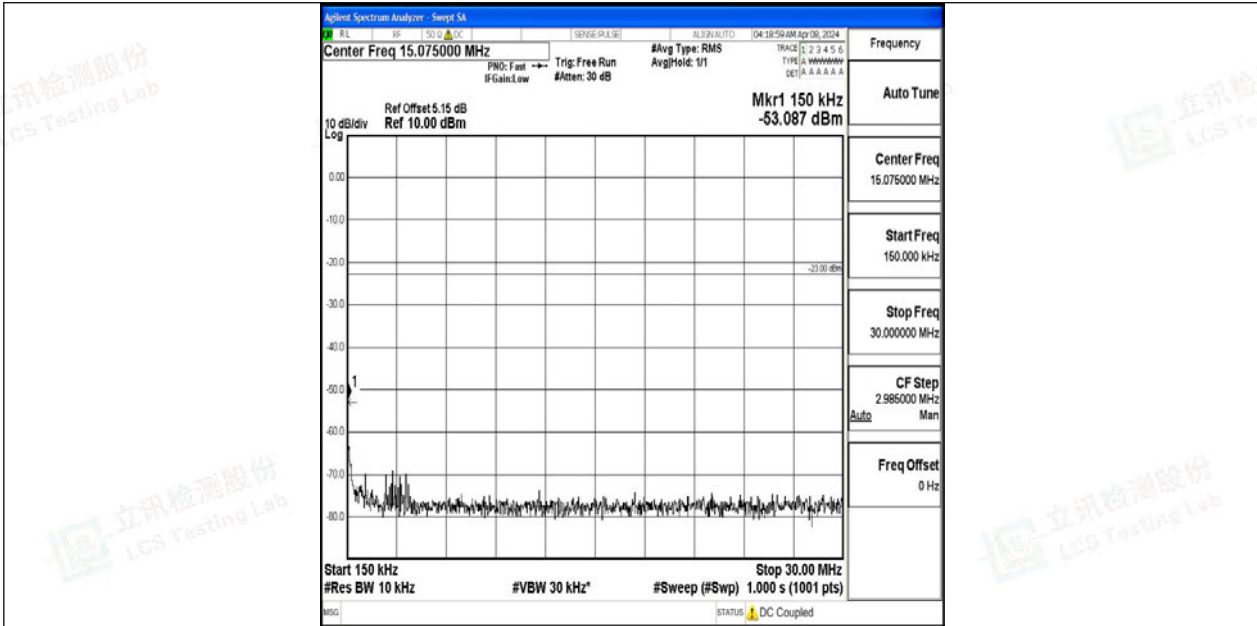
Band12_10MHz_64QAM_23095_1RB#0_0.15~30_0.15~30
