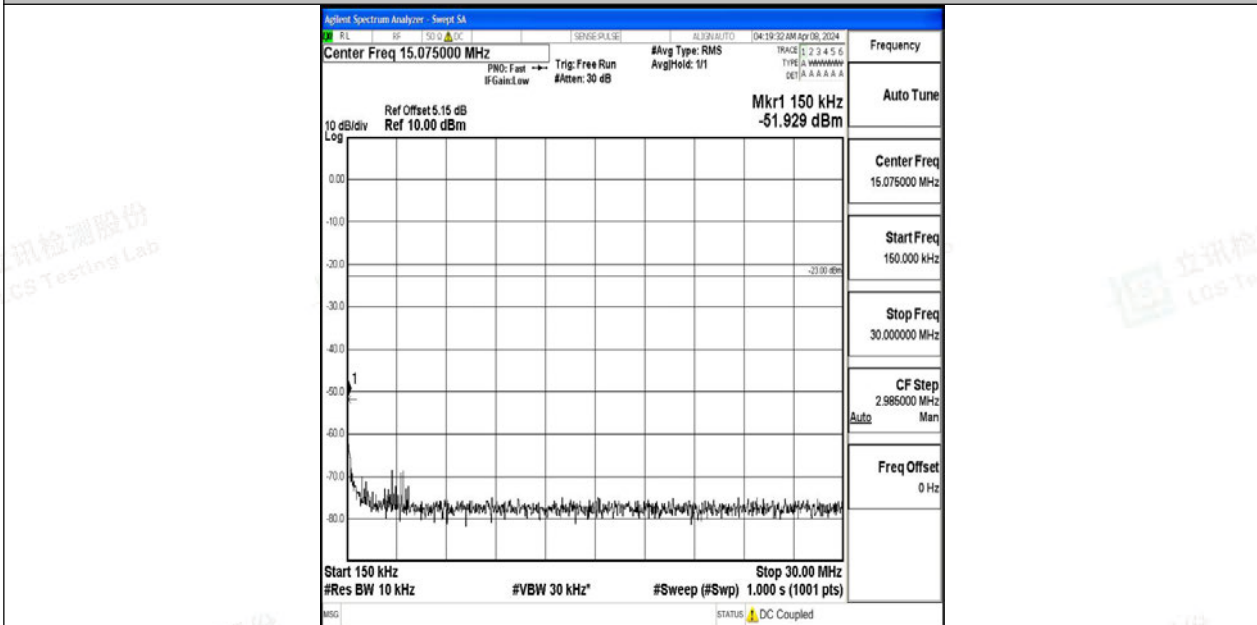
Band12_10MHz_QPSK_23130_1RB#0_0.15~30_0.15~30
