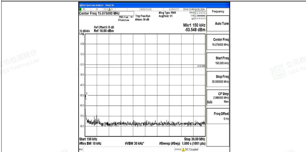
Band12_3MHz_QPSK_23095_1RB#0_0.15~30_0.15~30
