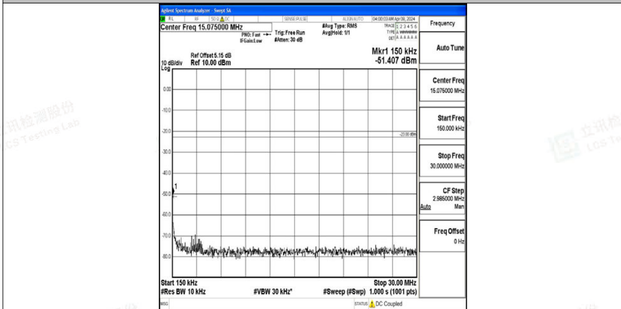
Band12_5MHz_QPSK_23095_1RB#0_0.15~30_0.15~30
