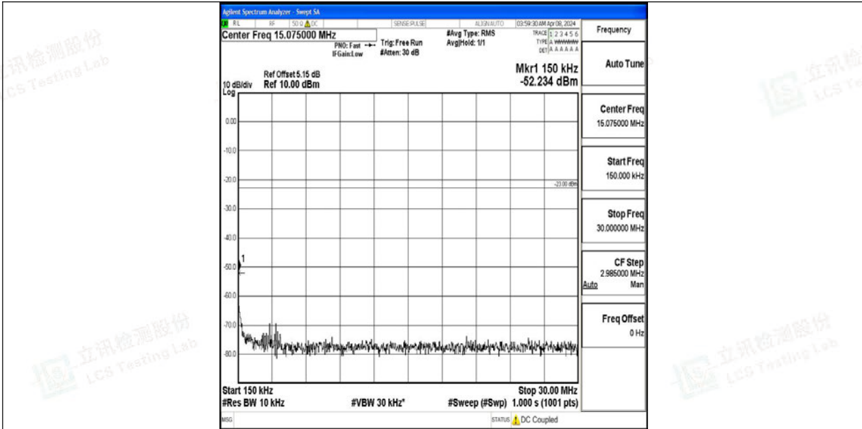
Band12_5MHz_64QAM_23035_1RB#0_0.15~30_0.15~30
