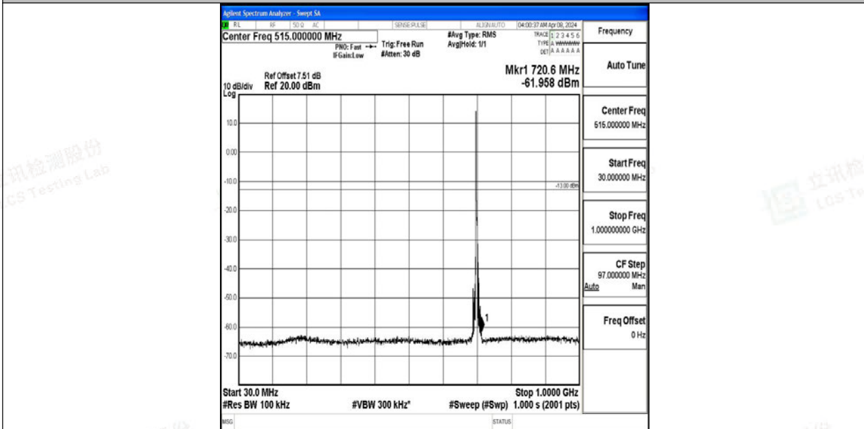
Band12_5MHz_64QAM_23095_1RB#0_30~1000_30~1000
