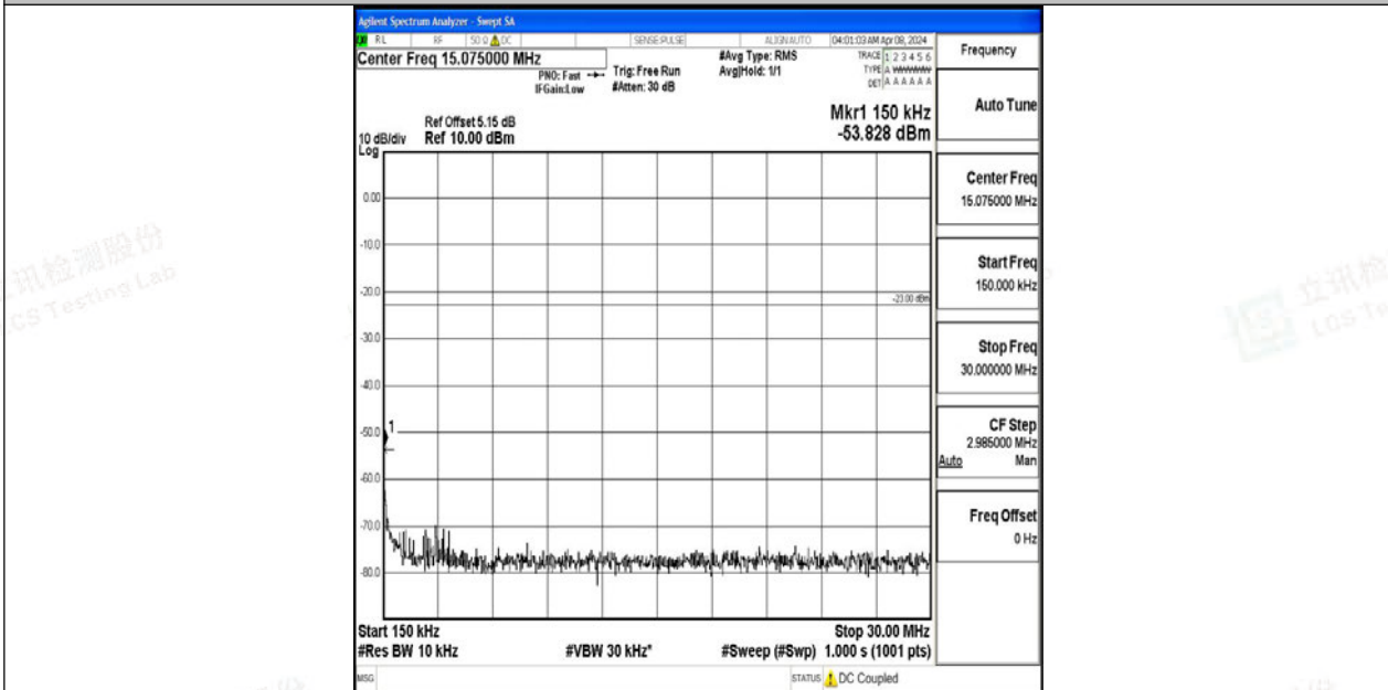
Band12_5MHz_QPSK_23155_1RB#0_0.15~30_0.15~30
