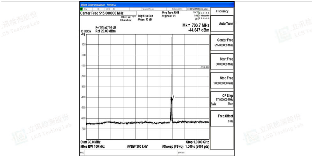
Band12_1.4MHz_QPSK_23017_1RB#0_30~1000_30~1000
