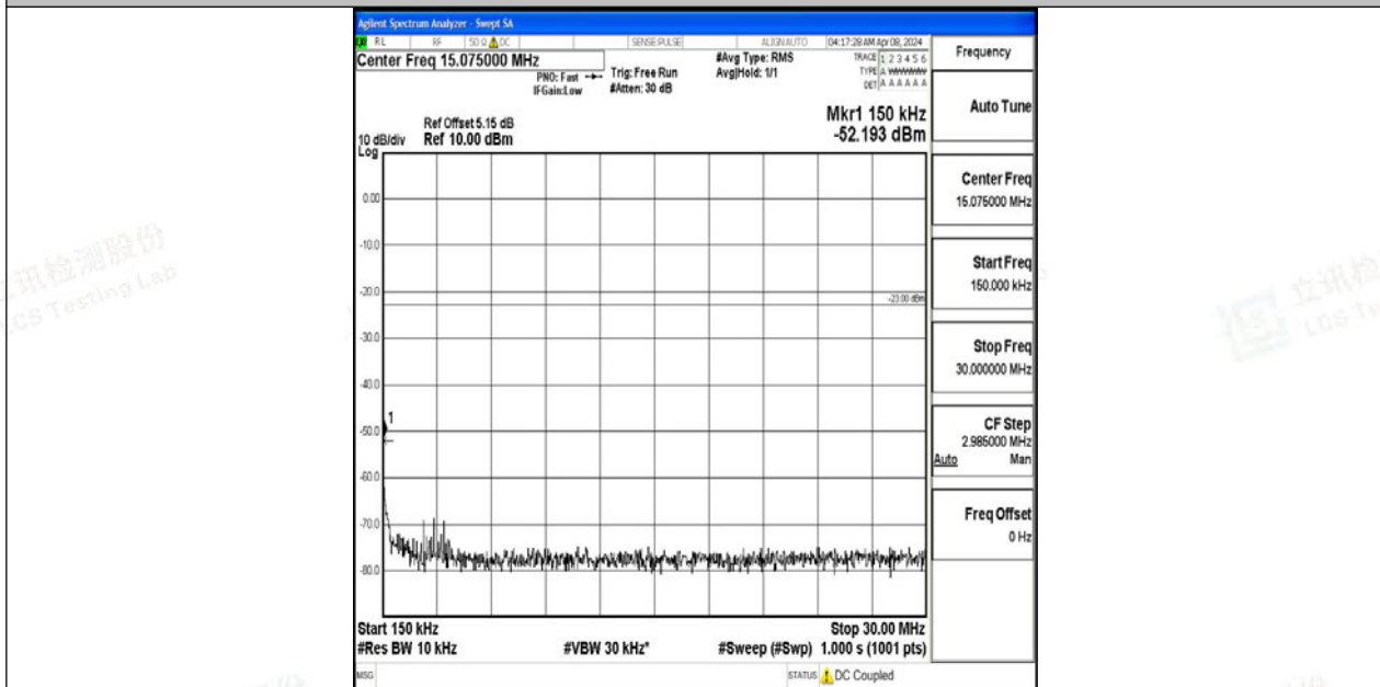
Band12_10MHz_QPSK_23060_1RB#0_0.15~30_0.15~30
