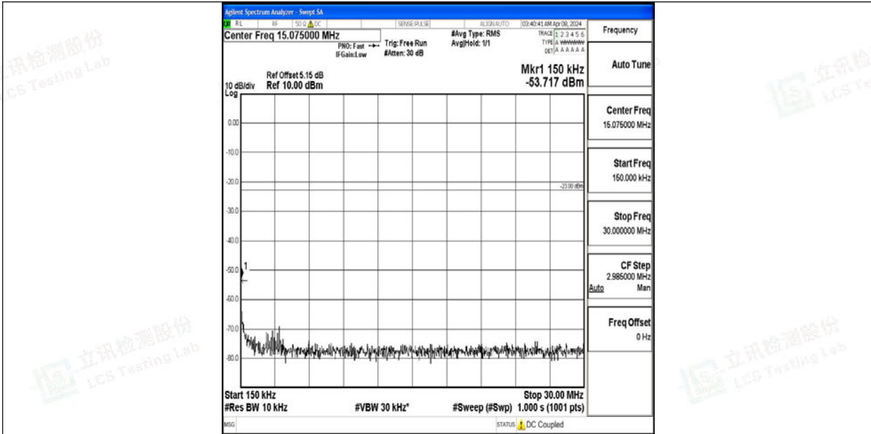
Band12_3MHz_64QAM_23025_1RB#0_0.15~30_0.15~30
