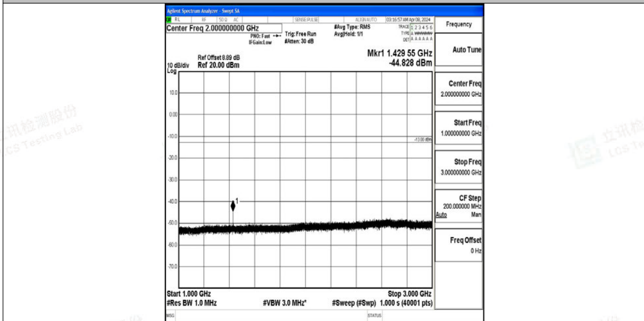
Band12_1.4MHz_QPSK_23173_1RB#0_1000~3000_1000~3000
