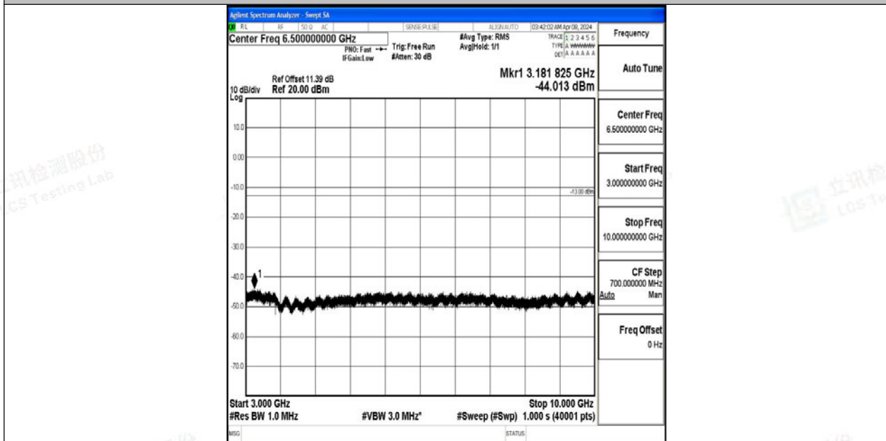
Band12_3MHz_64QAM_23095_1RB#0_3000~10000_3000~10000
