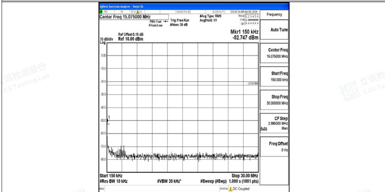
Band12_3MHz_QPSK_23165_1RB#0_0.15~30_0.15~30
