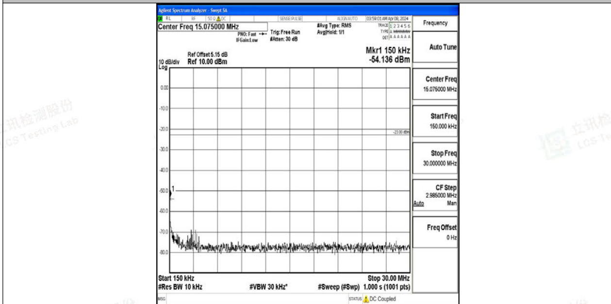
Band12_5MHz_QPSK_23035_1RB#0_0.15~30_0.15~30
