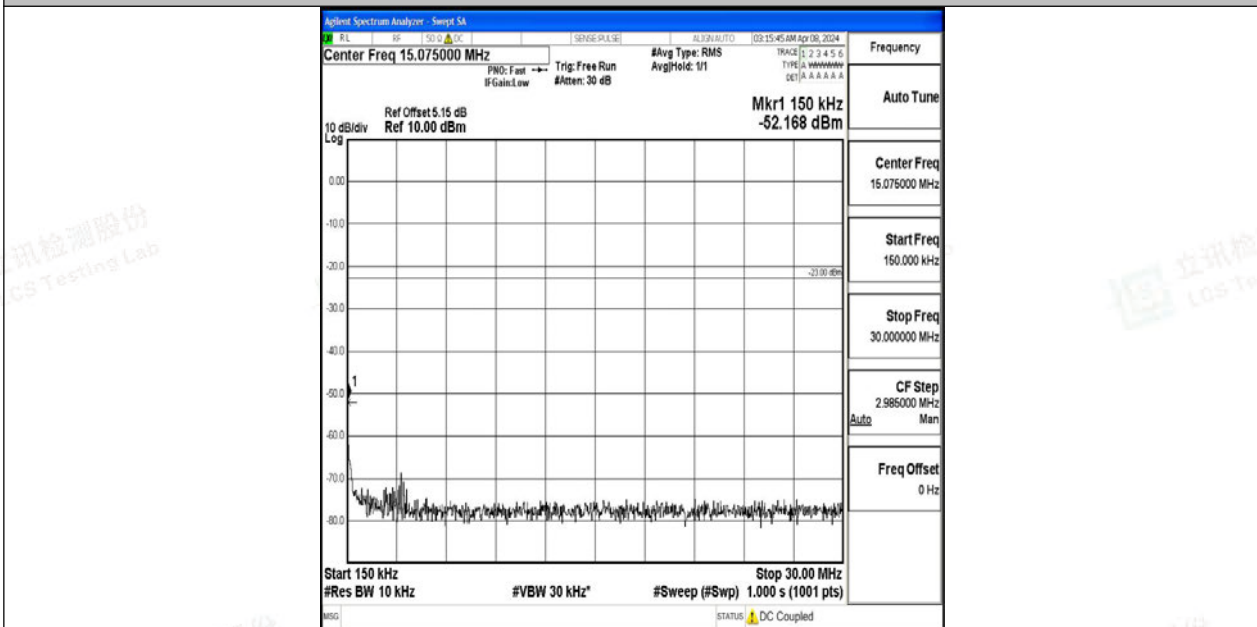
Band12_1.4MHz_QPSK_23095_1RB#0_0.15~30_0.15~30
