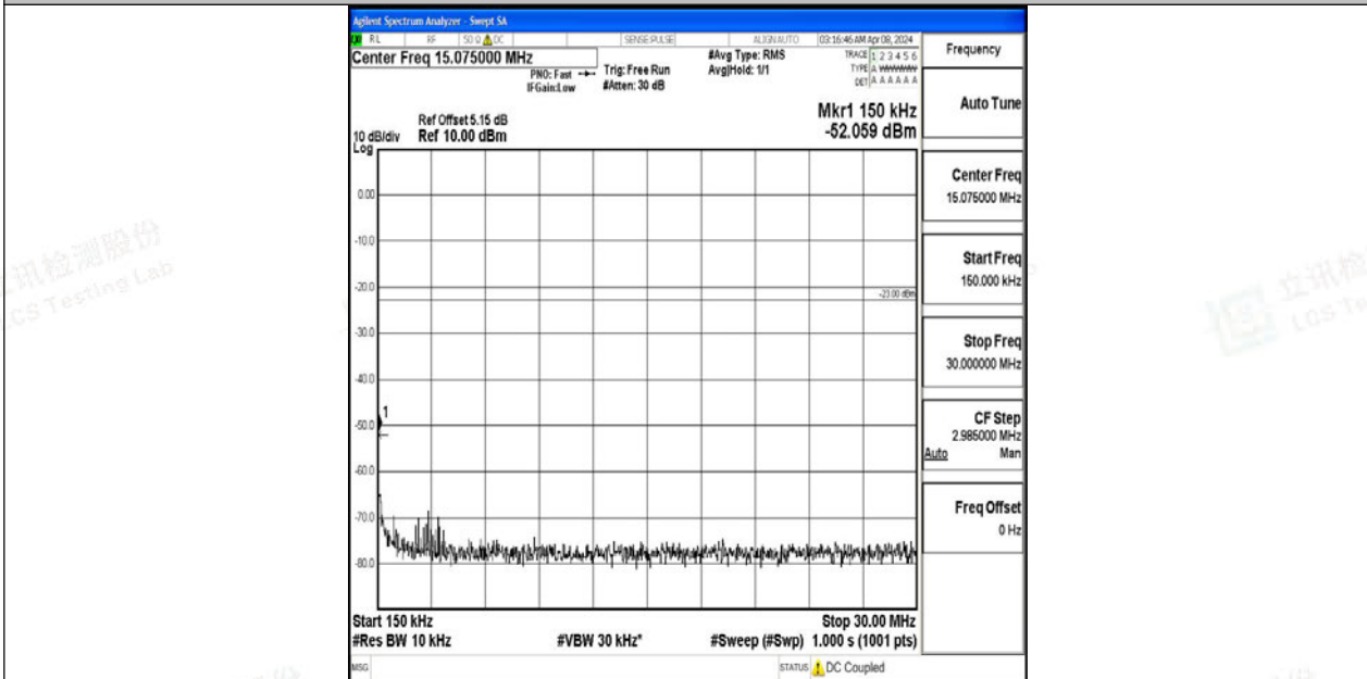
Band12_1.4MHz_QPSK_23173_1RB#0_0.15~30_0.15~30
