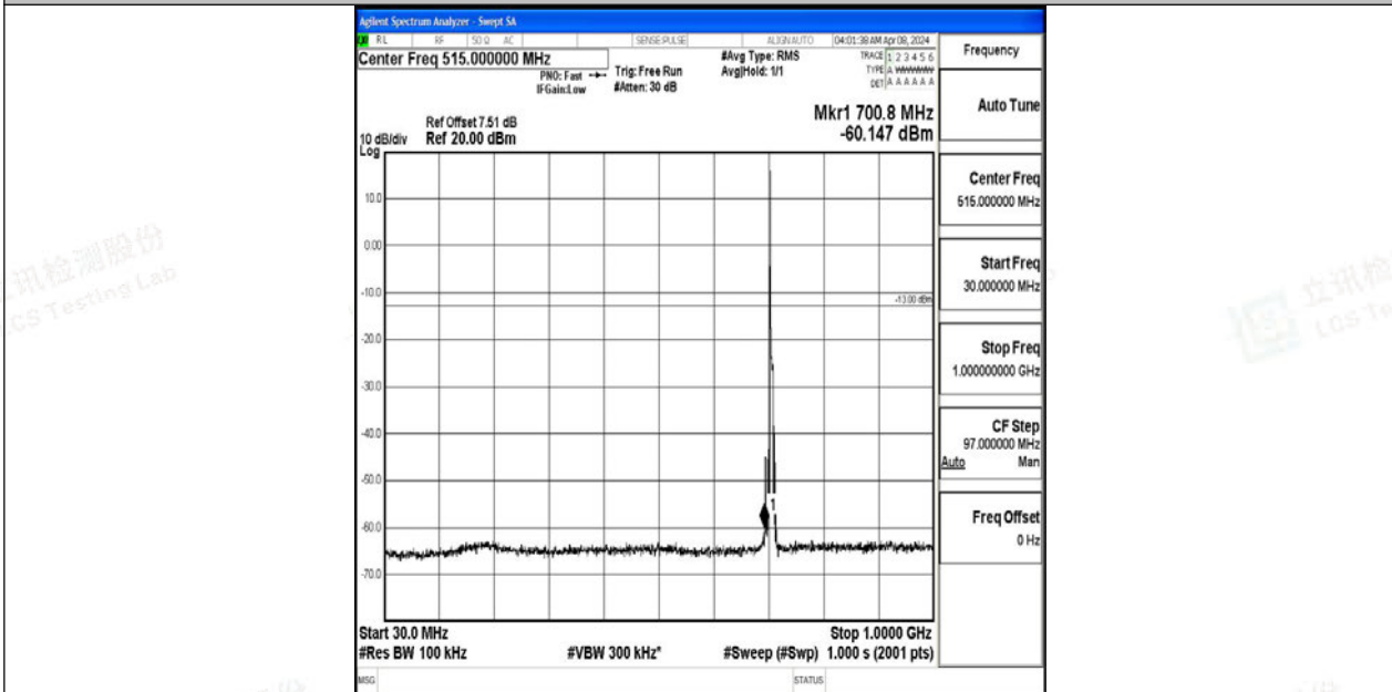
Band12_5MHz_64QAM_23155_1RB#0_30~1000_30~1000
