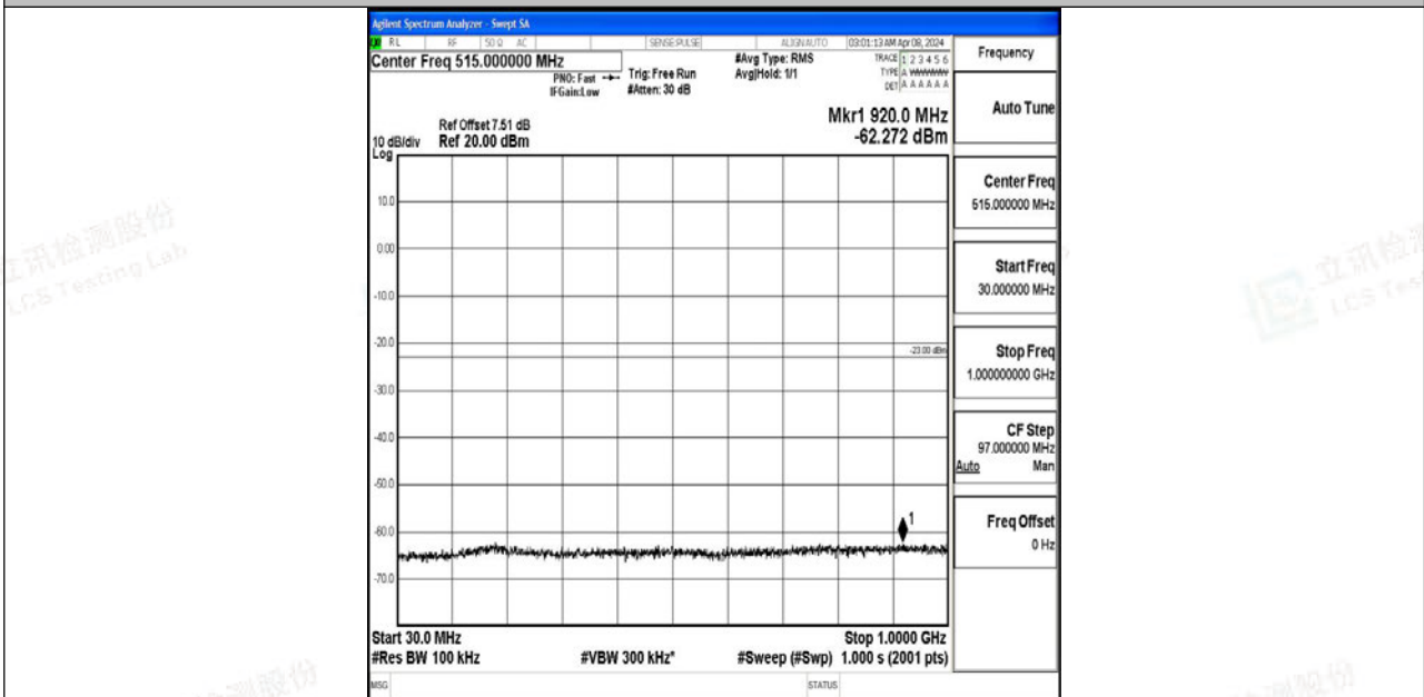
Band4_20MHz_QPSK_20300_1RB#0_30~1000_30~1000
