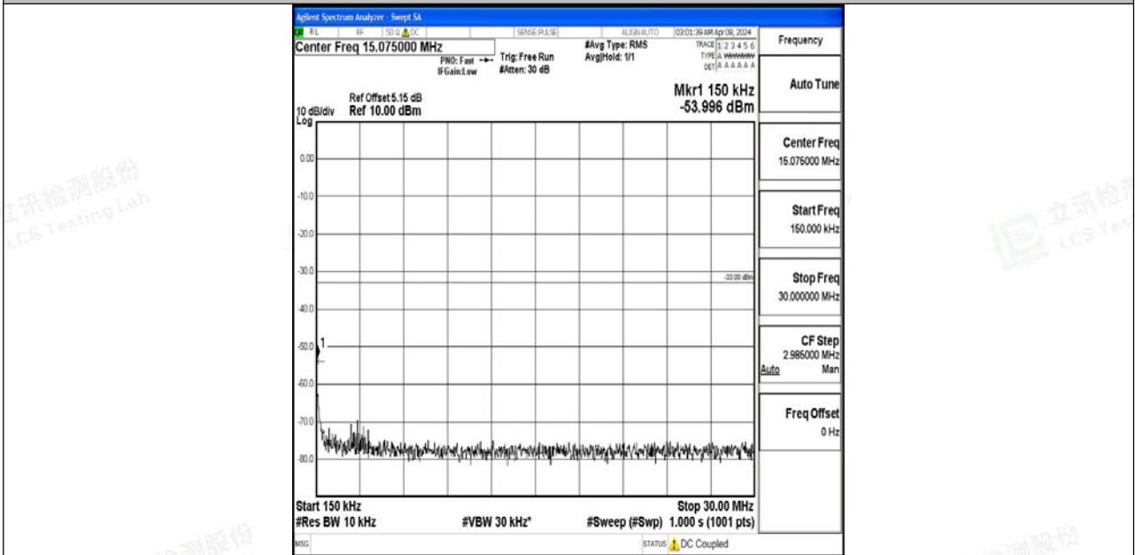
Band4_20MHz_64QAM_20300_1RB#0_0.15~30_0.15~30
