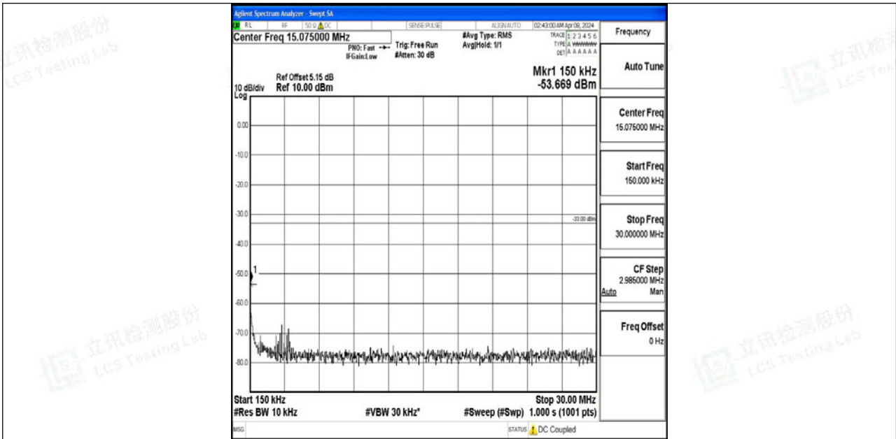
Band4_15MHz_QPSK_2025_1RB#0_0.15~30_0.15~30
