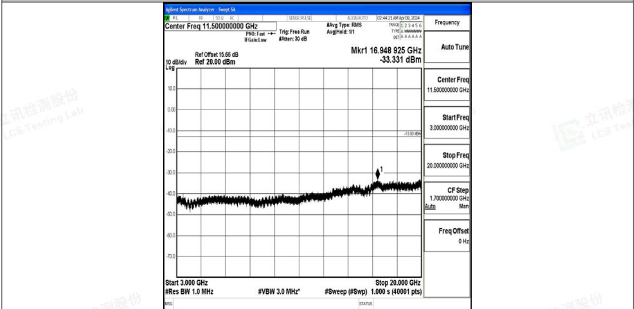
Band4_15MHz_QPSK_20175_1RB#0_3000~20000_3000~20000
