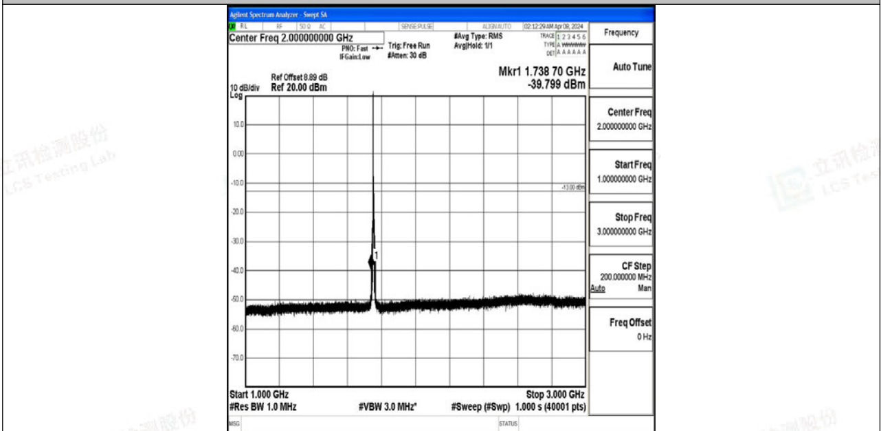
Band4_5MHz_64QAM_20375_1RB#0_1000~3000_1000~3000
