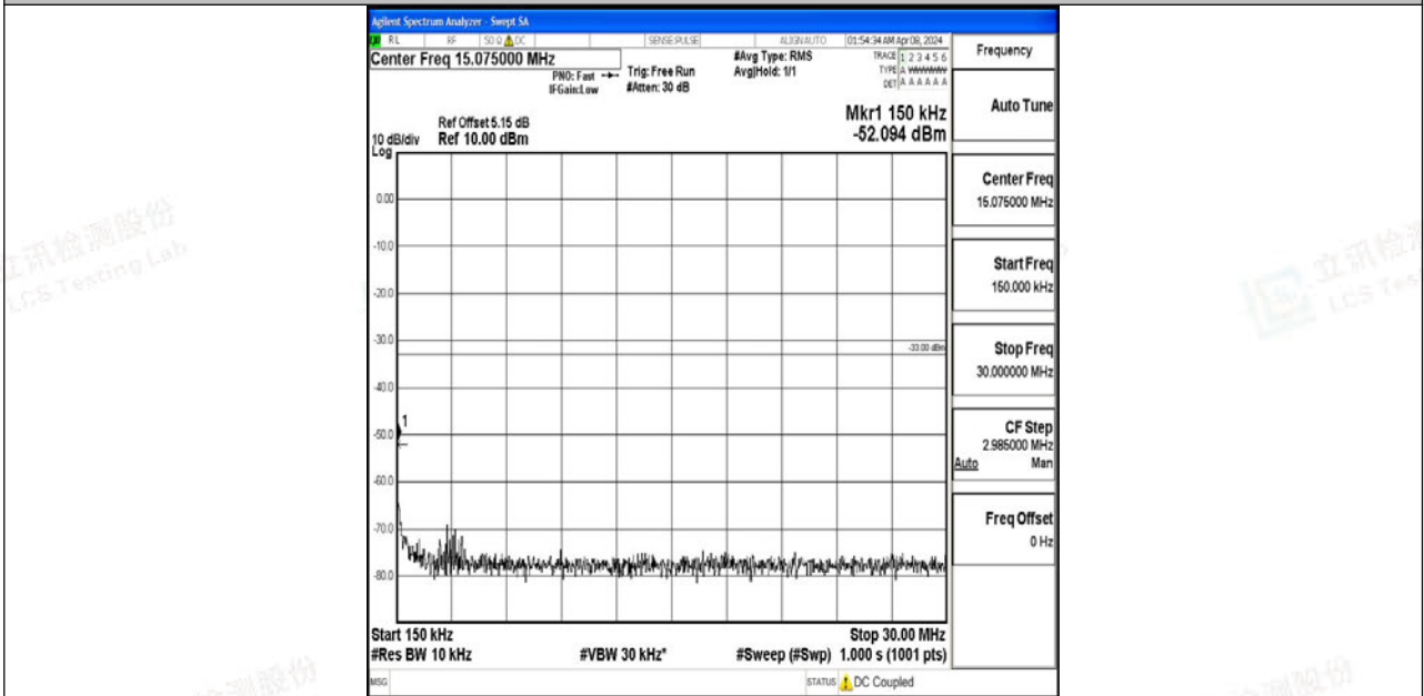
Band4_3MHz_64QAM_20385_1RB#0_0.15~30_0.15~30
