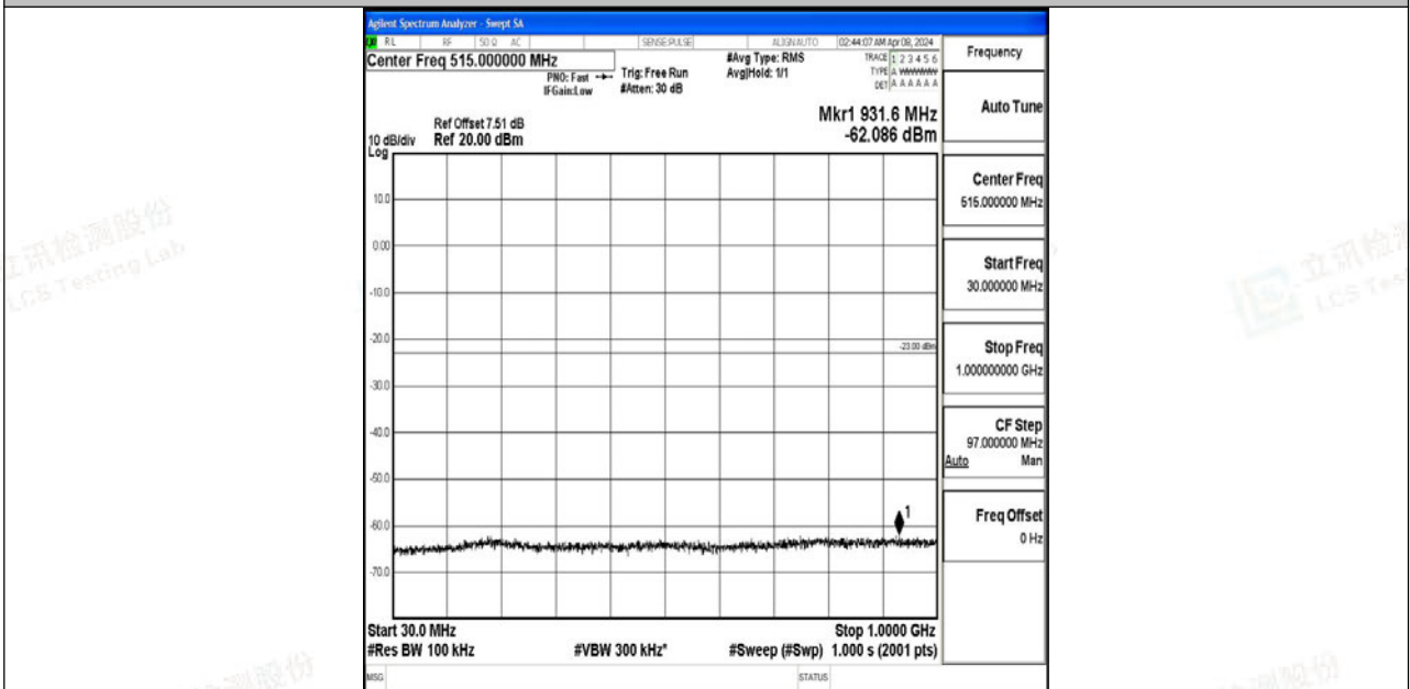
Band4_15MHz_QPSK_20175_1RB#0_30~1000_30~1000
