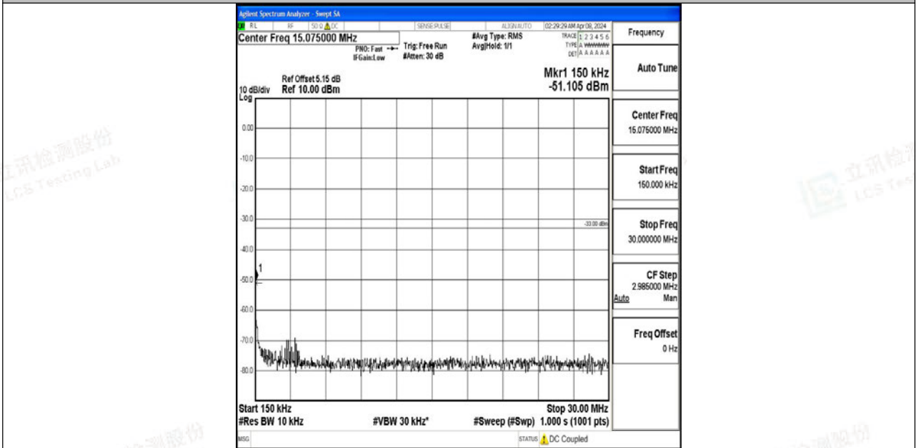
Band4_10MHz_64QAM_20350_1RB#0_0.15~30_0.15~30
