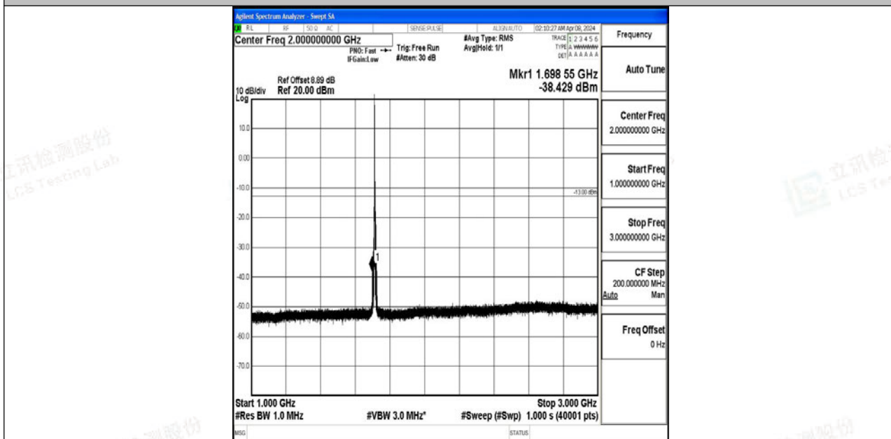
Band4_5MHz_64QAM_19975_1RB#0_1000~3000_1000~3000
