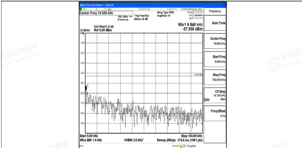
Band4_20MHz_QPSK_20050_1RB#0_0.009~0.15_0.009~0.15
