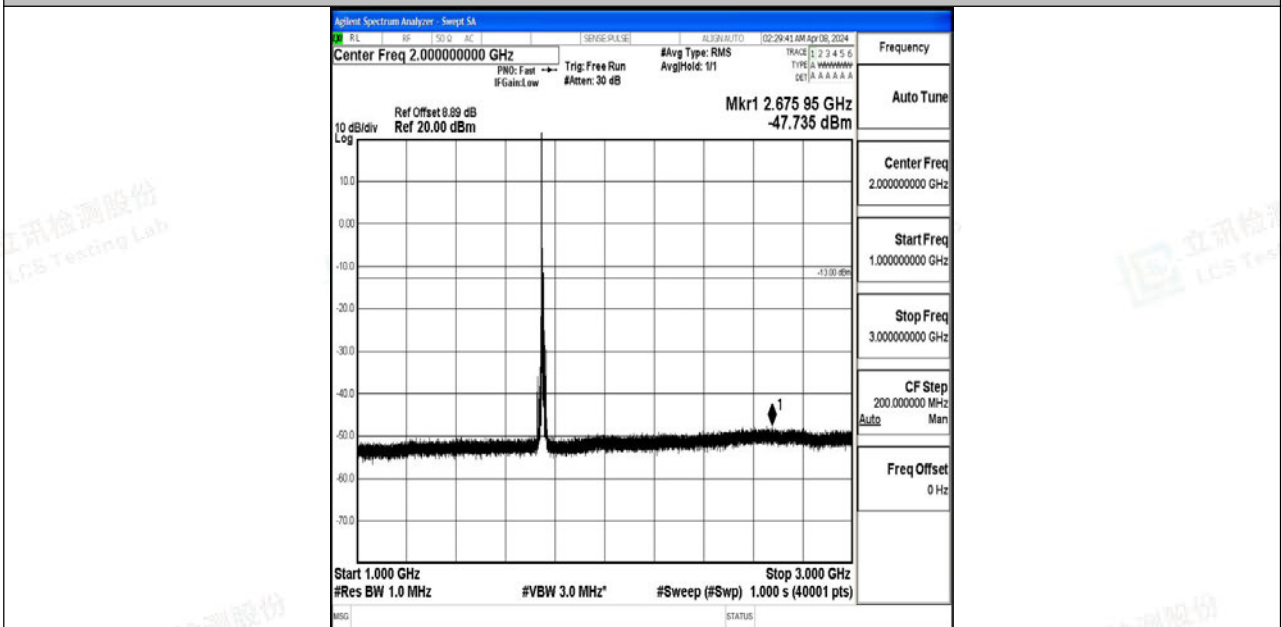
Band4_10MHz_64QAM_20350_1RB#0_1000~3000_1000~3000
