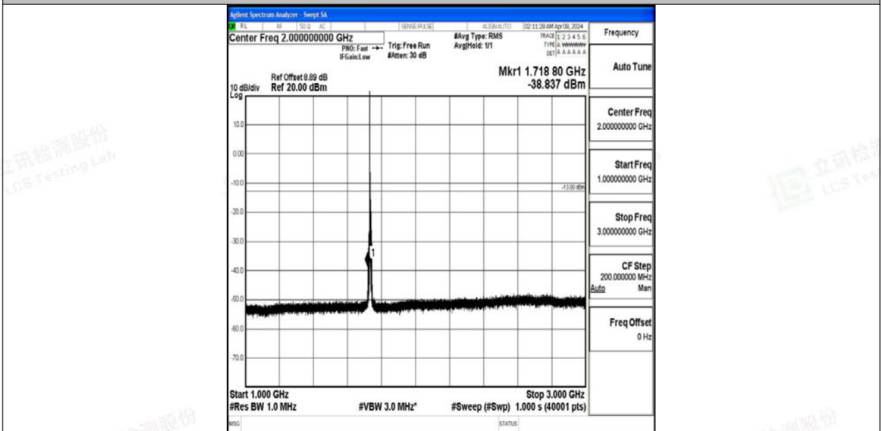
Band4_5MHz_64QAM_20175_1RB#0_1000~3000_1000~3000
