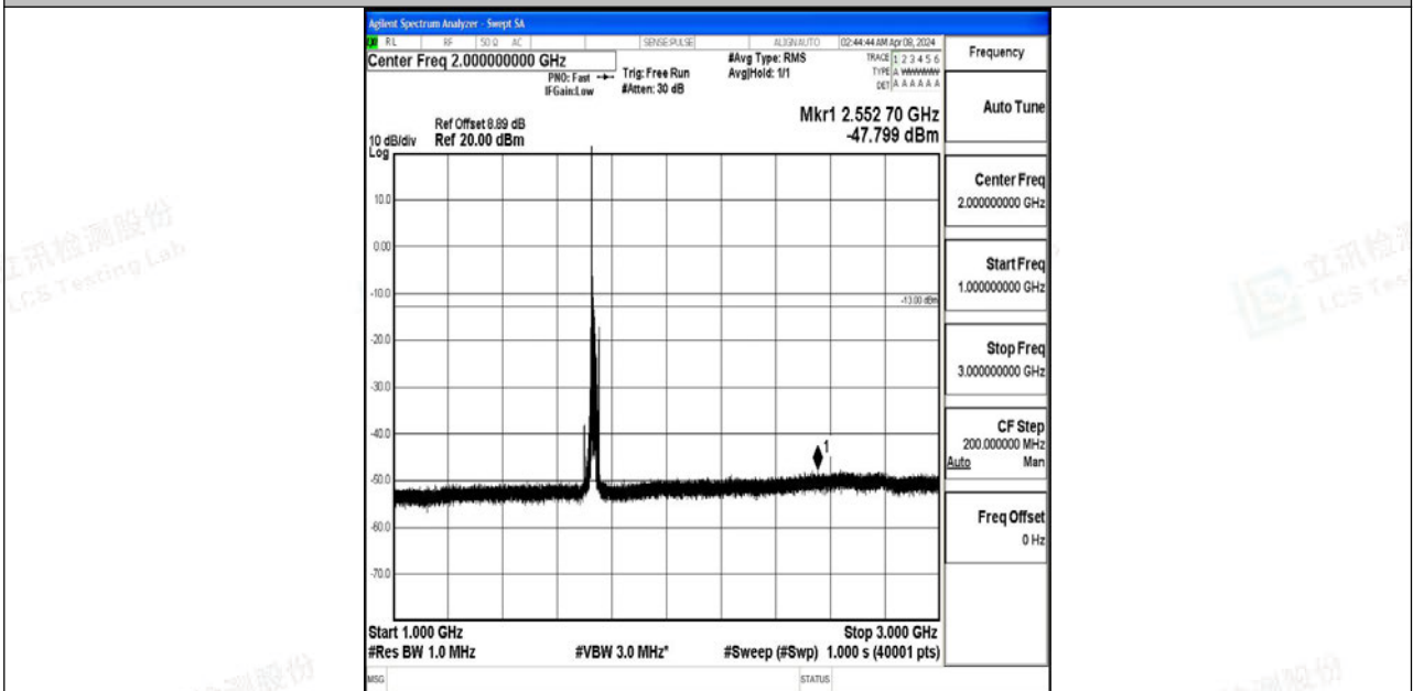
Band4_15MHz_64QAM_20175_1RB#0_1000~3000_1000~3000
