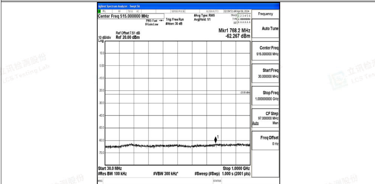
Band4_5MHz_QPSK_19975_1RB#0_30~1000_30~1000
