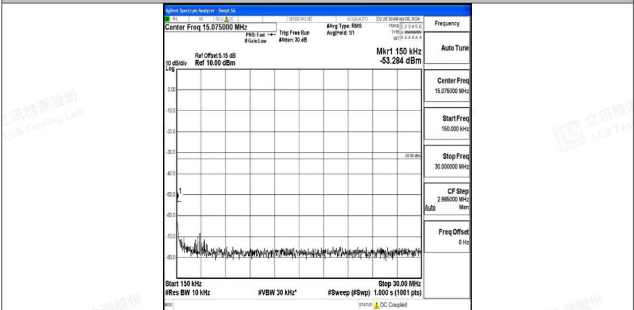
Band4_10MHz_64QAM_20175_1RB#0_0.15~30_0.15~30
