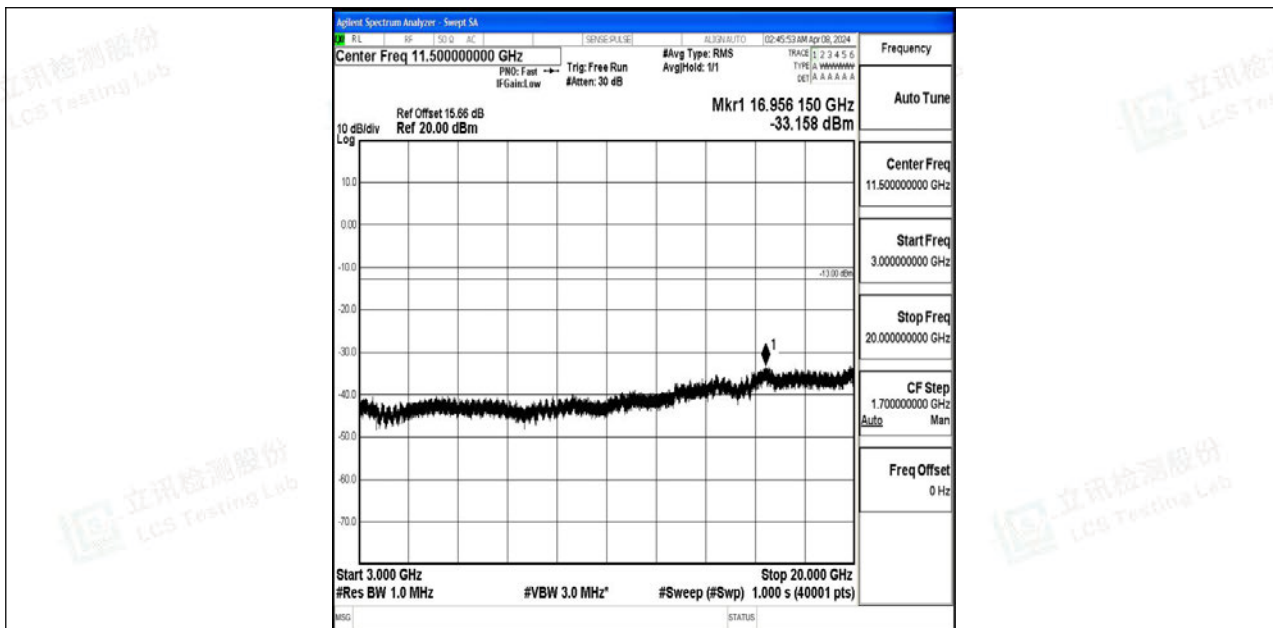
Band4_15MHz_64QAM_20325_1RB#0_3000~20000_3000~20000
