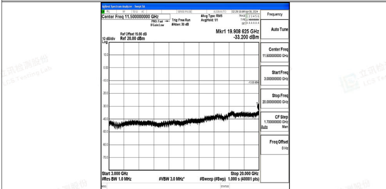
Band4_10MHz_QPSK_20350_1RB#0_3000~20000_3000~20000
