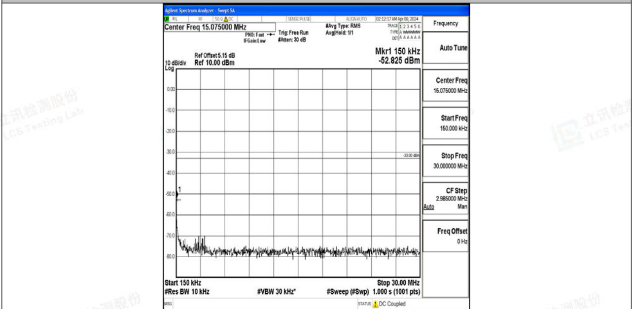
Band4_5MHz_64QAM_20375_1RB#0_0.15~30_0.15~30
