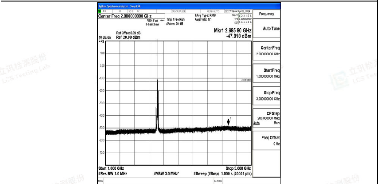
Band4_10MHz_64QAM_20000_1RB#0_1000~3000_1000~3000
