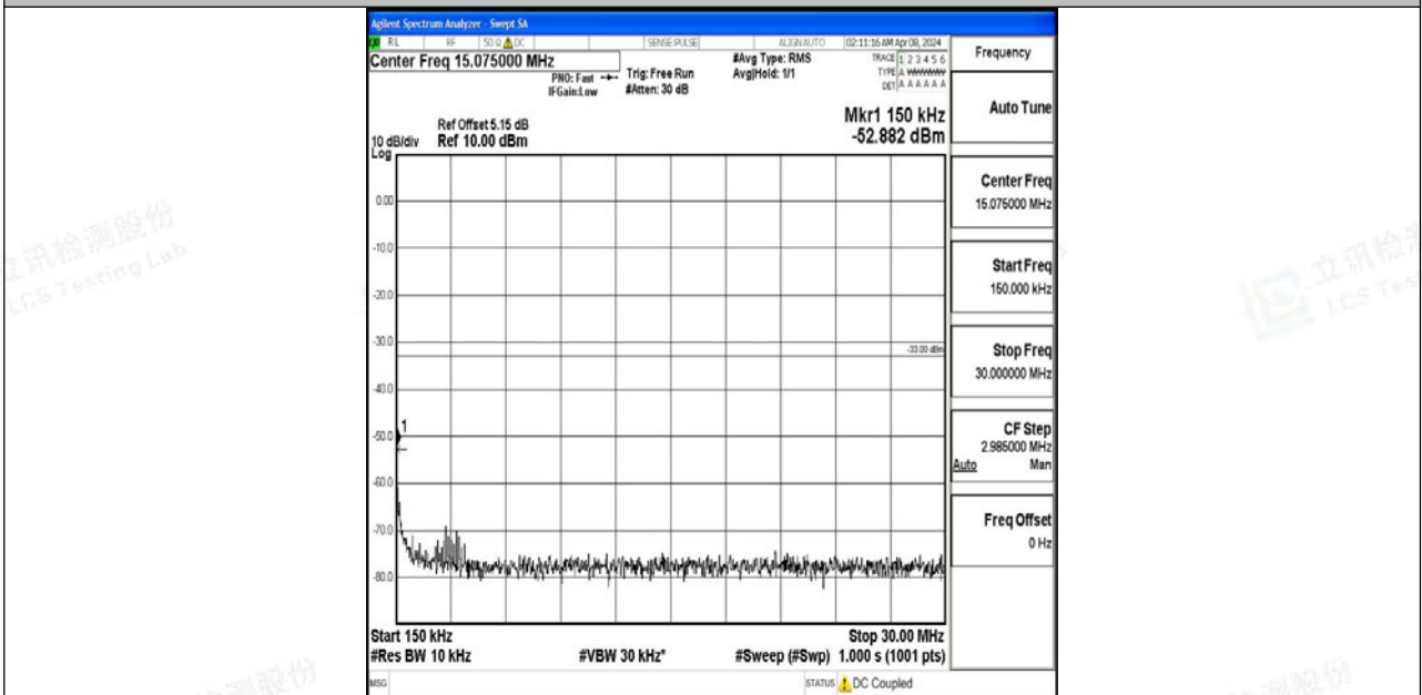
Band4_5MHz_64QAM_20175_1RB#0_0.15~30_0.15~30
