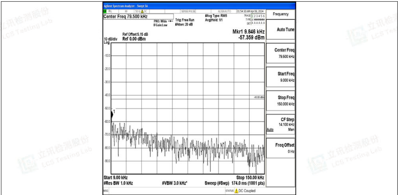
Band4_3MHz_64QAM_20385_1RB#0_0.009~0.15_0.009~0.15
