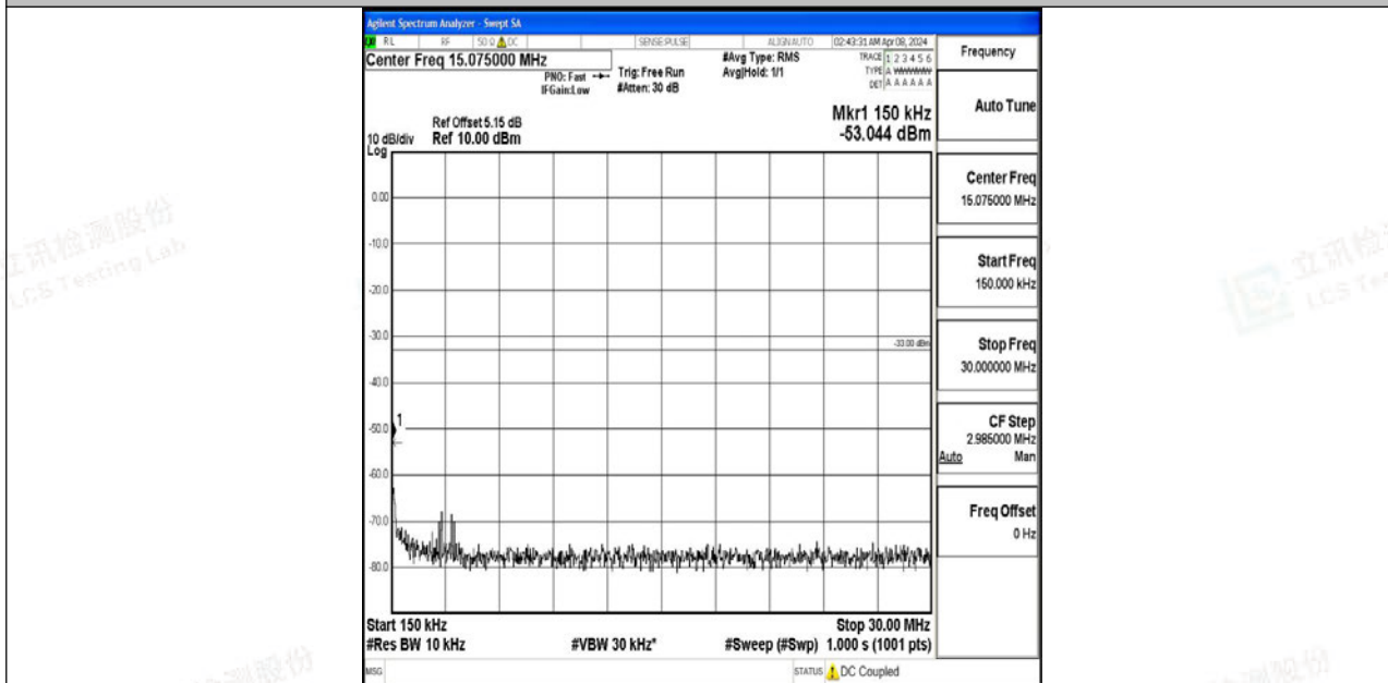
Band4_15MHz_64QAM_2025_1RB#0_0.15~30_0.15~30
