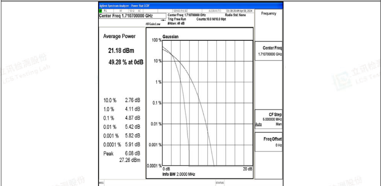
Band4-1.4MHz-64QAM-19957-6RB#0-PASS
