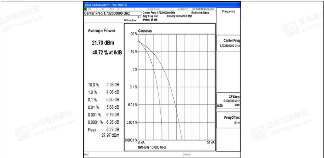
Band4-10MHz-QPSK-20175-50RB#0-PASS
