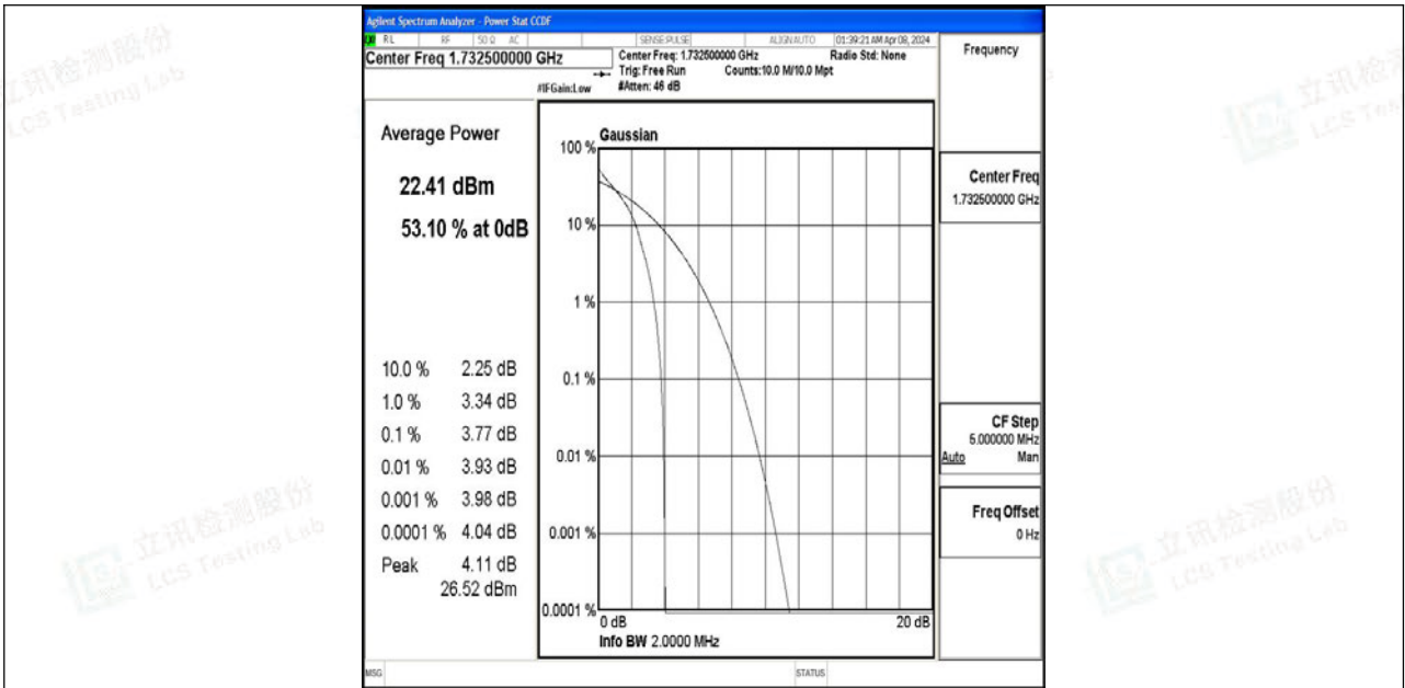
Band4-1.4MHz-QPSK-20175-1RB#0-PASS
