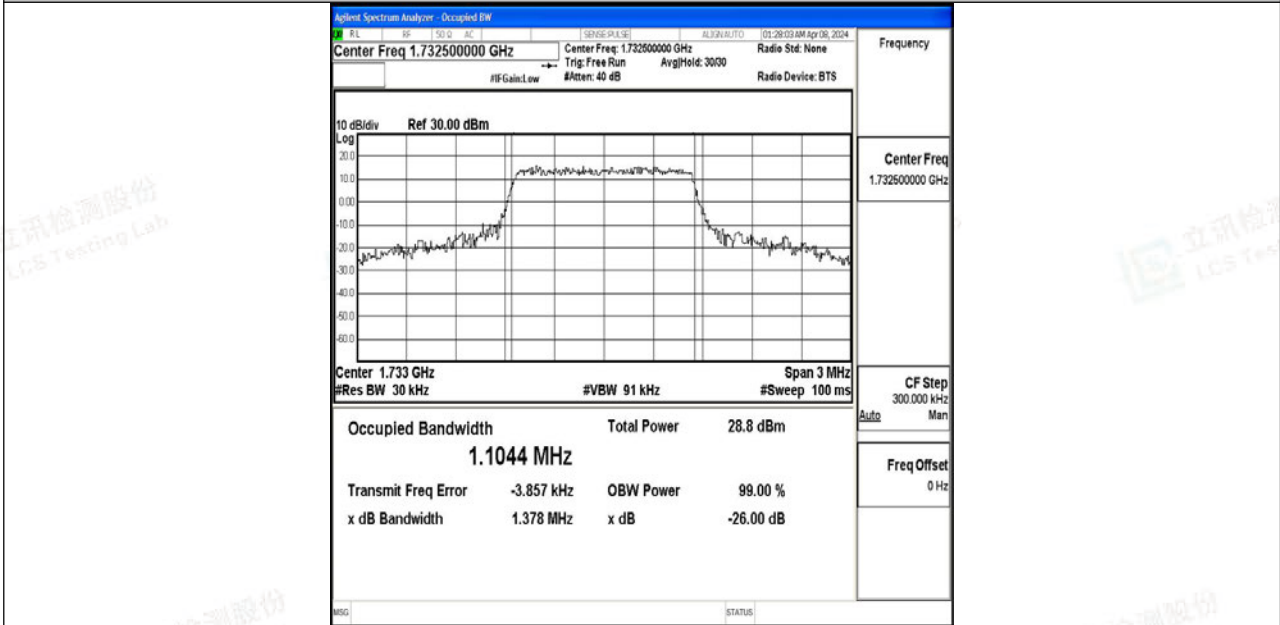
Band4-1.4MHz-64QAM-20175-6RB#0-PASS
