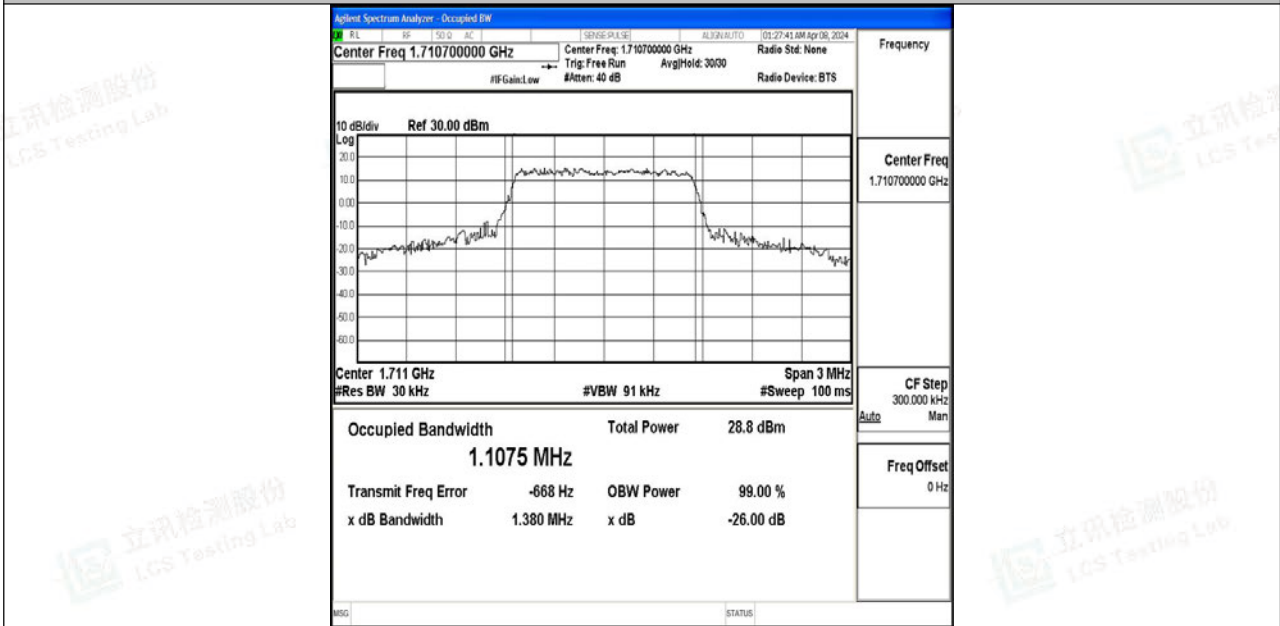
Band4-1.4MHz-64QAM-19957-6RB#0-PASS
