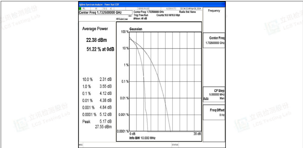
Band4-10MHz-QPSK-20175-1RB#0-PASS
