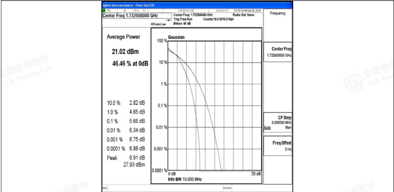
Band4-10MHz-64QAM-20175-50RB#0-PASS
