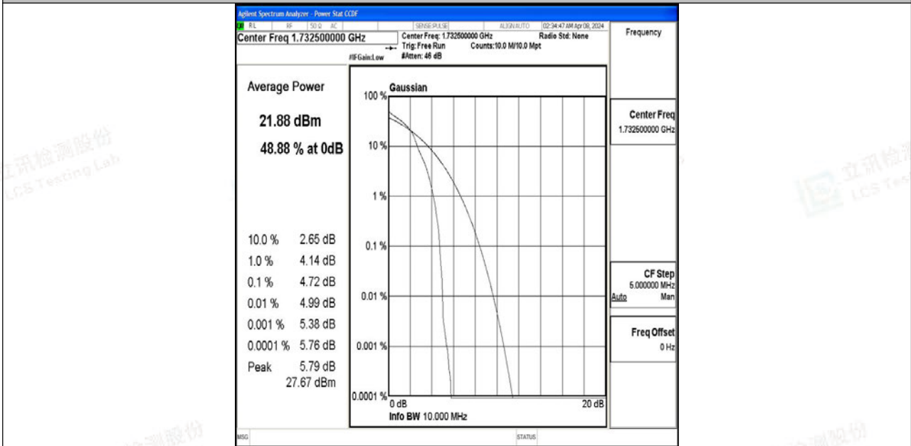
Band4-10MHz-64QAM-20175-1RB#0-PASS
