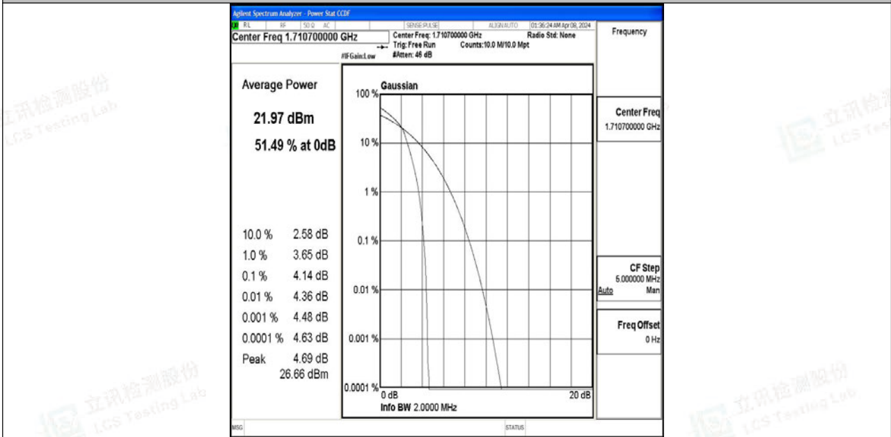
Band4-1.4MHz-64QAM-19957-1RB#0-PASS
