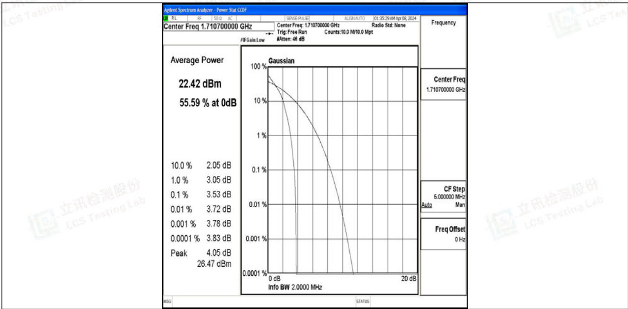
Band4-1.4MHz-QPSK-19957-1RB#0-PASS
