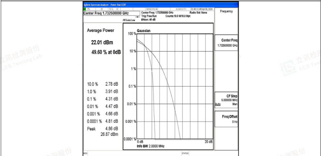
Band4-1.4MHz-64QAM-20175-1RB#0-PASS
