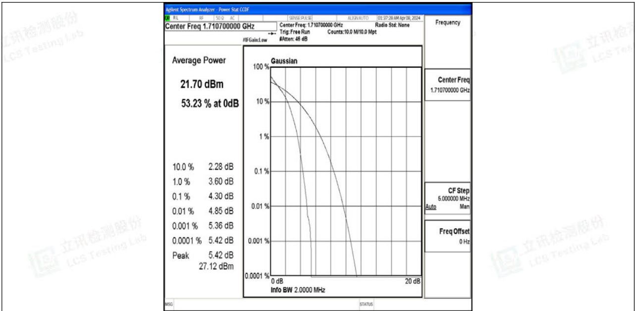
Band4-1.4MHz-QPSK-19957-6RB#0-PASS
