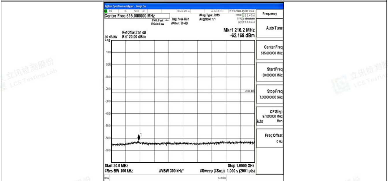
Band2_20MHz_QPSK_18900_1RB#0_30~1000_30~1000
