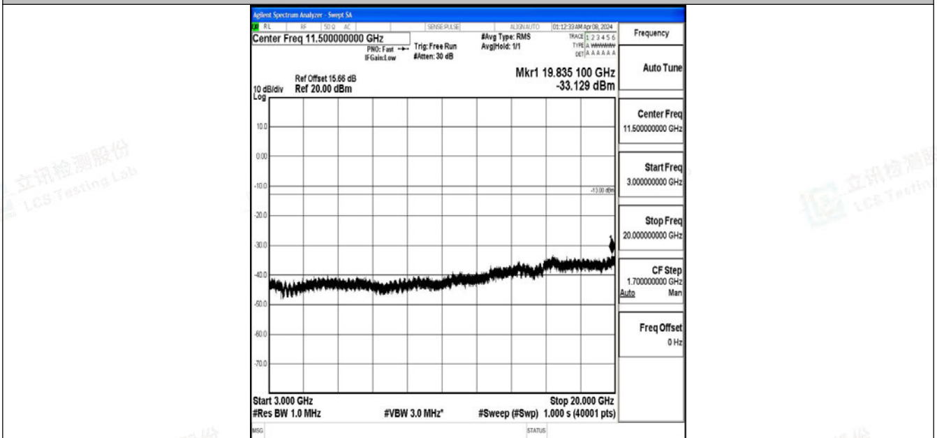
Band2_20MHz_QPSK_18700_1RB#0_3000~20000_3000~20000
