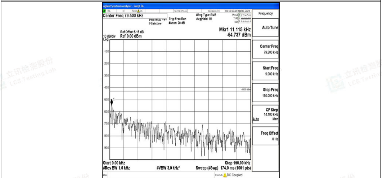
Band2_20MHz_QPSK_18900_1RB#0_0.009~0.15_0.009~0.15
