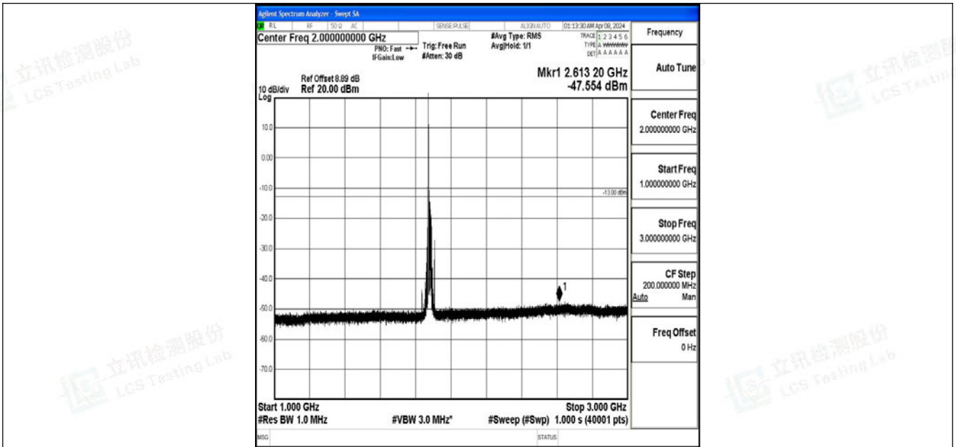
Band2_20MHz_QPSK_18900_1RB#0_1000~3000_1000~3000
