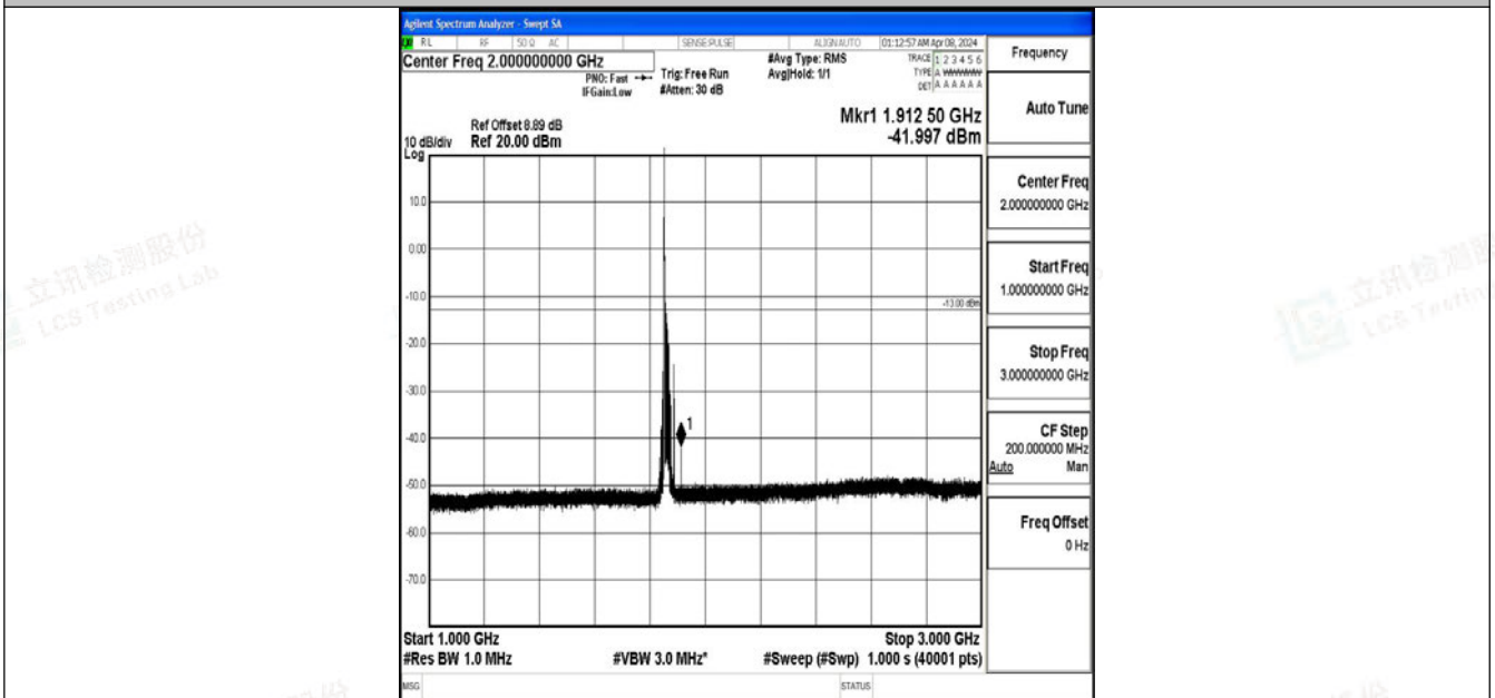
Band2_20MHz_64QAM_18700_1RB#0_1000~3000_1000~3000
