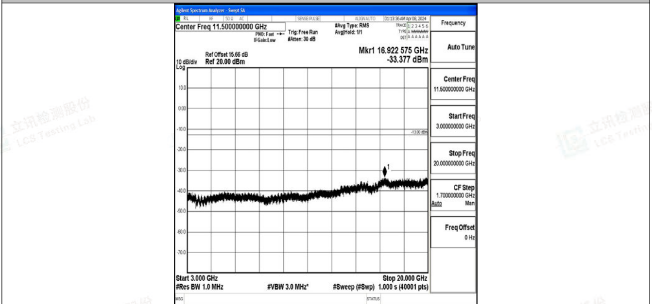
Band2_20MHz_QPSK_18900_1RB#0_3000~20000_3000~20000
