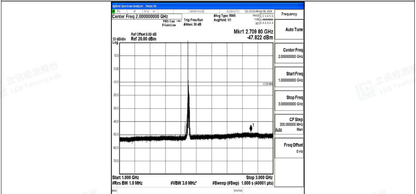
Band2_20MHz_64QAM_19100_1RB#0_1000~3000_1000~3000
