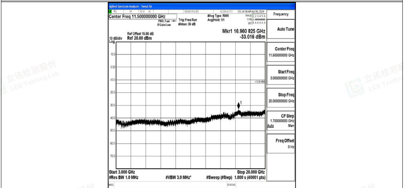
Band2_20MHz_QPSK_19100_1RB#0_3000~20000_3000~20000
