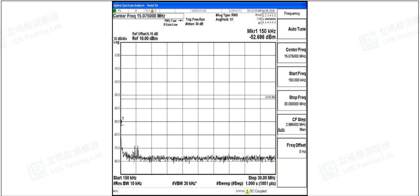
Band2_20MHz_QPSK_18700_1RB#0_0.15~30_0.15~30
