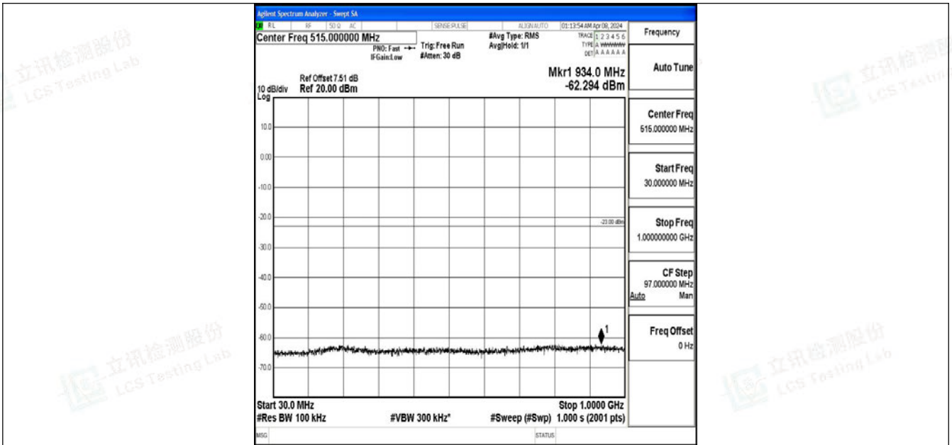
Band2_20MHz_64QAM_18900_1RB#0_30~1000_30~1000
