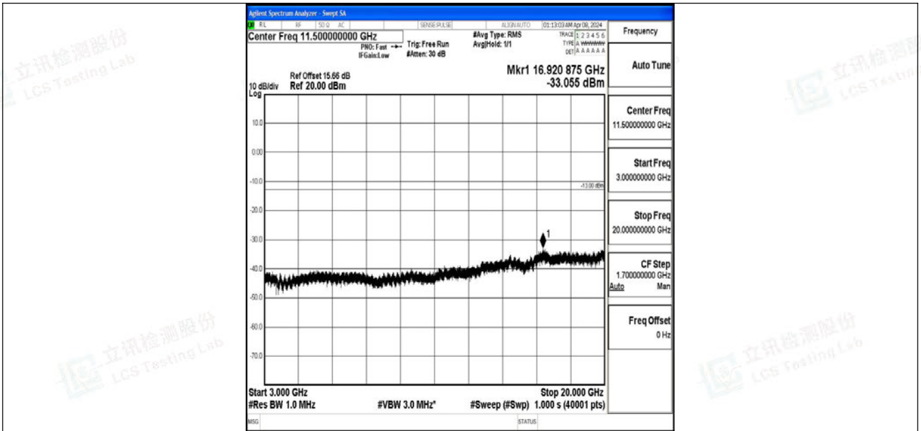
Band2_20MHz_64QAM_18700_1RB#0_3000~20000_3000~20000
