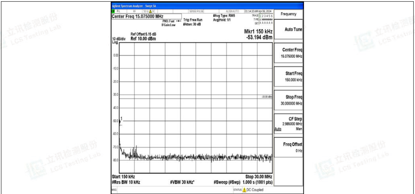
Band2_20MHz_QPSK_19100_1RB#0_0.15~30_0.15~30
