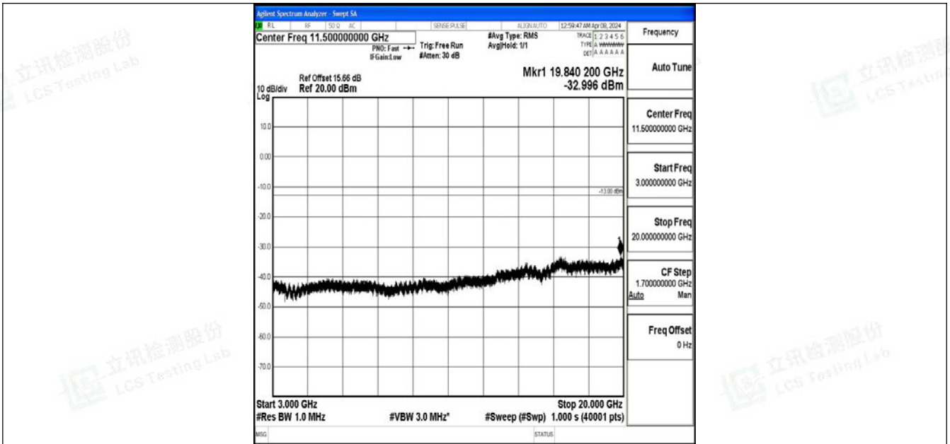
Band2_15MHz_64QAM_19125_1RB#0_3000~20000_3000~20000
