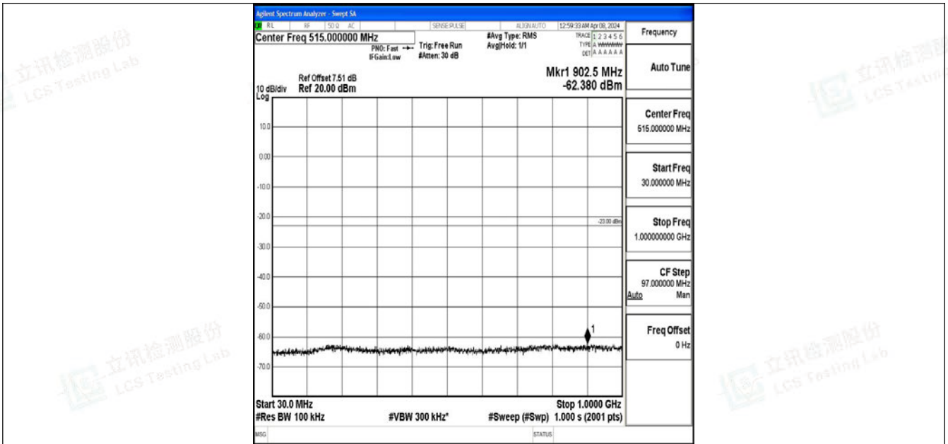
Band2_15MHz_64QAM_19125_1RB#0_30~1000_30~1000
