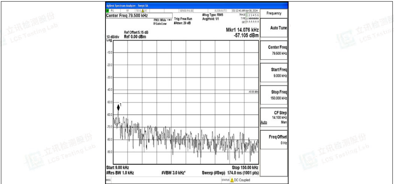
Band2_20MHz_64QAM_18700_1RB#0_0.009~0.15_0.009~0.15
