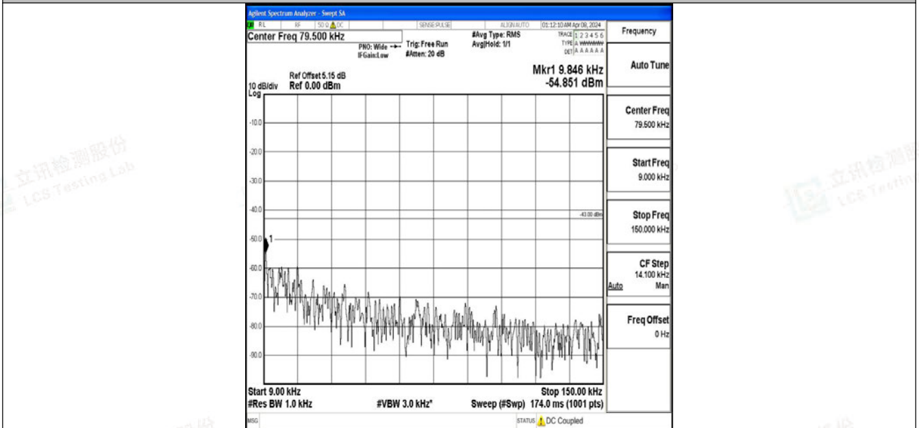
Band2_20MHz_QPSK_18700_1RB#0_0.009~0.15_0.009~0.15
