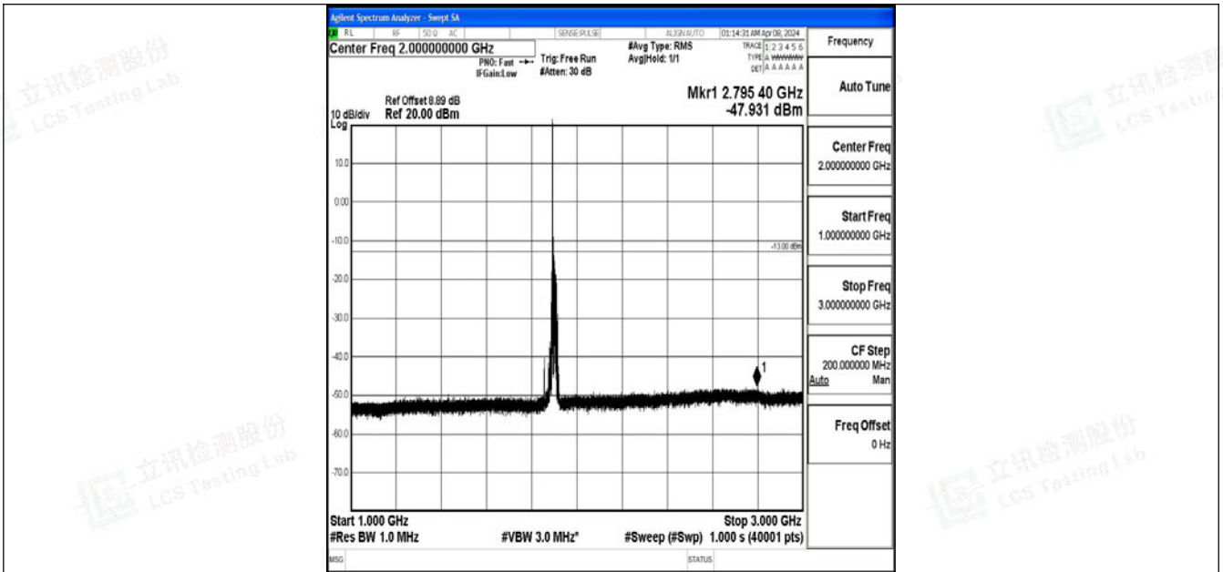
Band2_20MHz_QPSK_19100_1RB#0_1000~3000_1000~3000
