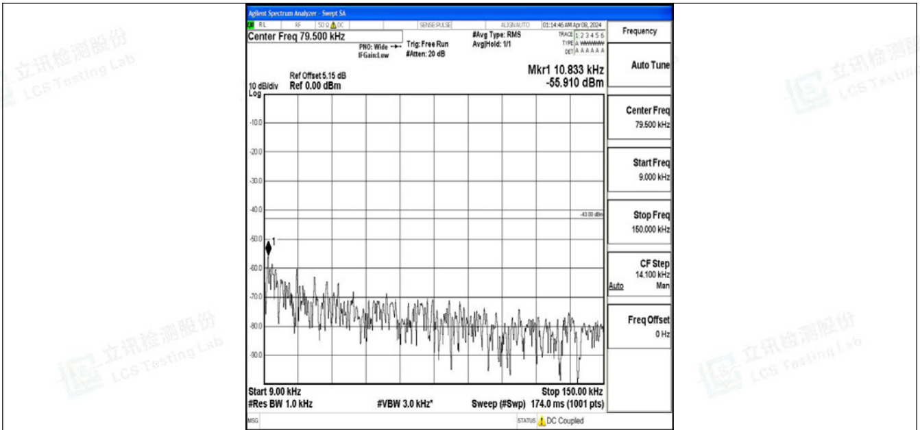
Band2_20MHz_64QAM_19100_1RB#0_0.009~0.15_0.009~0.15
