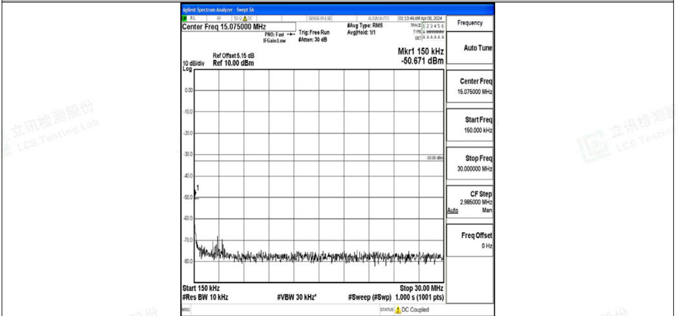
Band2_20MHz_64QAM_18900_1RB#0_0.15~30_0.15~30
