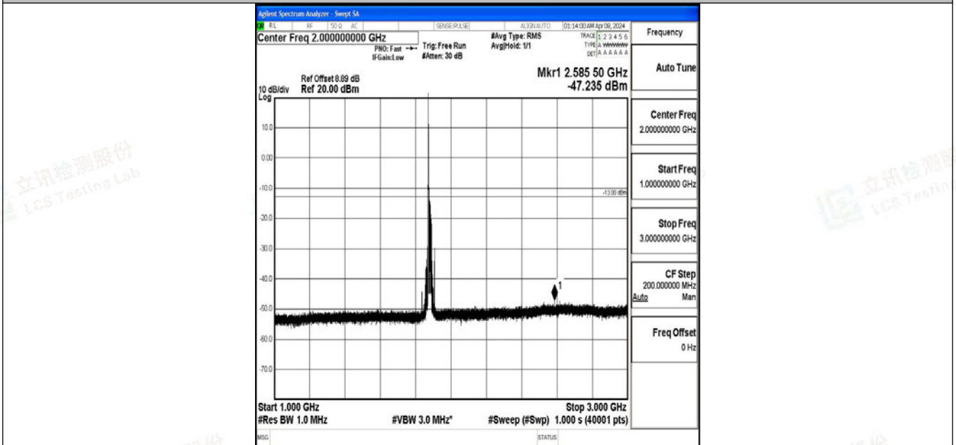
Band2_20MHz_64QAM_18900_1RB#0_1000~3000_1000~3000
