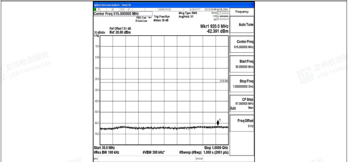
Band2_20MHz_QPSK_18700_1RB#0_30~1000_30~1000
