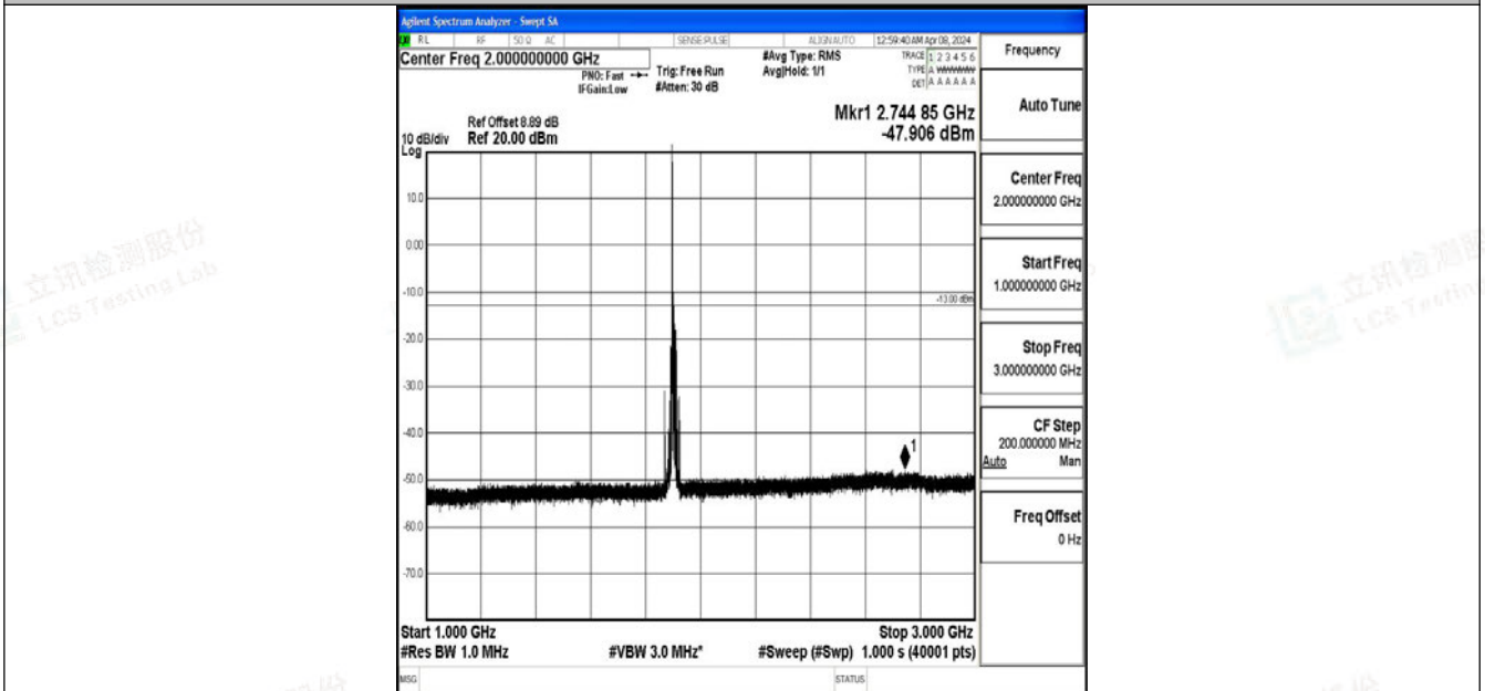
Band2_15MHz_64QAM_19125_1RB#0_1000~3000_1000~3000
