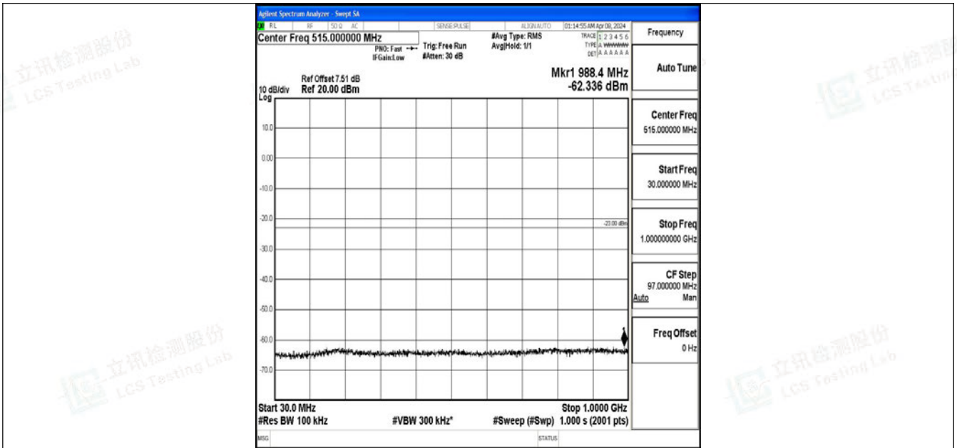
Band2_20MHz_64QAM_19100_1RB#0_30~1000_30~1000
