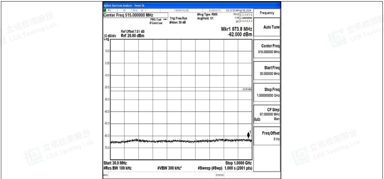
Band2_20MHz_64QAM_18700_1RB#0_30~1000_30~1000
