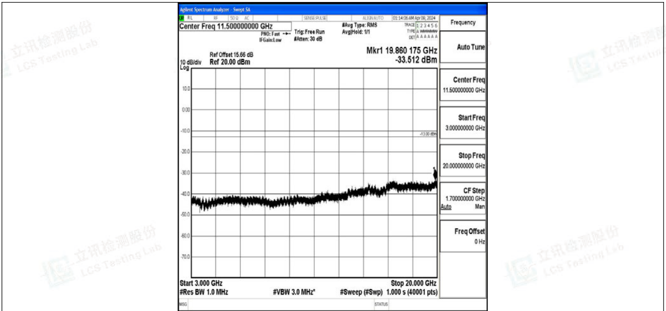
Band2_20MHz_64QAM_18900_1RB#0_3000~20000_3000~20000
