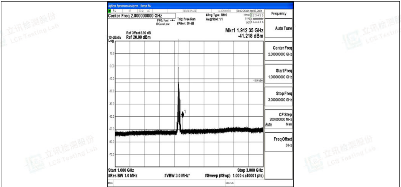
Band2_20MHz_QPSK_18700_1RB#0_1000~3000_1000~3000
