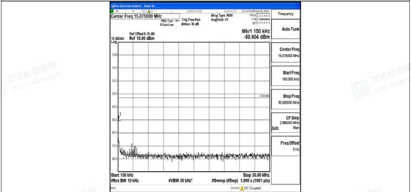
Band2_20MHz_64QAM_19100_1RB#0_0.15~30_0.15~30
