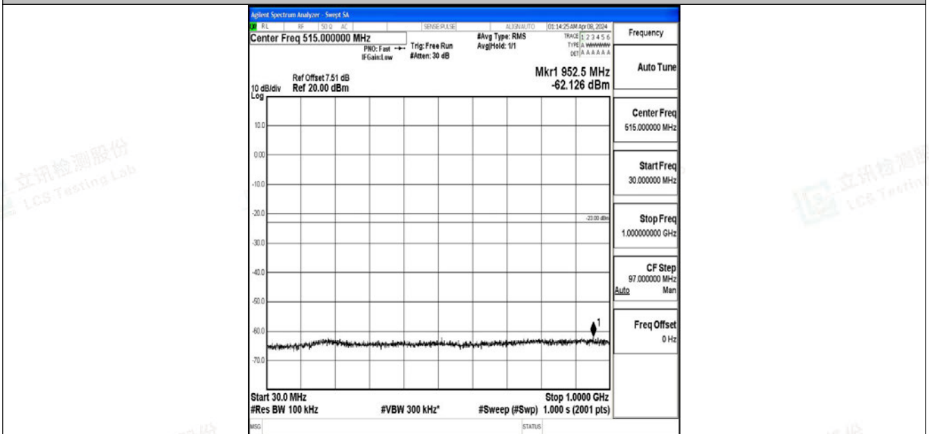
Band2_20MHz_QPSK_19100_1RB#0_30~1000_30~1000
