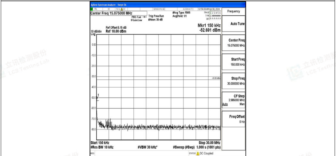
Band2_15MHz_64QAM_19125_1RB#0_0.15~30_0.15~30
