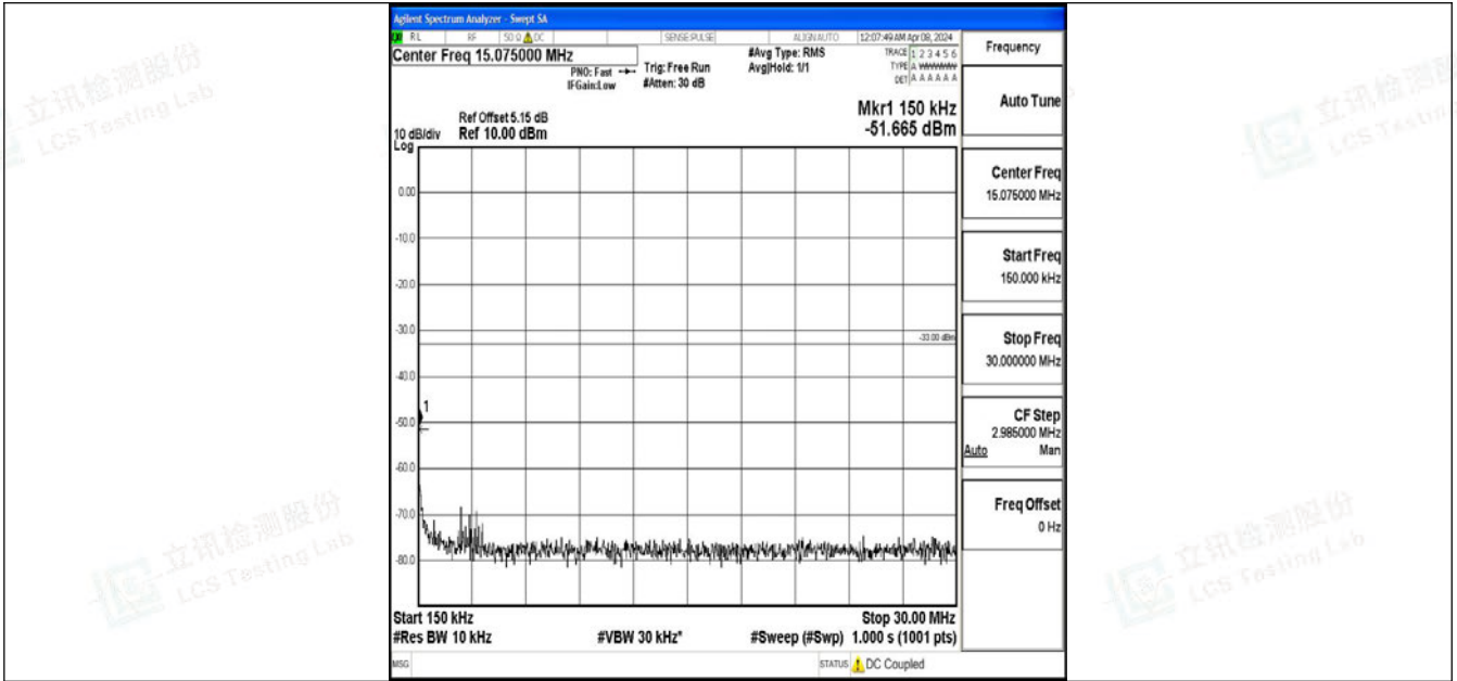
Band2_3MHz_QPSK_19185_1RB#0_0.15~30_0.15~30
