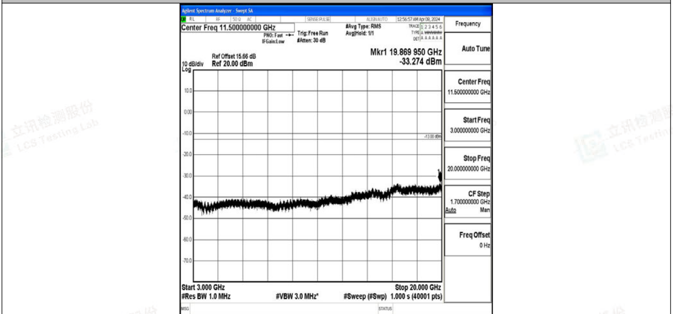
Band2_15MHz_QPSK_18675_1RB#0_3000~20000_3000~20000
