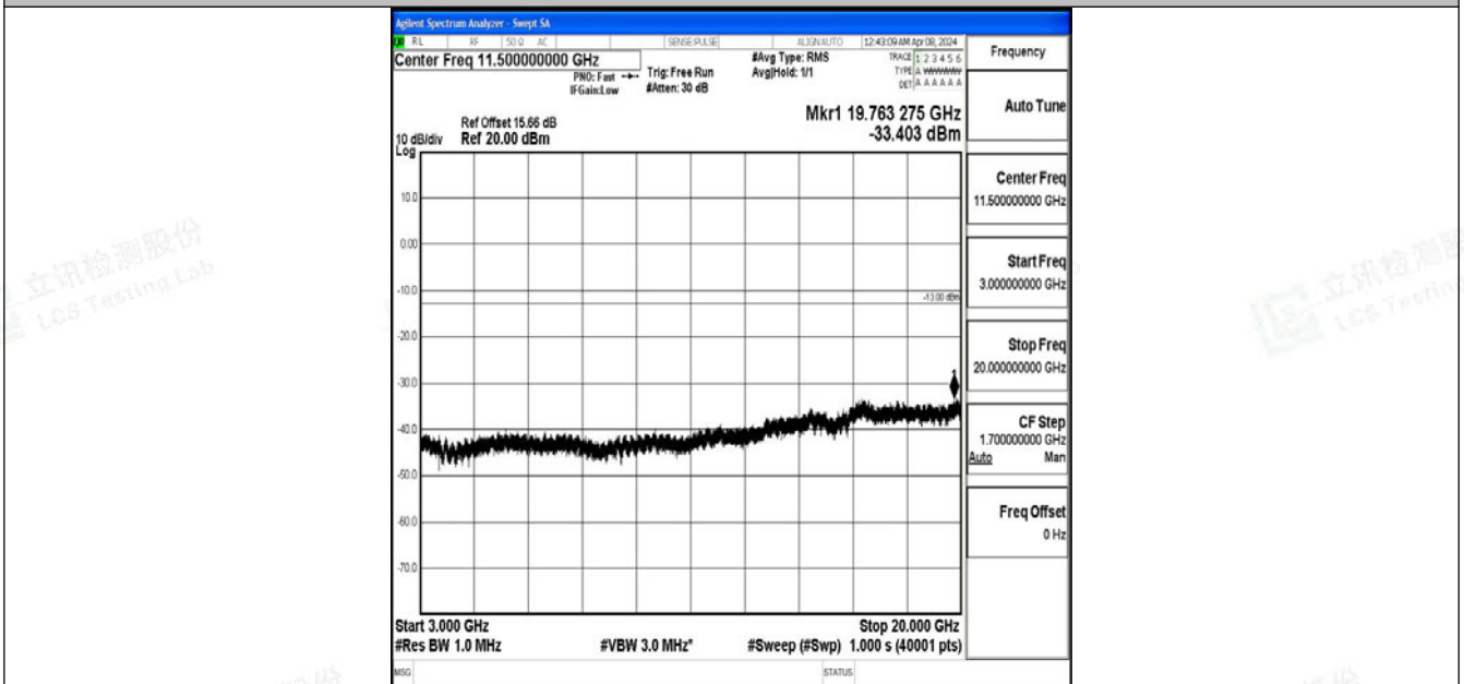
Band2_10MHz_QPSK_19150_1RB#0_3000~20000_3000~20000
