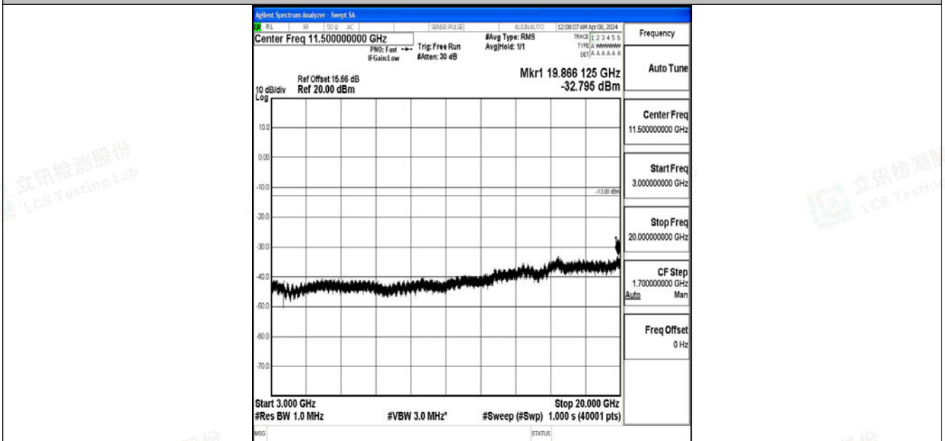
Band2_3MHz_QPSK_19185_1RB#0_3000~20000_3000~20000
