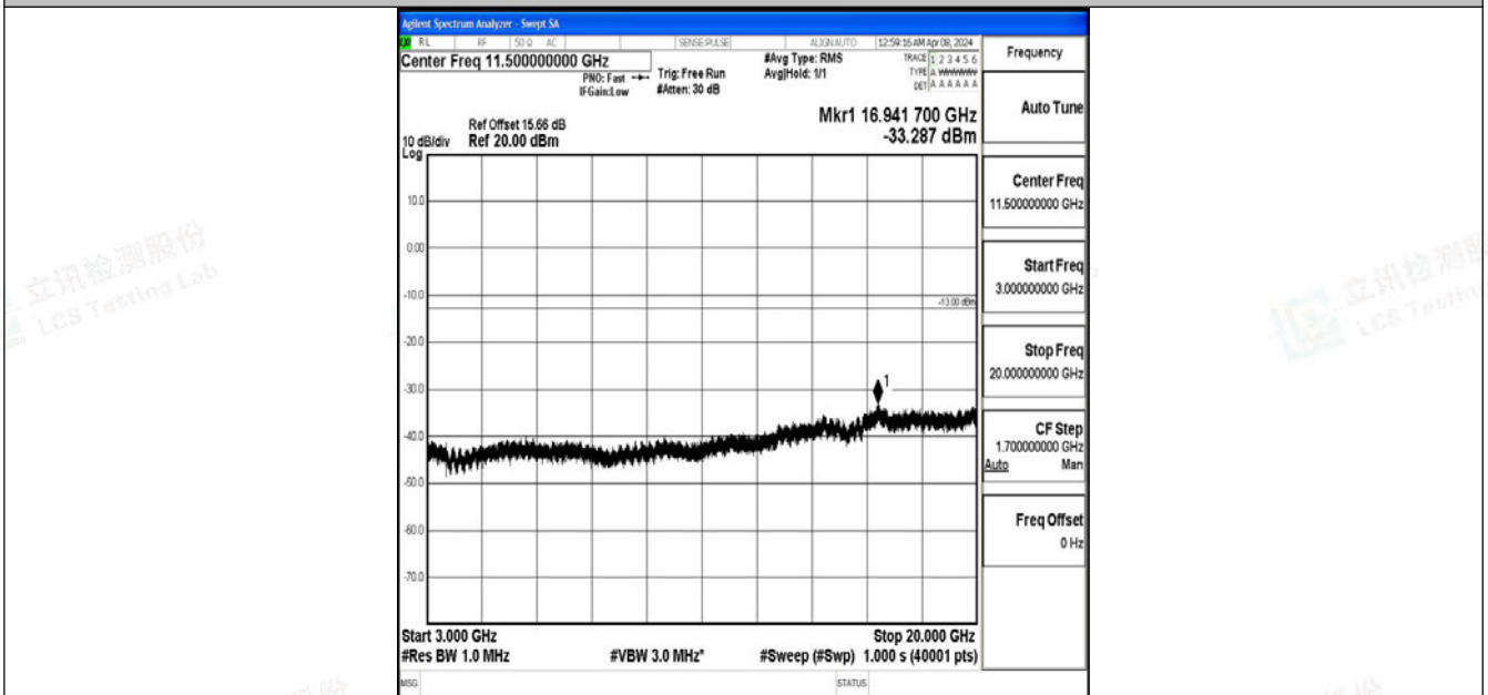
Band2_15MHz_QPSK_19125_1RB#0_3000~20000_3000~20000
