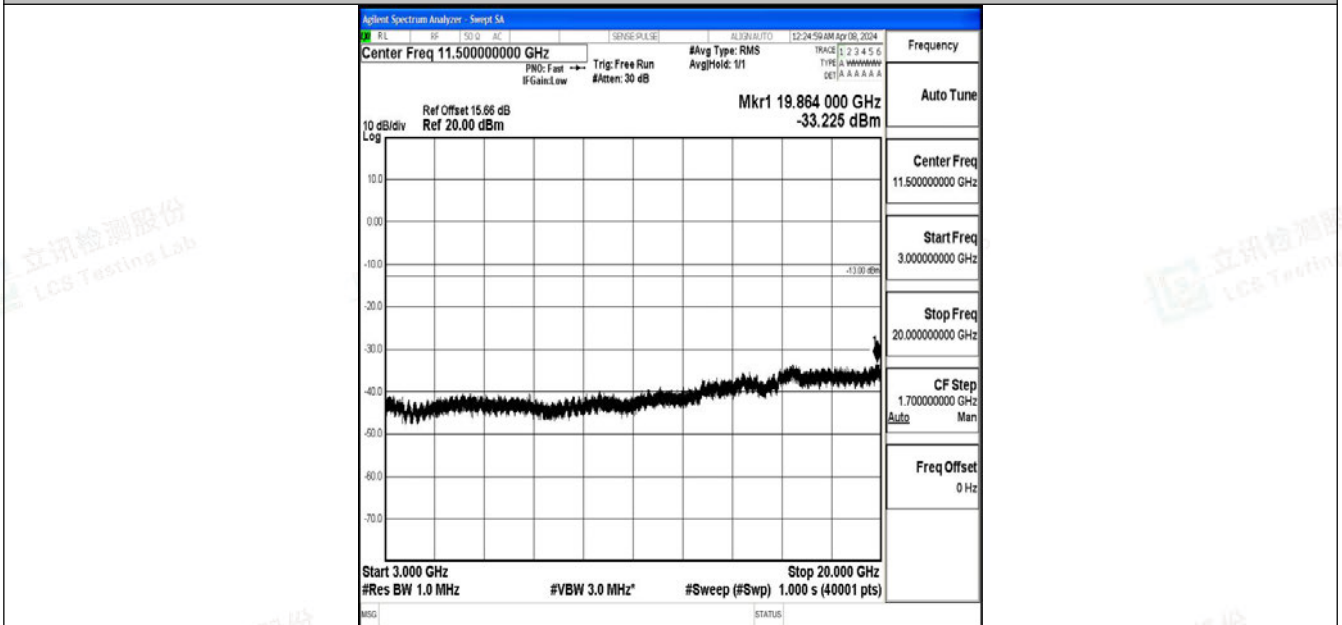
Band2_5MHz_QPSK_18900_1RB#0_3000~20000_3000~20000
