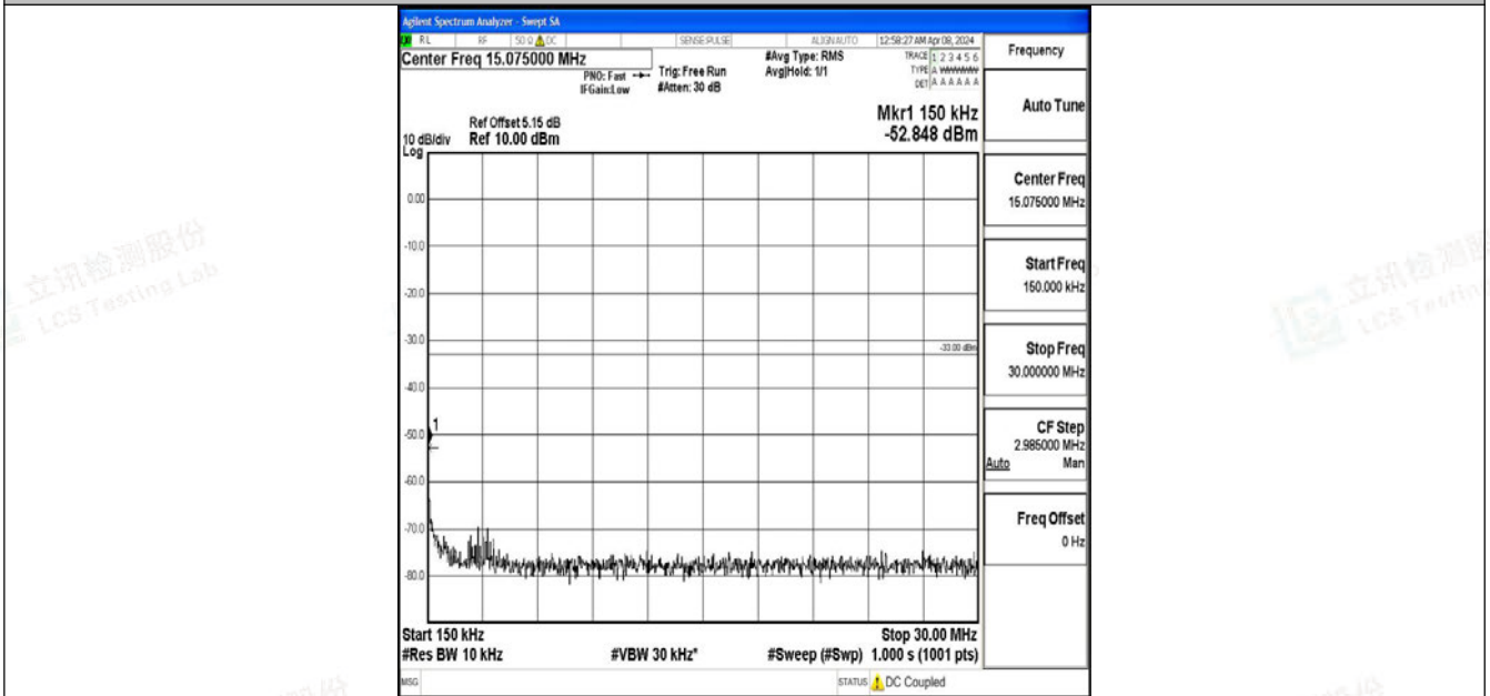
Band2_15MHz_64QAM_18900_1RB#0_0.15~30_0.15~30
