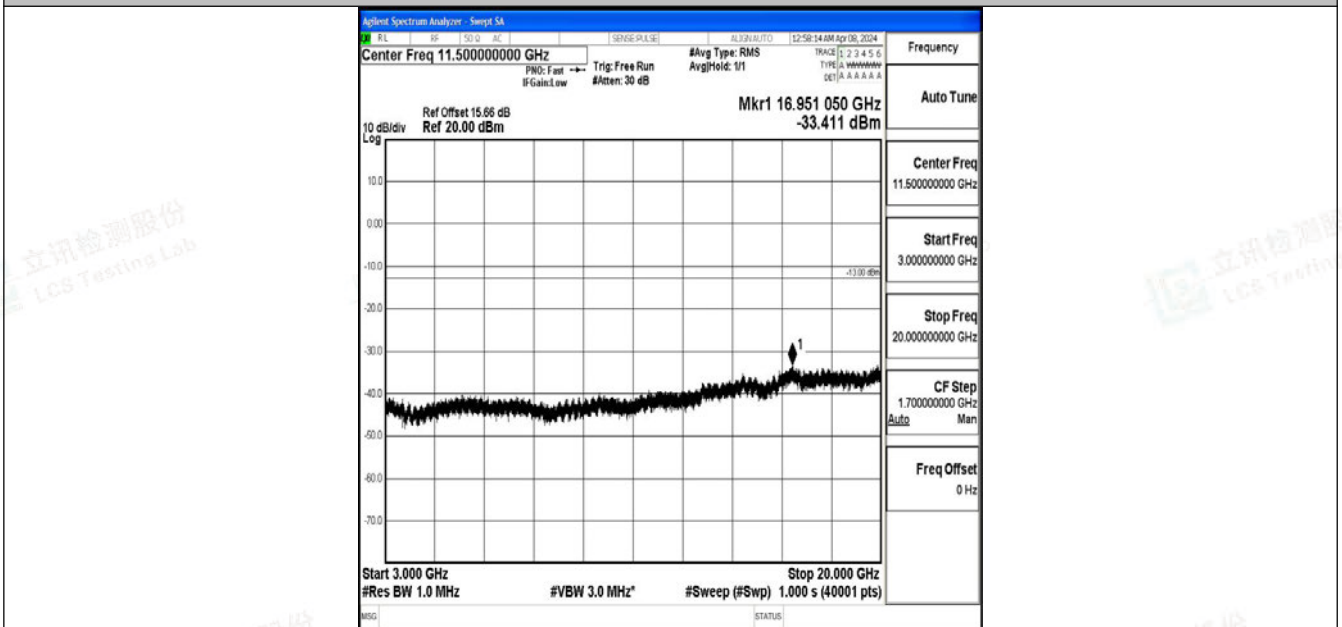
Band2_15MHz_QPSK_18900_1RB#0_3000~20000_3000~20000
