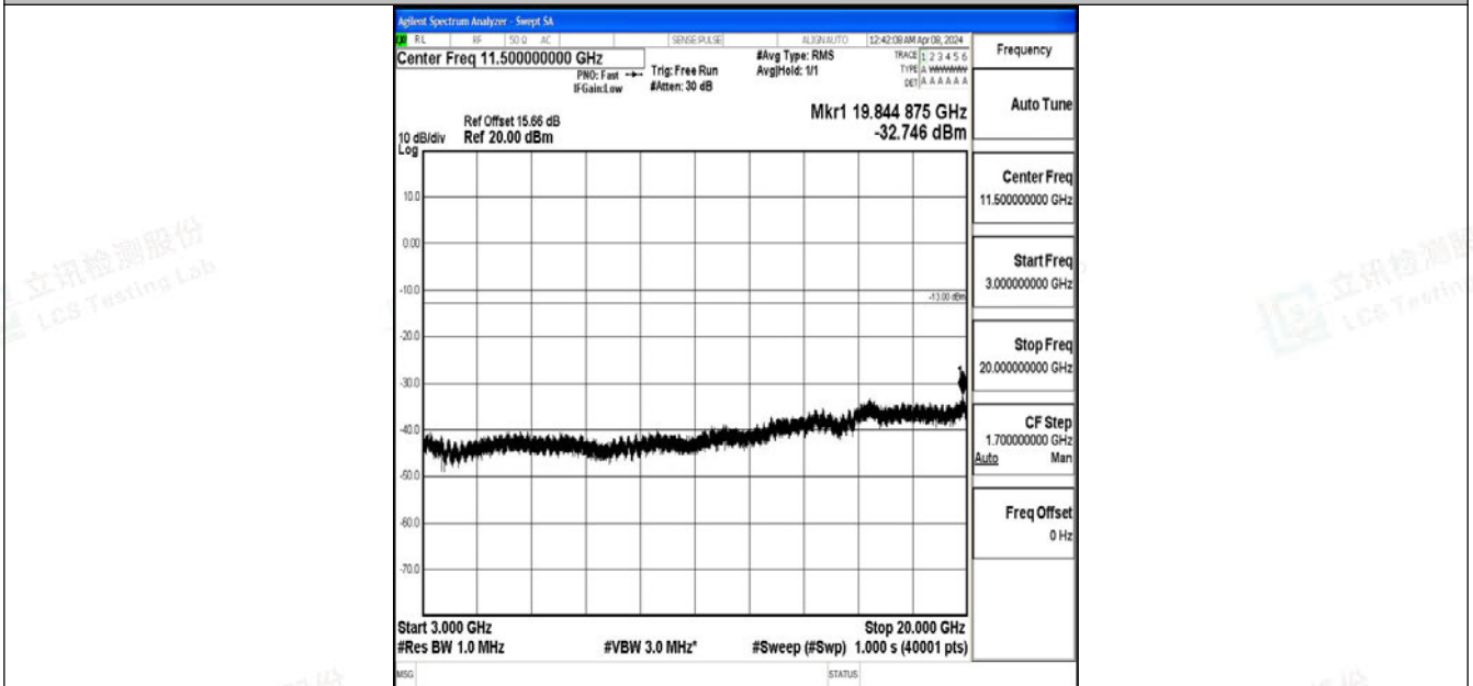
Band2_10MHz_QPSK_18900_1RB#0_3000~20000_3000~20000
