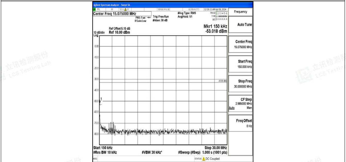
Band2_5MHz_64QAM_19175_1RB#0_0.15~30_0.15~30
