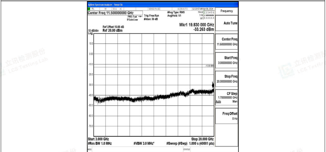
Band2_5MHz_QPSK_18625_1RB#0_3000~20000_3000~20000
