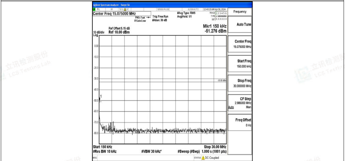
Band2_10MHz_64QAM_19150_1RB#0_0.15~30_0.15~30
