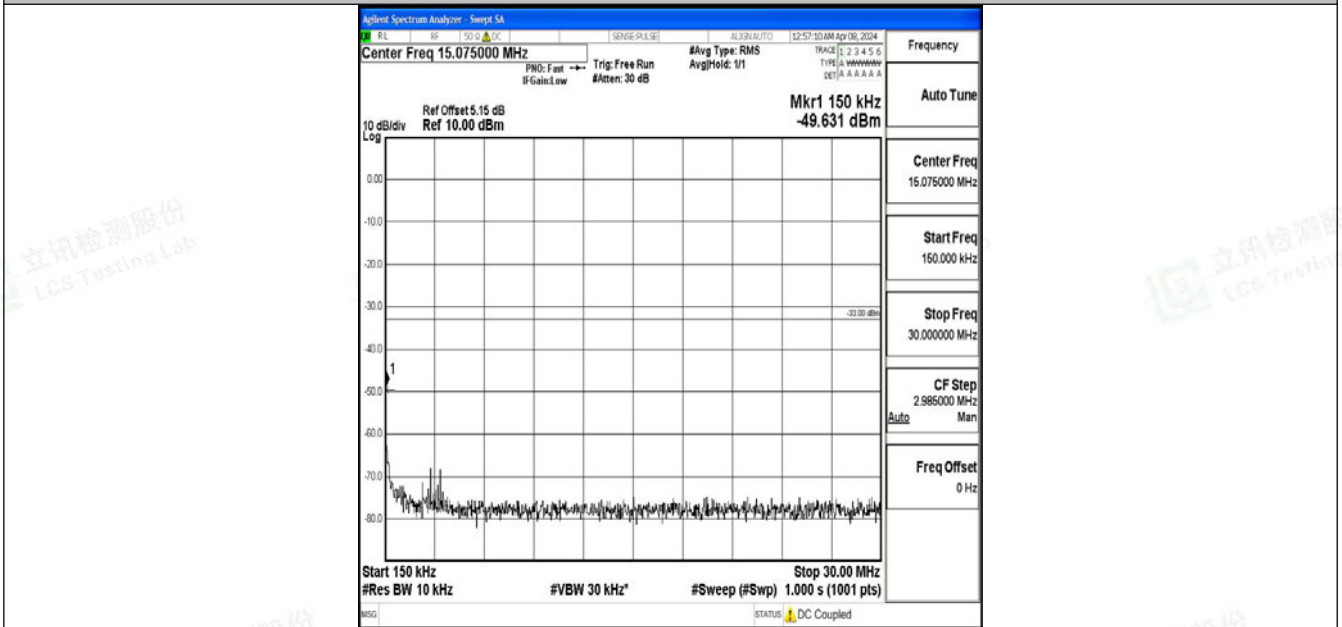
Band2_15MHz_64QAM_18675_1RB#0_0.15~30_0.15~30
