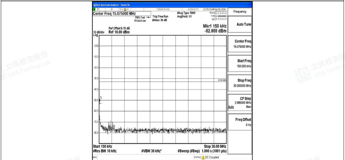
Band2_5MHz_64QAM_18900_1RB#0_0.15~30_0.15~30
