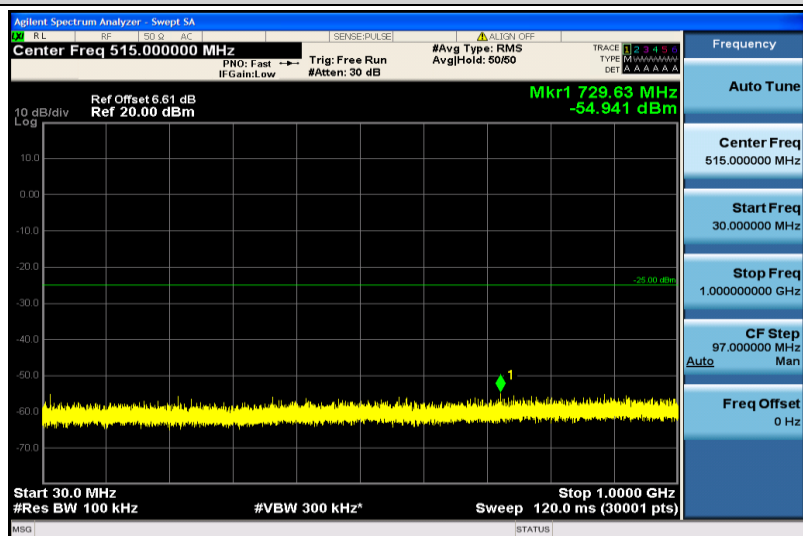
Band41-5MHz-16QAM-40740-1RB#0-30~1000MHz
