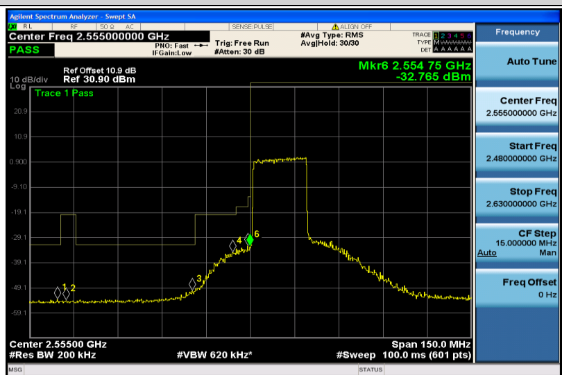
Band41-20MHz-16QAM-40340-100RB#0
