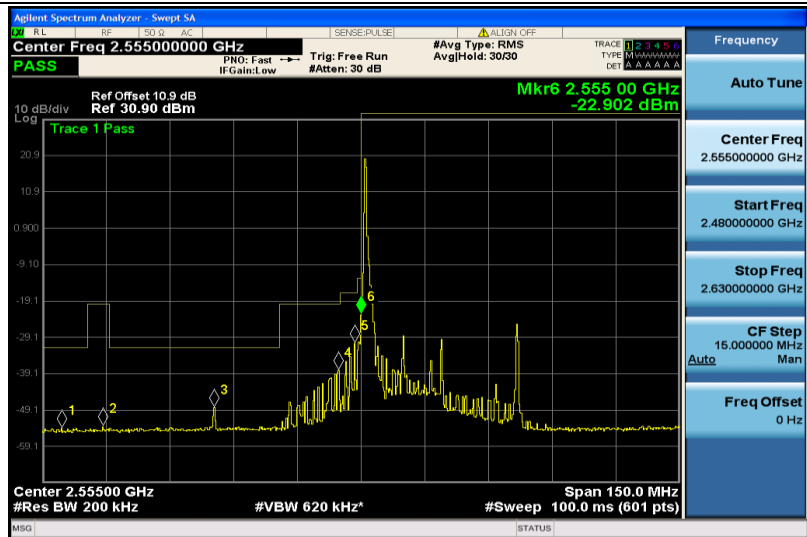
Band41-20MHz-QPSK-40340-1RB#0
