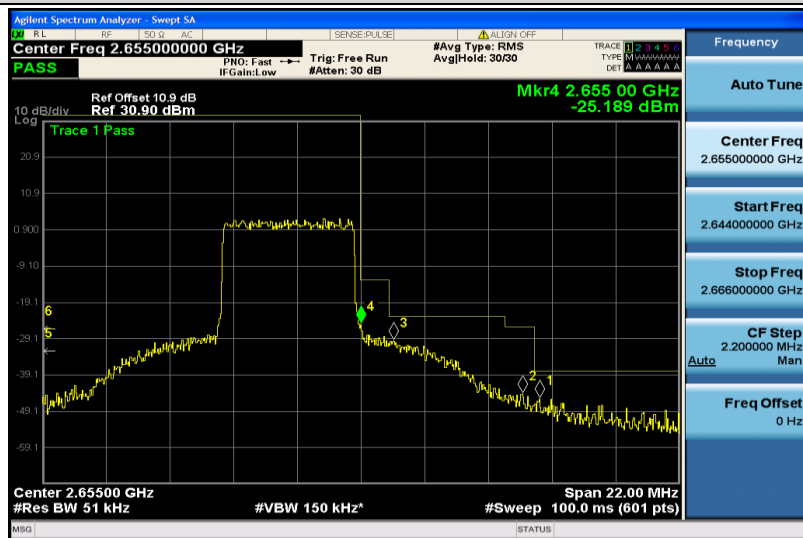
Band41-5MHz-16QAM-41215-25RB#0
