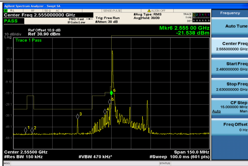
Band41-15MHz-QPSK-40315-1RB#0
