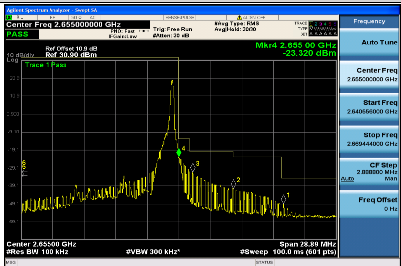
Band41-10MHz-16QAM-41190-1RB#49
