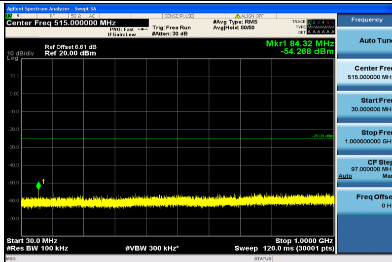
Band41-10MHz-QPSK-41190-1RB#0-30~1000MHz
