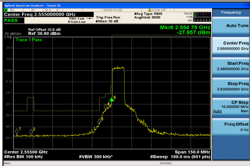
Band41-10MHz-QPSK-40290-50RB#0
