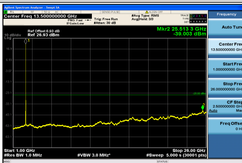
Band41-10MHz-16QAM-41190-1RB#0-1000~26000MHz
