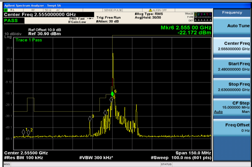
Band41-10MHz-16QAM-40290-1RB#0
