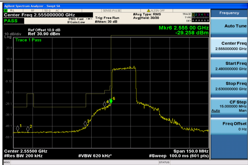
Band41-20MHz-QPSK-40340-100RB#0
