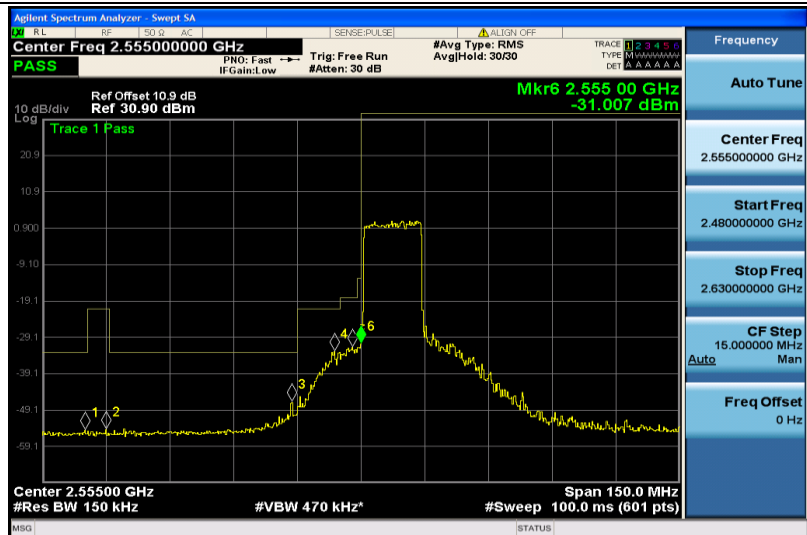
Band41-15MHz-16QAM-40315-75RB#0
