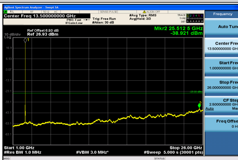
Band41-15MHz-QPSK-41165-1RB#0-1000~26000MHz
