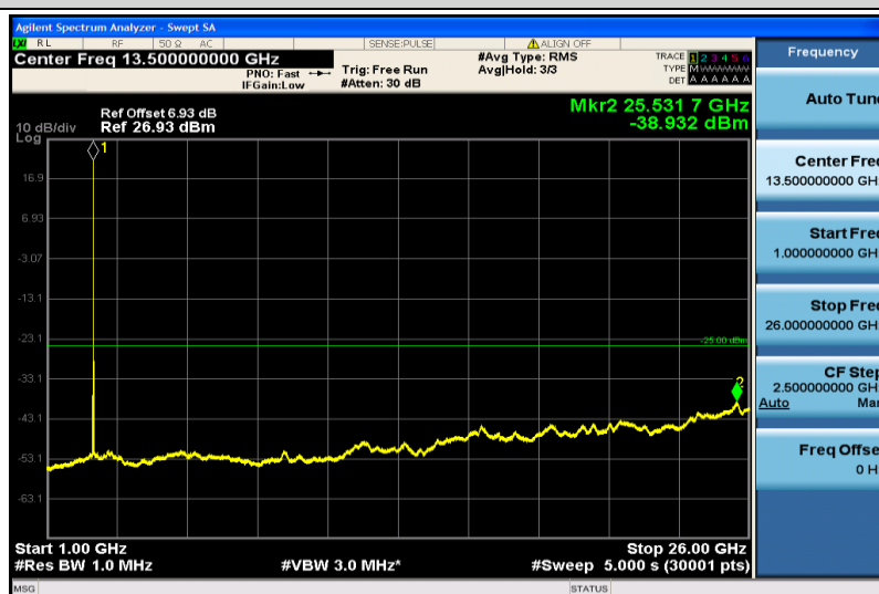
Band41-15MHz-16QAM-41165-1RB#0-1000~26000MHz
