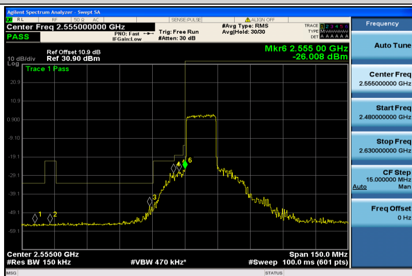
Band41-15MHz-QPSK-40315-75RB#0
