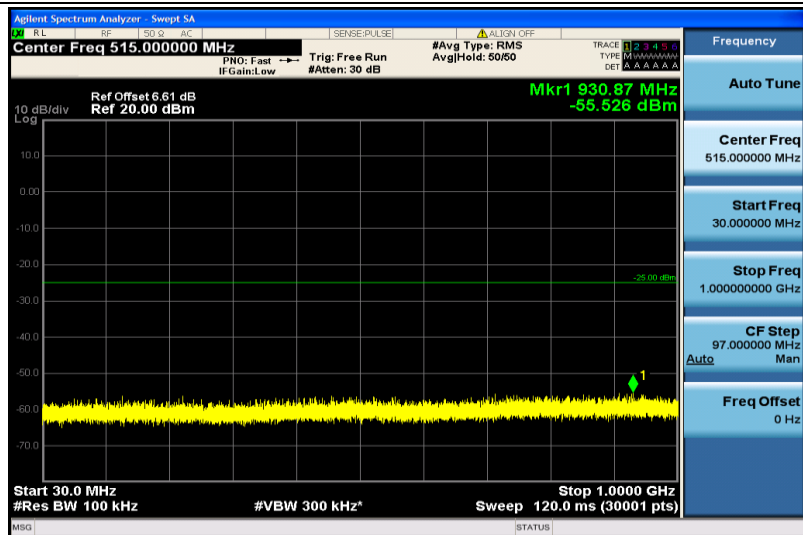
Band41-5MHz-16QAM-40265-1RB#0-30~1000MHz
