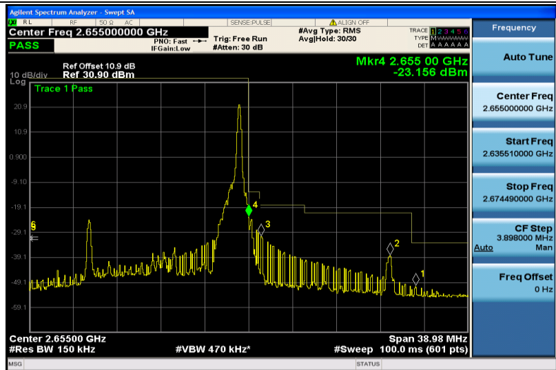
Band41-15MHz-QPSK-41165-1RB#74
