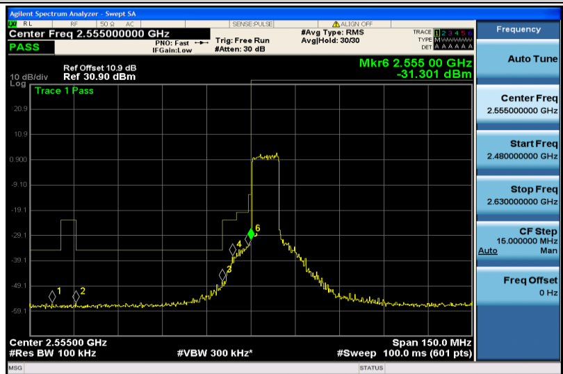
Band41-10MHz-16QAM-40290-50RB#0
