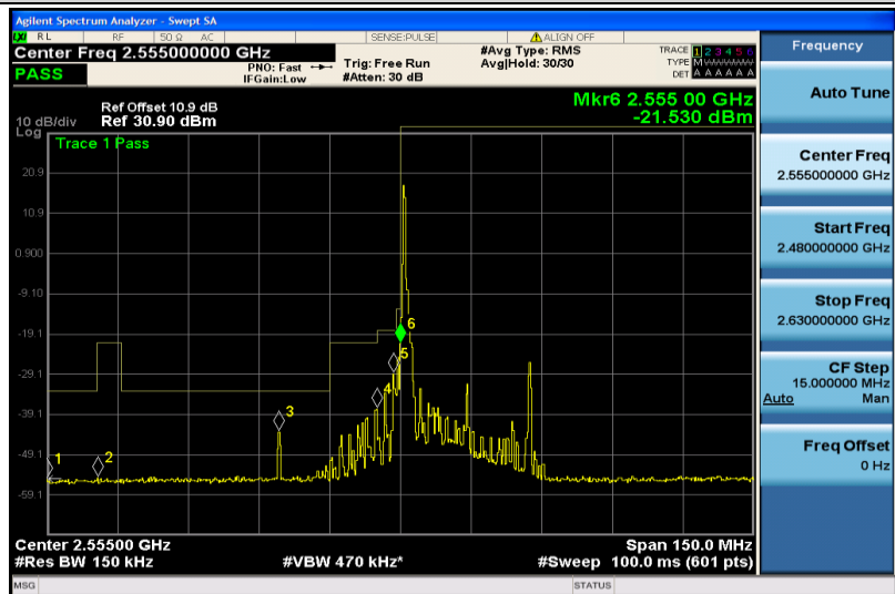
Band41-15MHz-16QAM-40315-1RB#0
