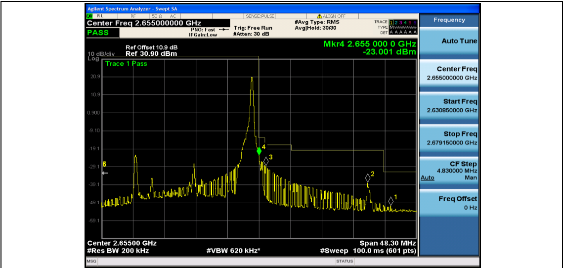
Band41-20MHz-16QAM-41140-1RB#99
