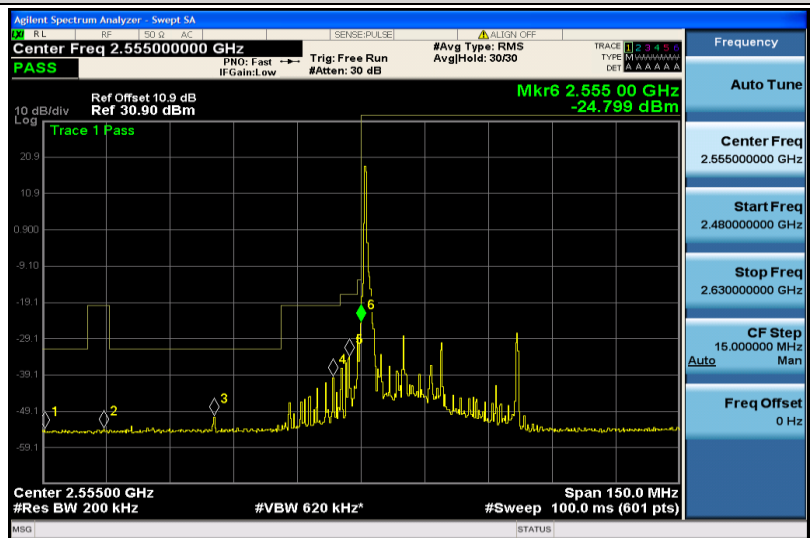
Band41-20MHz-16QAM-40340-1RB#0
