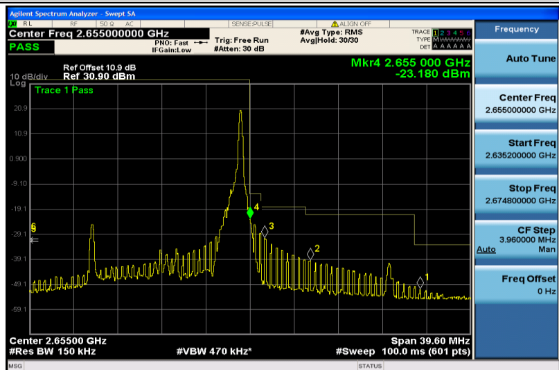
Band41-15MHz-16QAM-41165-1RB#74
