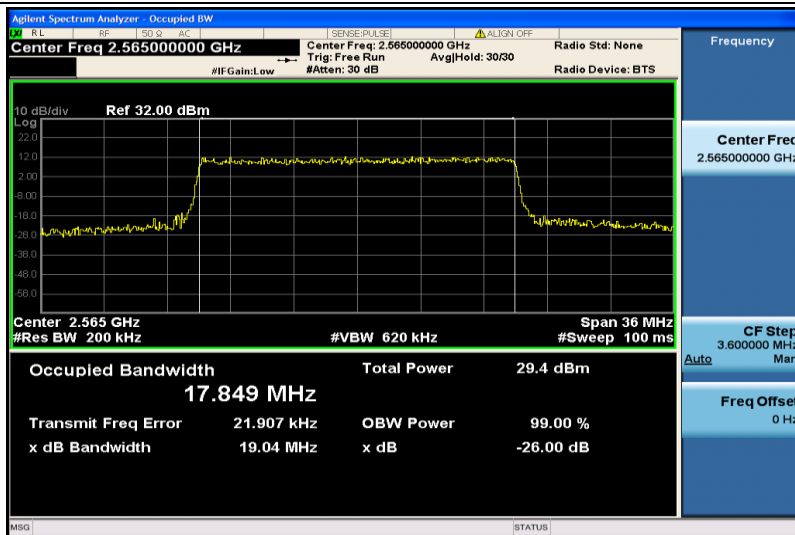
Band41-20MHz-16QAM-40340-100RB#0-17.849
