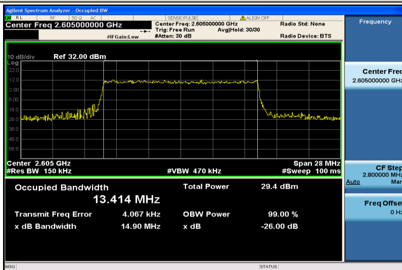
Band41-15MHz-16QAM-40740-75RB#0-13.414
