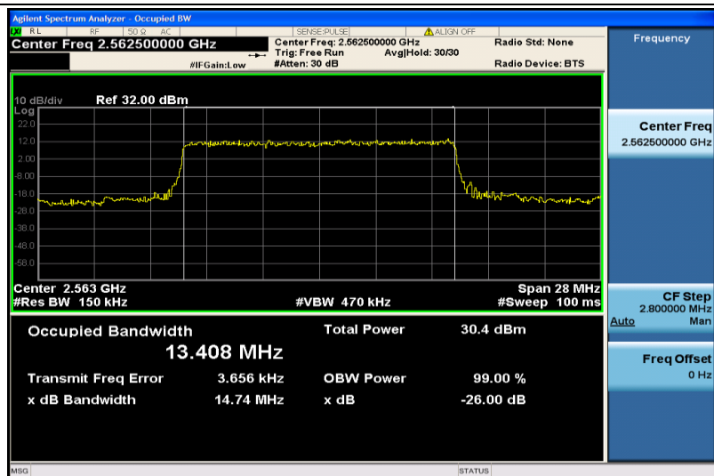
Band41-15MHz-QPSK-40315-75RB#0-13.408
