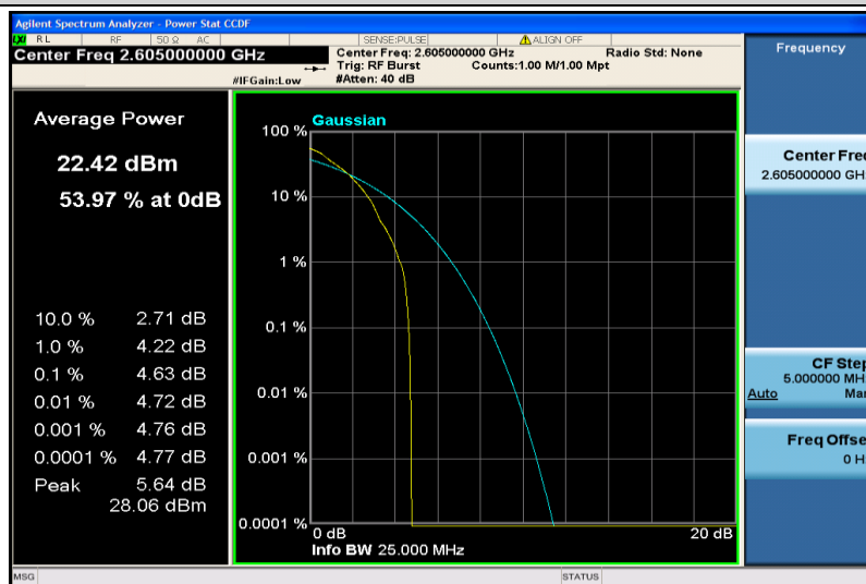
Band41-10MHz-QPSK-40740-1RB#0
