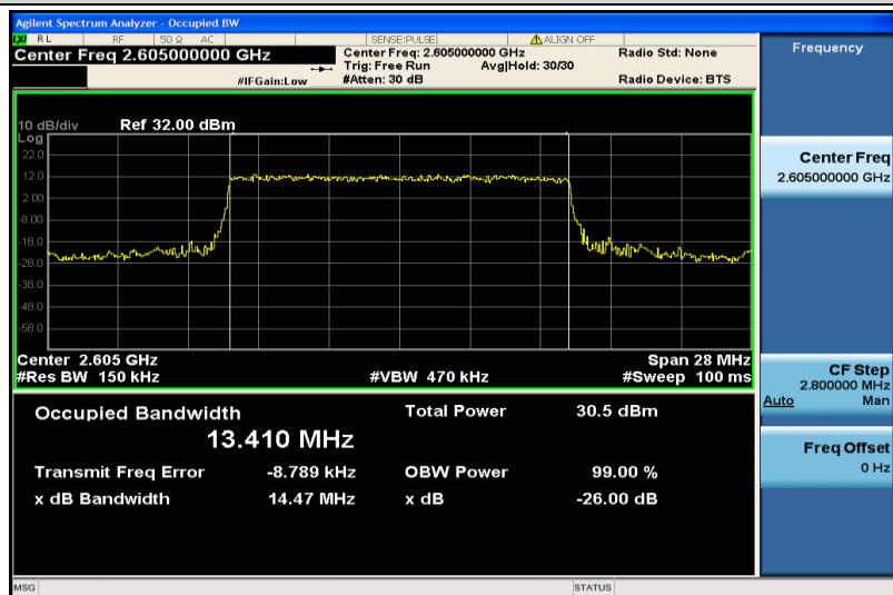
Band41-15MHz-QPSK-40740-75RB#0-13.410
