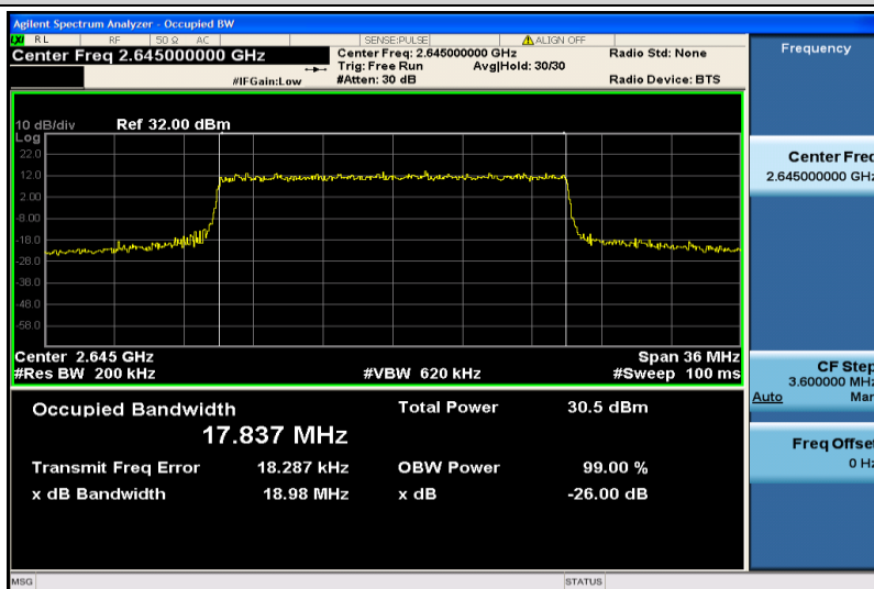
Band41-20MHz-QPSK-41140-100RB#0-17.837
