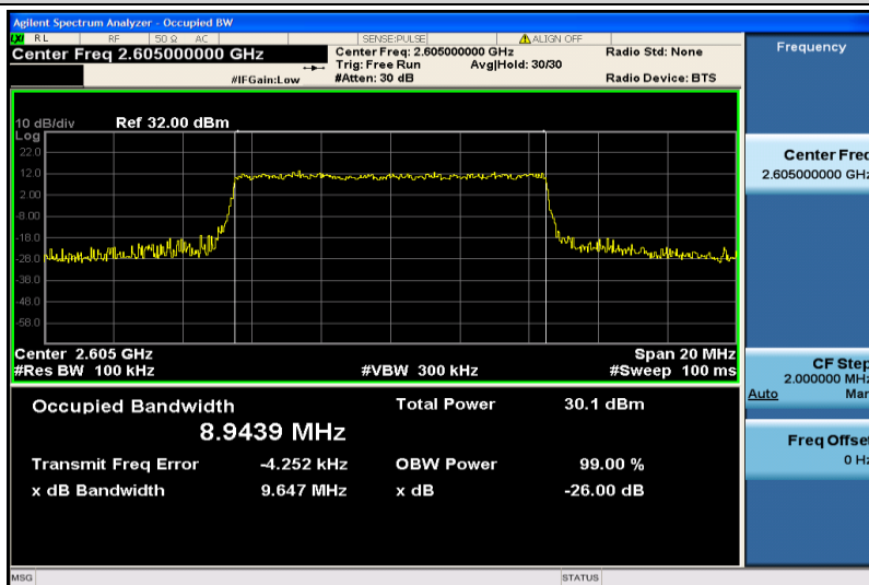
Band41-10MHz-QPSK-40740-50RB#0-8.9439
