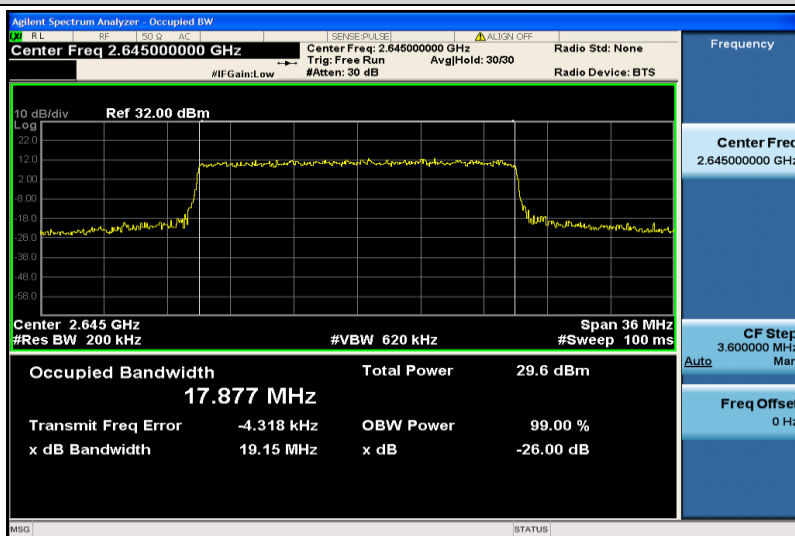
Band41-20MHz-16QAM-41140-100RB#0-17.877
