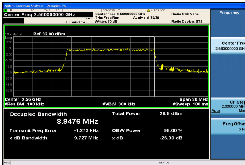
Band41-10MHz-16QAM-40290-50RB#0-8.9476
