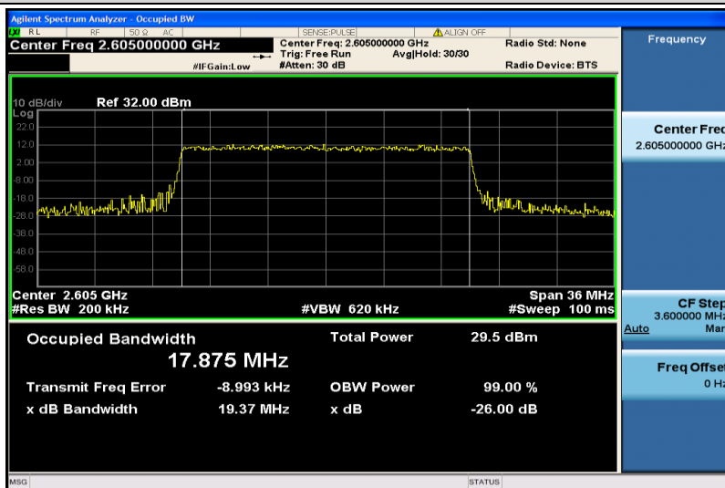
Band41-20MHz-16QAM-40740-100RB#0-17.875
