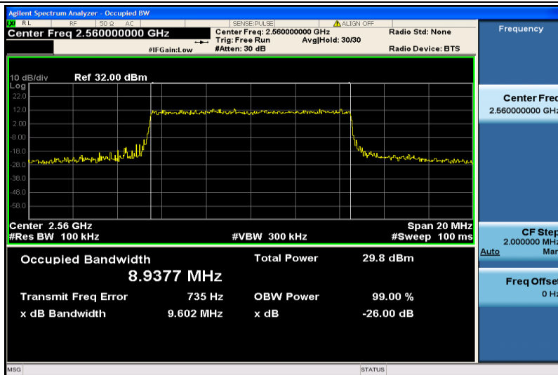
Band41-10MHz-QPSK-40290-50RB#0-8.9377
