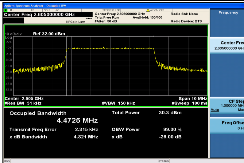
Band41-5MHz-QPSK-40740-25RB#0-4.4725
