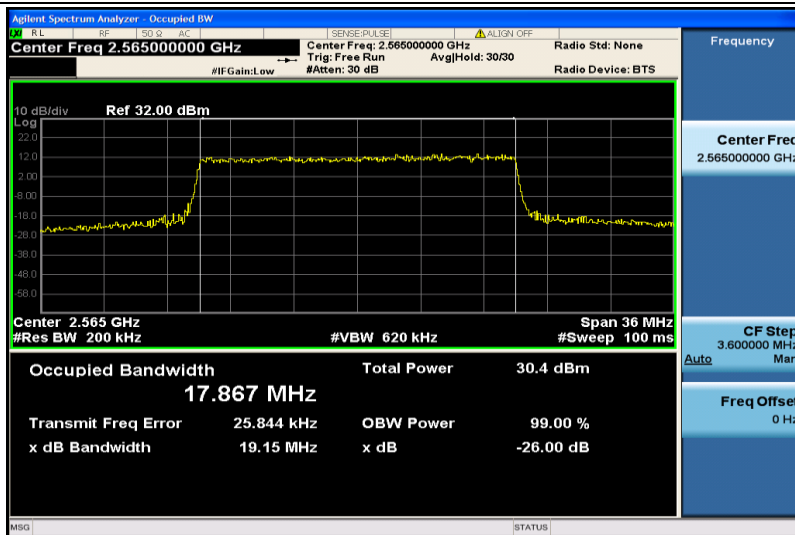
Band41-20MHz-QPSK-40340-100RB#0-17.867
