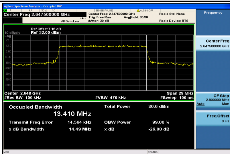
Band41-15MHz-QPSK-41165-75RB#0-13.410
