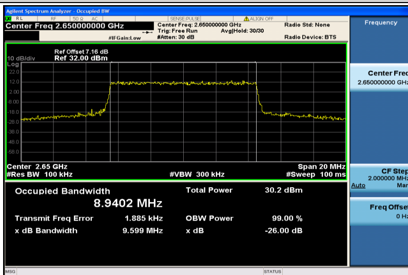
Band41-10MHz-QPSK-41190-50RB#0-8.9402
