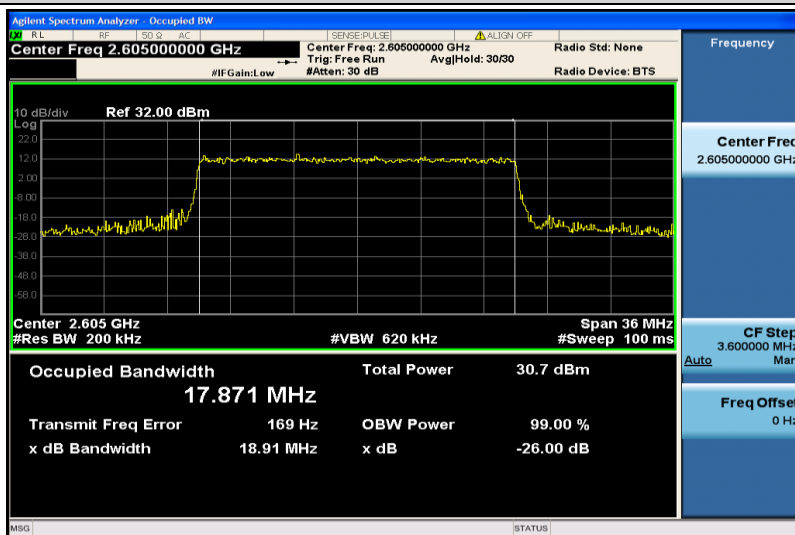
Band41-20MHz-QPSK-40740-100RB#0-17.871
