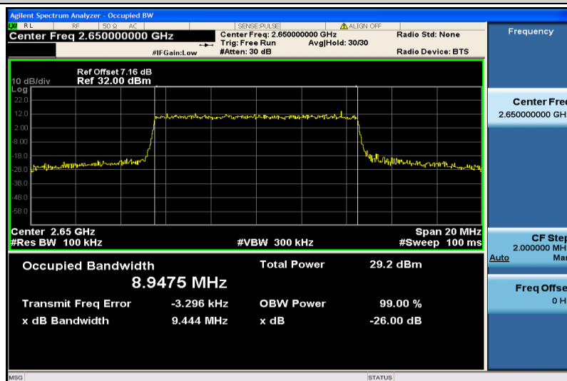
Band41-10MHz-16QAM-41190-50RB#0-8.9475
