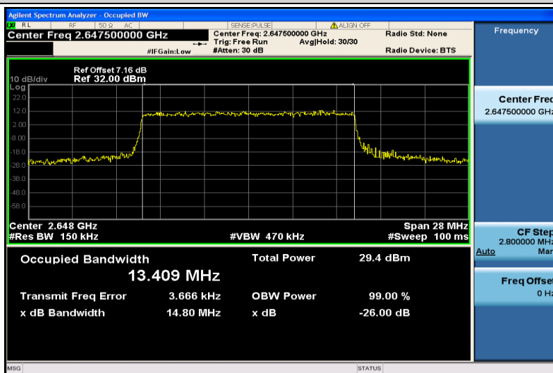
Band41-15MHz-16QAM-41165-75RB#0-13.409
