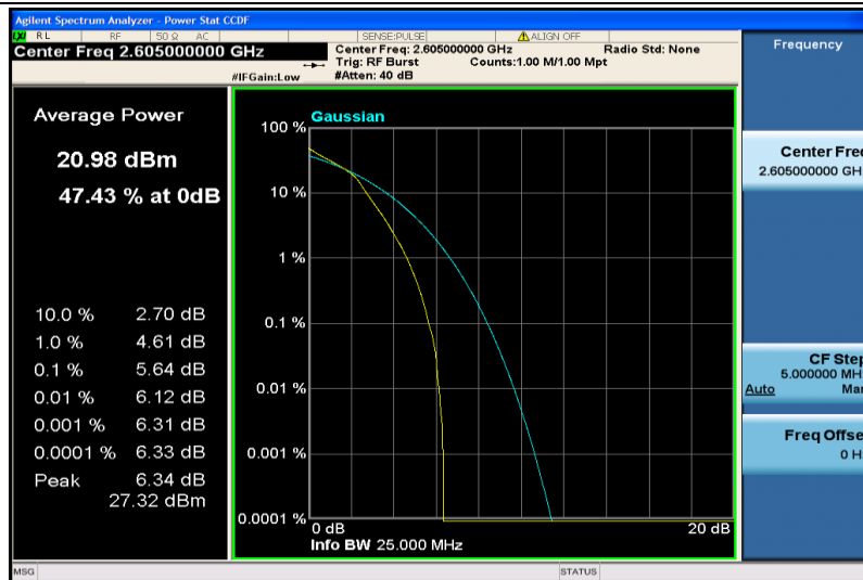
Band41-5MHz-16QAM-40740-25RB#0
