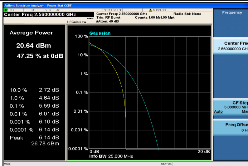
Band41-10MHz-16QAM-40290-50RB#0
