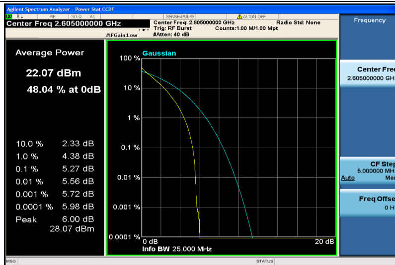
Band41-15MHz-QPSK-40740-75RB#0
