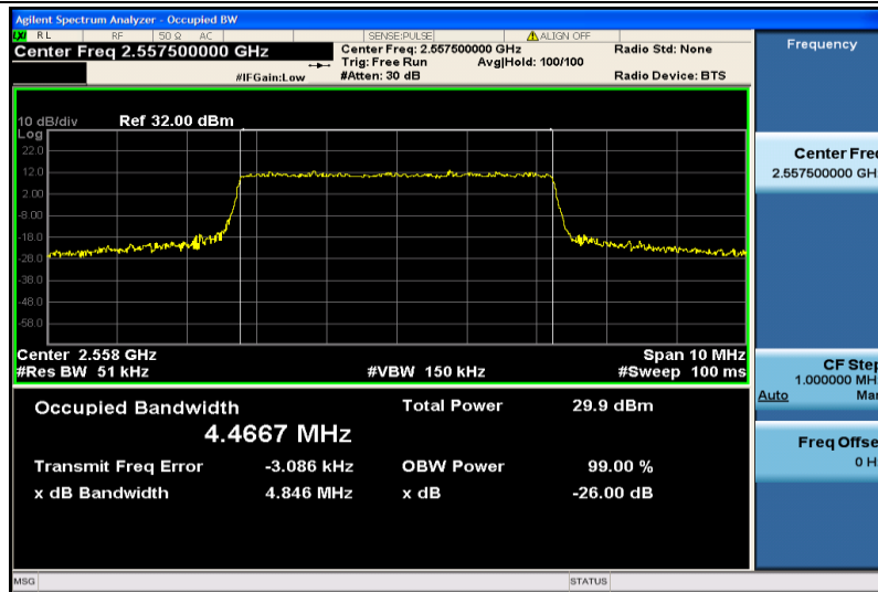
Band41-5MHz-QPSK-40265-25RB#0-4.4667
