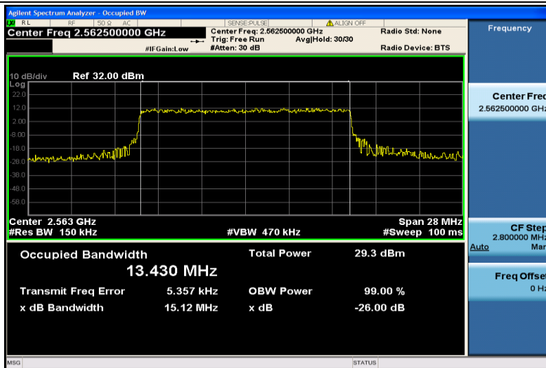
Band41-15MHz-16QAM-40315-75RB#0-13.430
