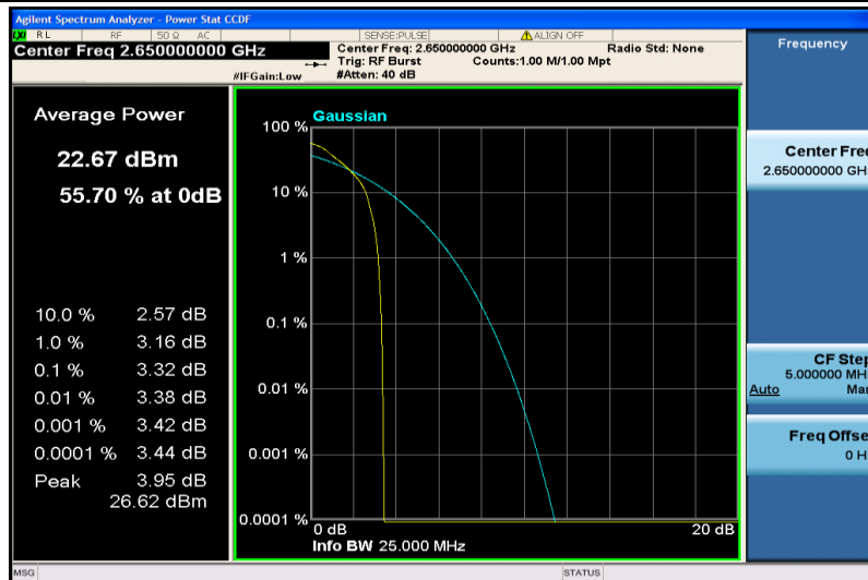
Band41-10MHz-QPSK-41190-1RB#0
