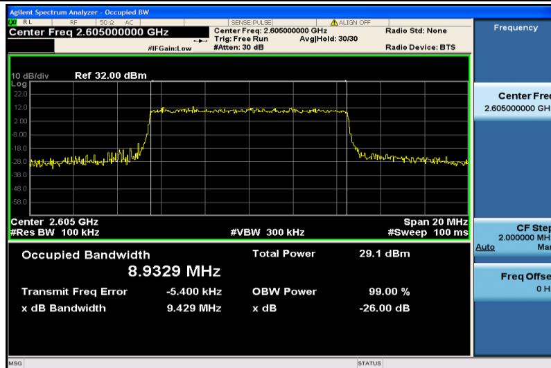
Band41-10MHz-16QAM-40740-50RB#0-8.9329
