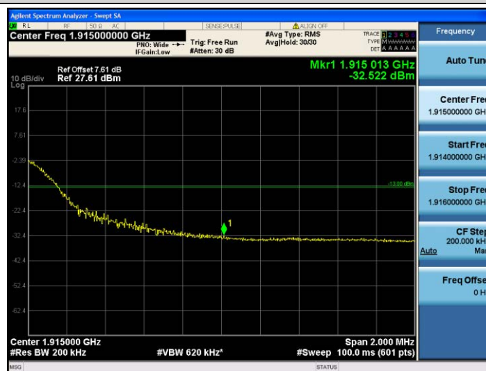
Band25-20MHz-16QAM-26590-100RB#0
