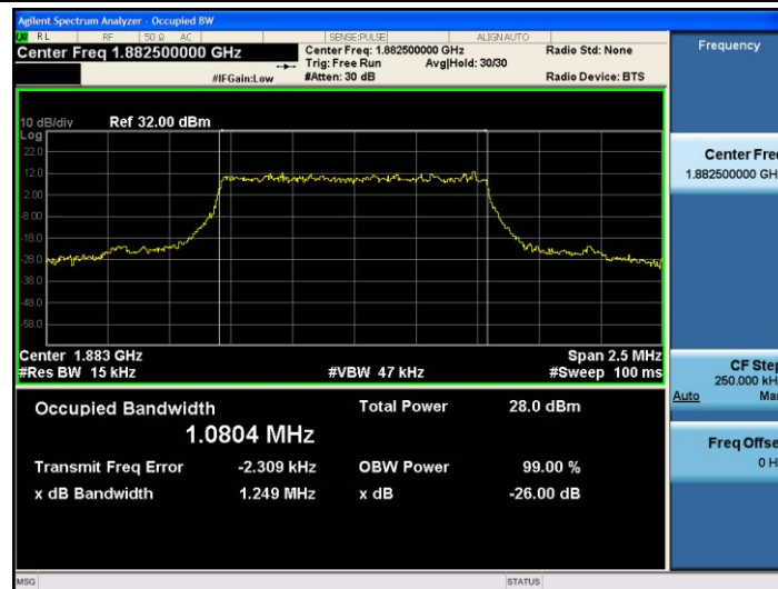
Band25-1.4MHz-QPSK-26365-6RB#0-1.0804
