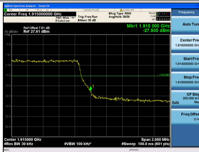
Band25-3MHz-16QAM-26675-15RB#0
