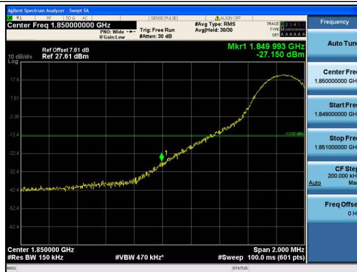
Band25-15MHz-16QAM-26115-1RB#0
