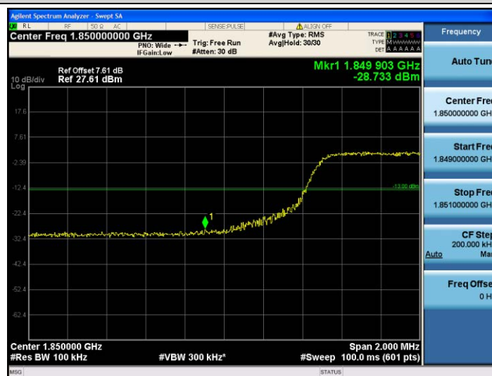
Band25-10MHz-16QAM-26090-50RB#0
