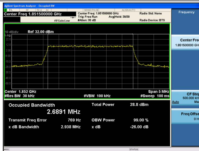
Band25-3MHz-QPSK-26055-15RB#0-2.6891
