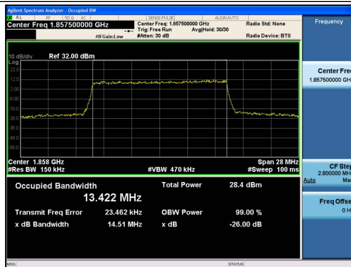
Band25-15MHz-16QAM-26115-75RB#0-13.422
