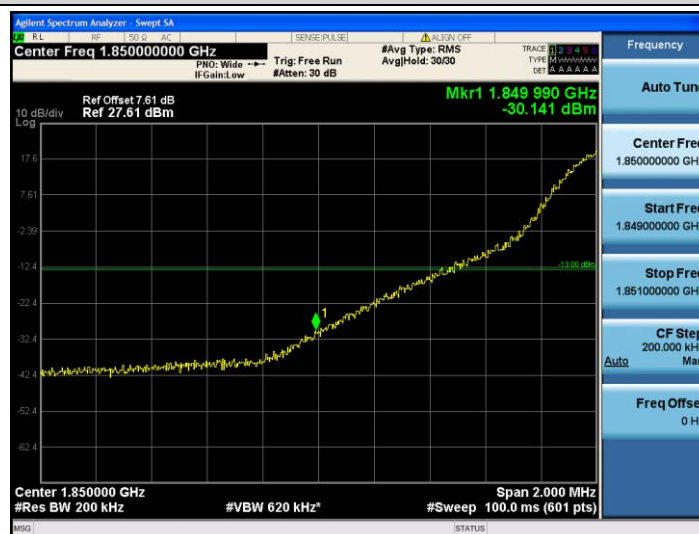
Band25-20MHz-16QAM-26140-1RB#0
