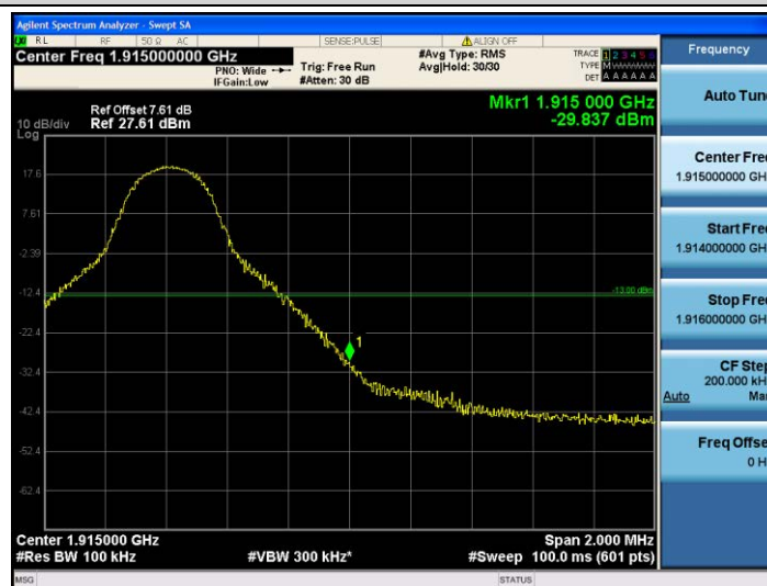
Band25-10MHz-QPSK-26640-1RB#49
