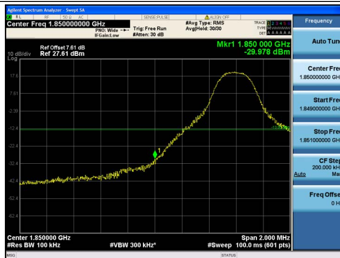
Band25-10MHz-QPSK-26090-1RB#0
