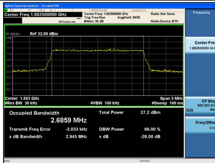
Band25-3MHz-16QAM-26365-15RB#0-2.6859
