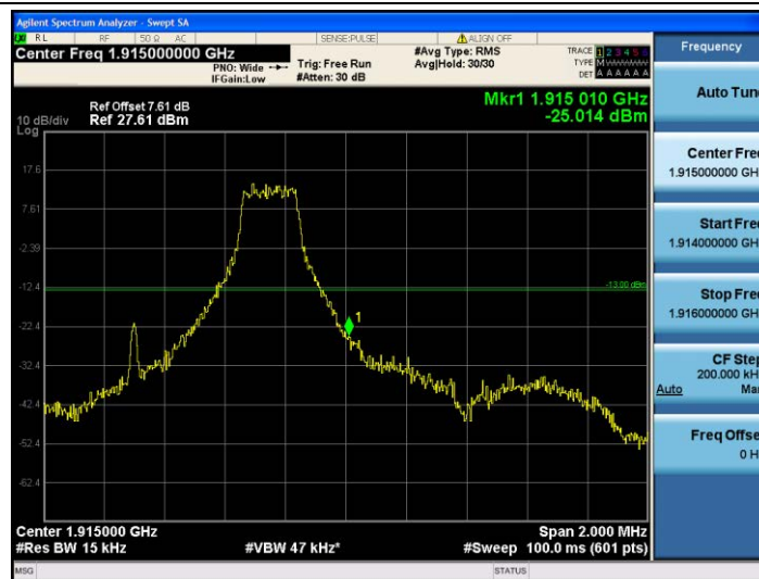
Band25-1.4MHz-16QAM-26683-1RB#5
