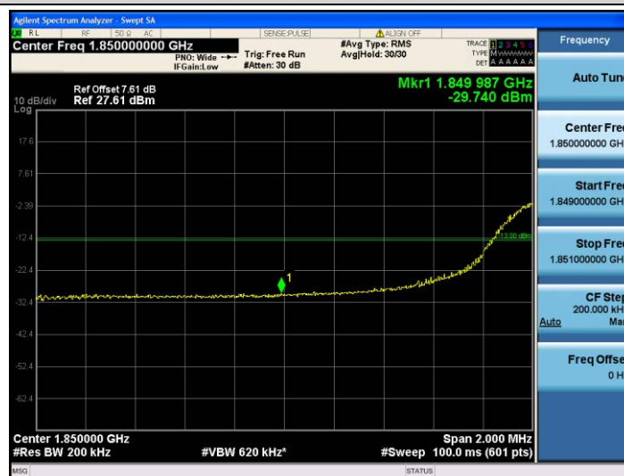
Band25-20MHz-QPSK-26140-100RB#0
