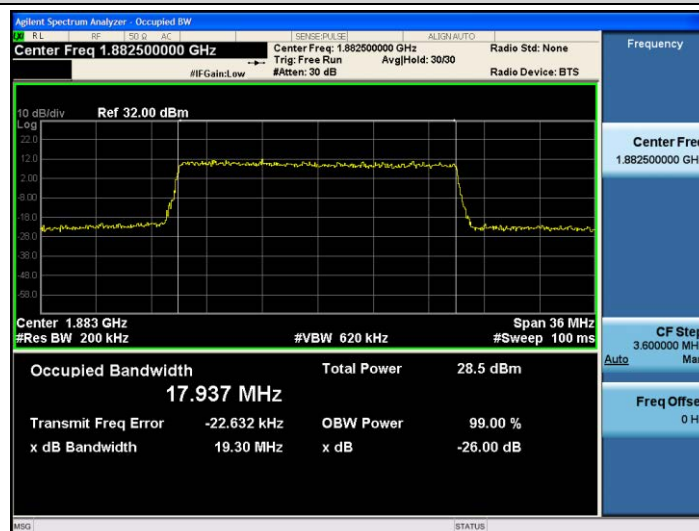
Band25-20MHz-16QAM-26365-100RB#0-17.937
