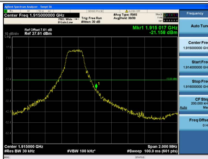
Band25-3MHz-16QAM-26675-1RB#14
