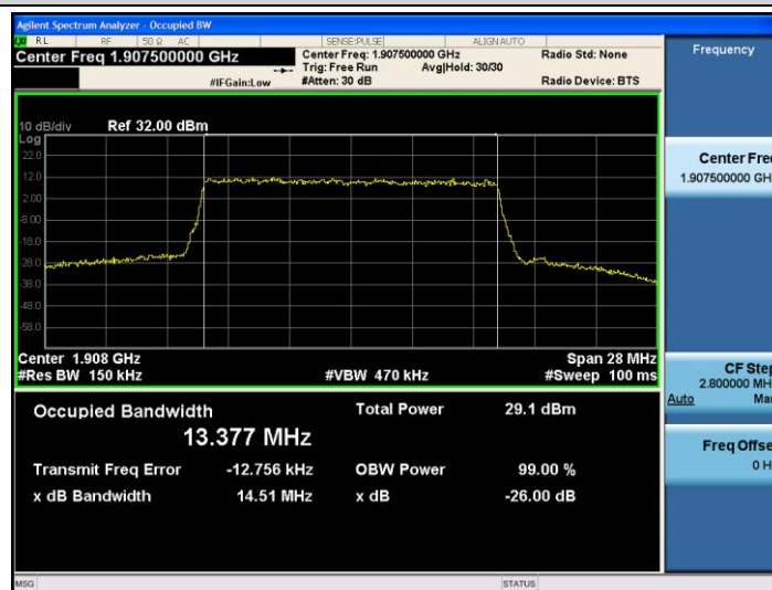
Band25-15MHz-QPSK-26615-75RB#0-13.377
