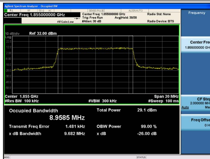
Band25-10MHz-QPSK-26090-50RB#0-8.9585
