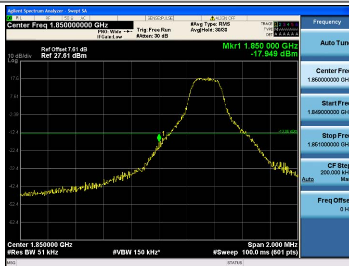
Band25-5MHz-QPSK-26065-1RB#0
