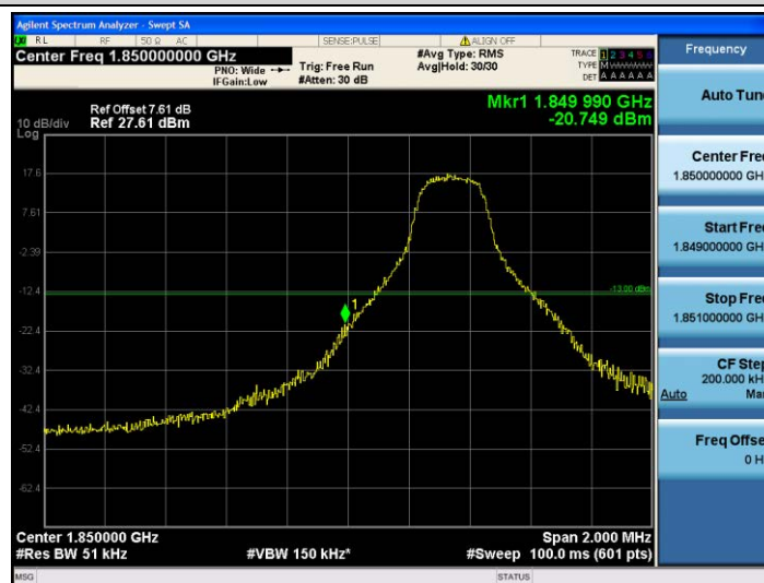
Band25-5MHz-16QAM-26065-1RB#0
