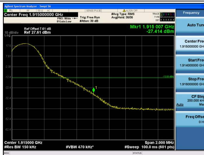
Band25-15MHz-QPSK-26615-1RB#74
