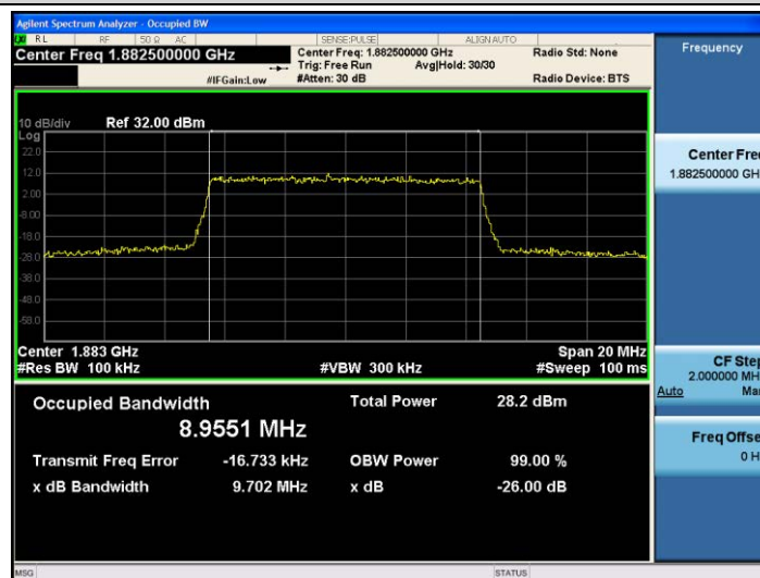
Band25-10MHz-16QAM-26365-50RB#0-8.9551
