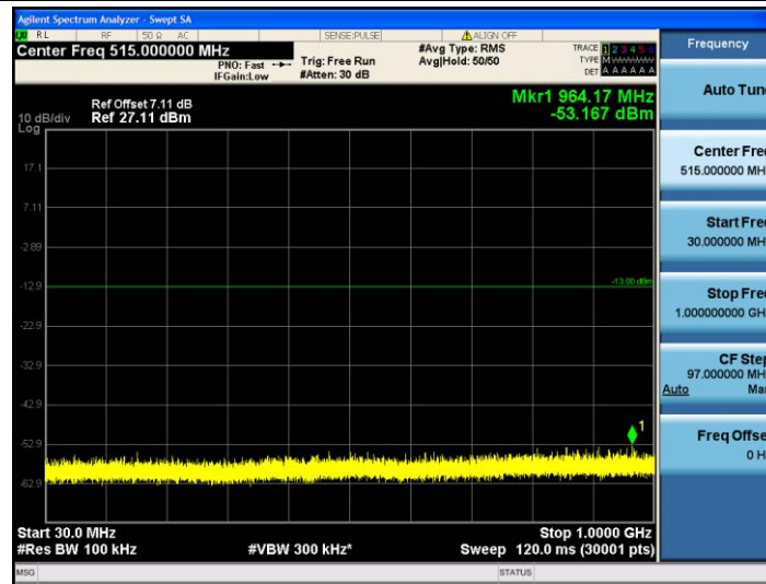
Band25-1.4MHz-QPSK-26047-1RB#0-30~1000MHz
