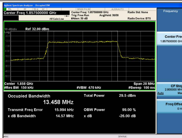
Band25-15MHz-QPSK-26115-75RB#0-13.458
