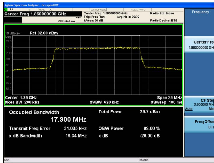
Band25-20MHz-QPSK-26140-100RB#0-17.900
