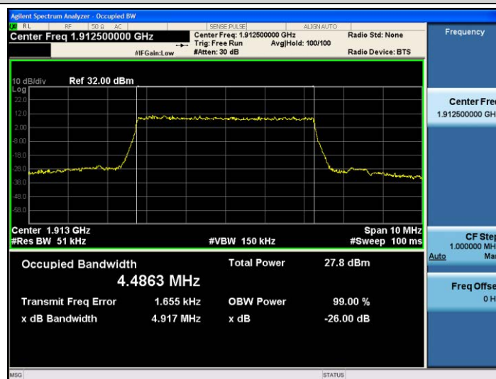
Band25-5MHz-16QAM-26665-25RB#0-4.4863
