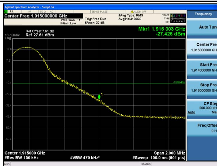
Band25-15MHz-16QAM-26615-1RB#74
