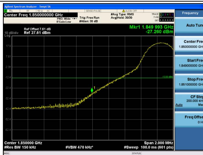
Band25-15MHz-QPSK-26115-1RB#0
