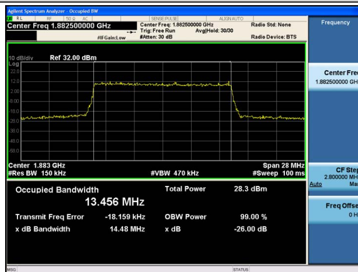
Band25-15MHz-16QAM-26365-75RB#0-13.456
