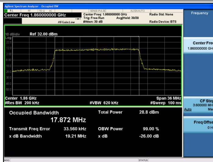
Band25-20MHz-16QAM-26140-100RB#0-17.872
