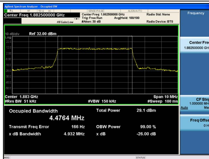
Band25-5MHz-QPSK-26365-25RB#0-4.4764
