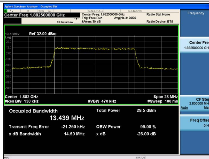
Band25-15MHz-QPSK-26365-75RB#0-13.439
