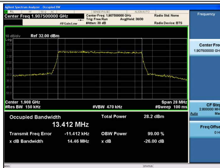
Band25-15MHz-16QAM-26615-75RB#0-13.412
