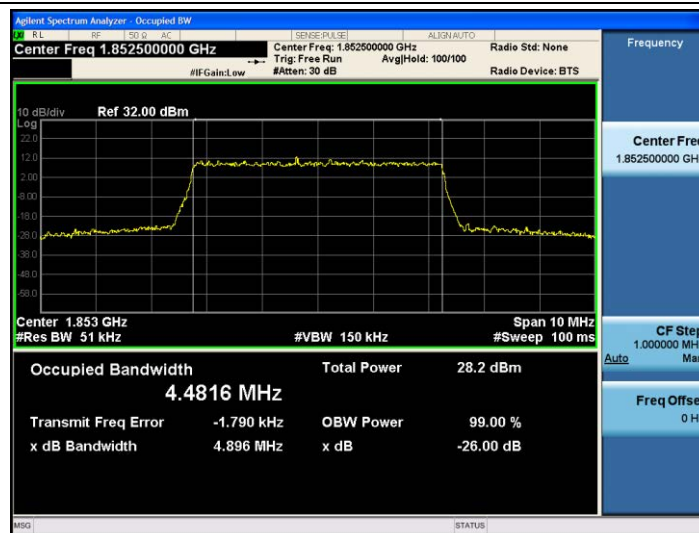
Band25-5MHz-16QAM-26065-25RB#0-4.4816
