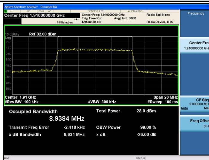
Band25-10MHz-16QAM-26640-50RB#0-8.9384
