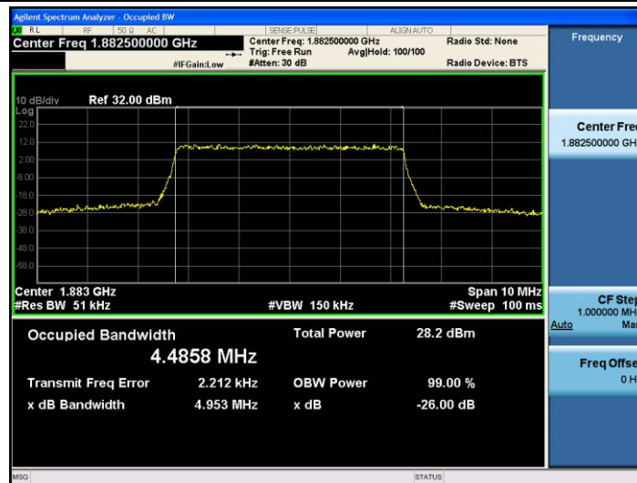
Band25-5MHz-16QAM-26365-25RB#0-4.4858
