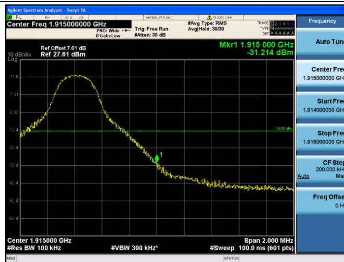
Band25-10MHz-16QAM-26640-1RB#49
