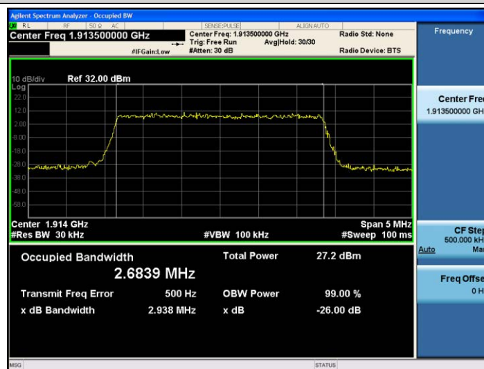
Band25-3MHz-16QAM-26675-15RB#0-2.6839
