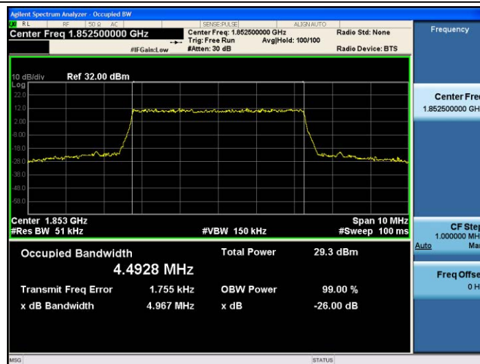
Band25-5MHz-QPSK-26065-25RB#0-4.4928
