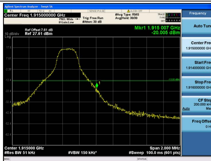
Band25-5MHz-16QAM-26665-1RB#24
