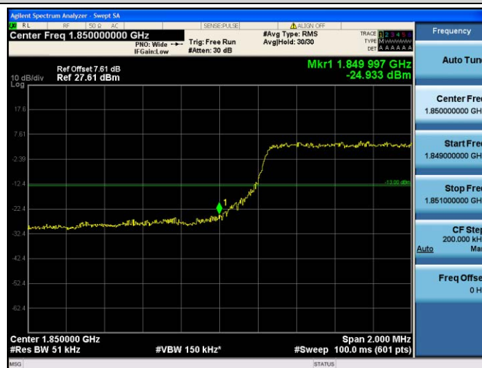
Band25-5MHz-QPSK-26065-25RB#0
