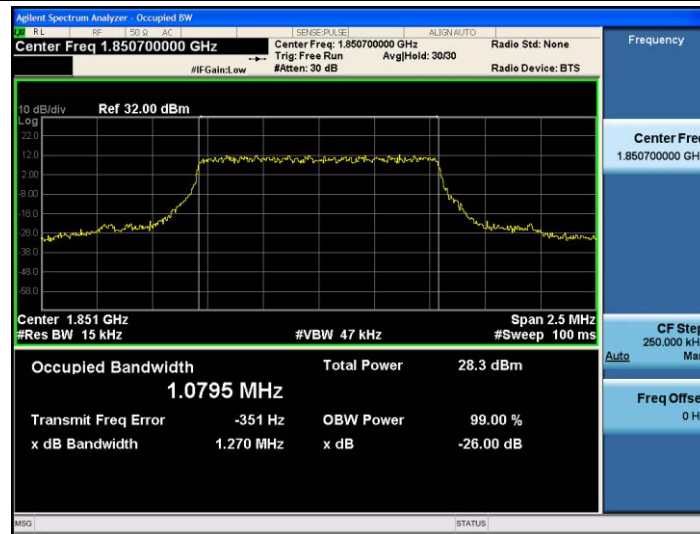
Band25-1.4MHz-QPSK-26047-6RB#0-1.0795
