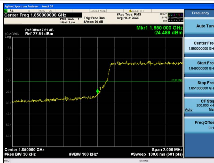
Band25-3MHz-QPSK-26055-15RB#0
