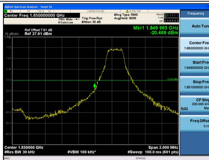
Band25-3MHz-QPSK-26055-1RB#0
