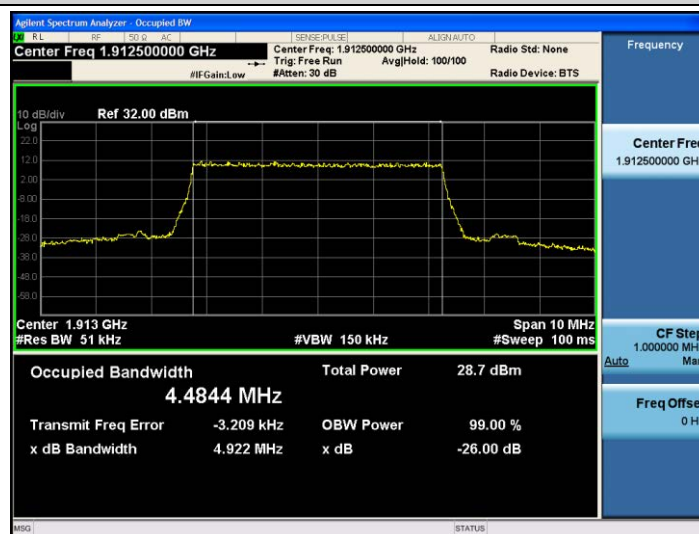
Band25-5MHz-QPSK-26665-25RB#0-4.4844
