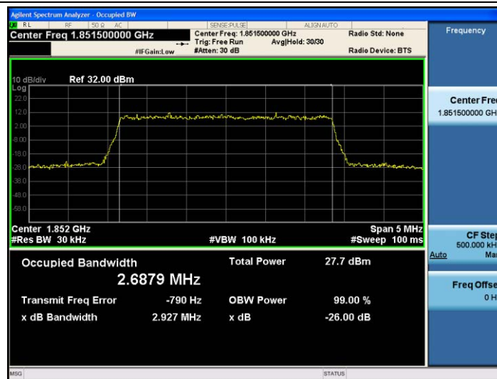
Band25-3MHz-16QAM-26055-15RB#0-2.6879
