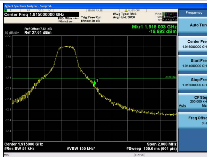
Band25-5MHz-QPSK-26665-1RB#24
