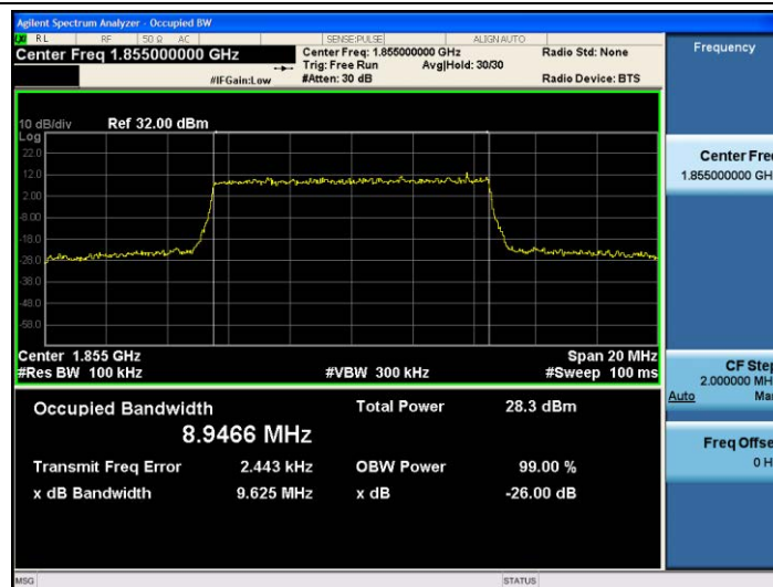
Band25-10MHz-16QAM-26090-50RB#0-8.9466
