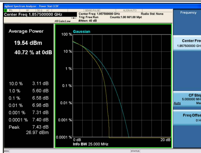
Band25-15MHz-16QAM-26115-75RB#0
