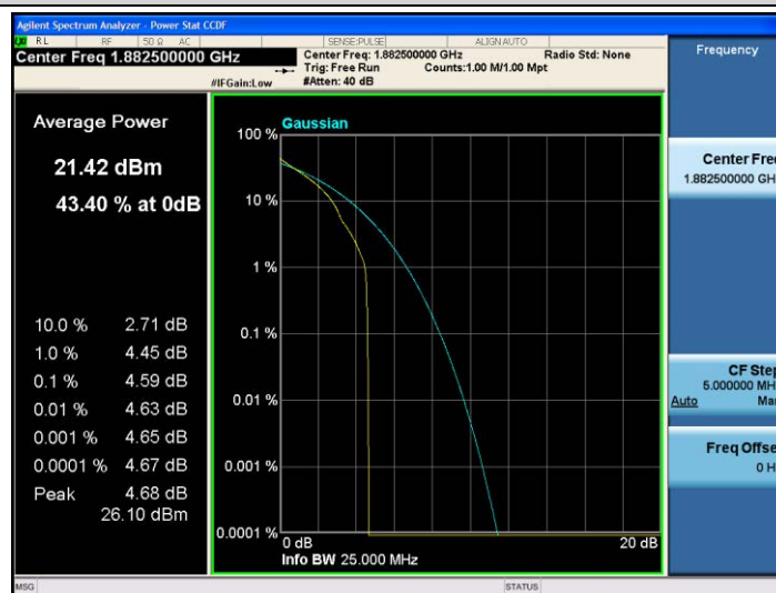
Band25-15MHz-QPSK-26365-1RB#0
