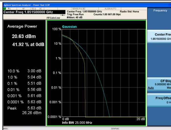
Band25-3MHz-16QAM-26055-1RB#0
