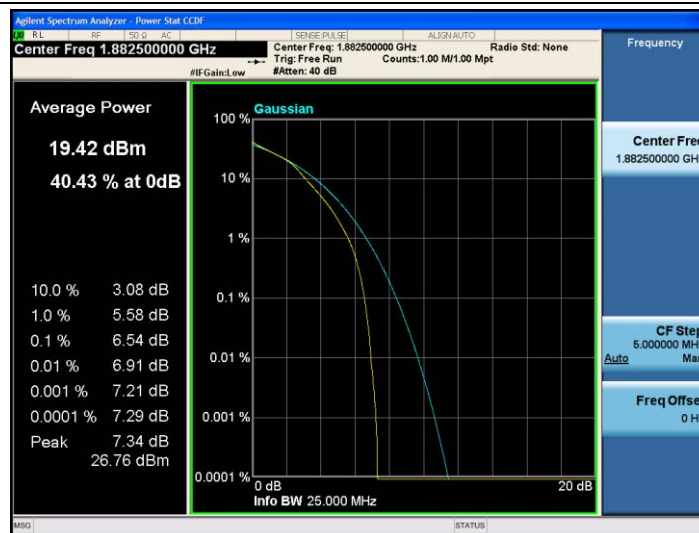
Band25-15MHz-16QAM-26365-75RB#0
