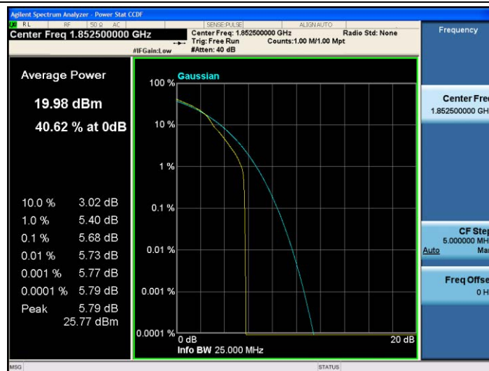
Band25-5MHz-16QAM-26065-1RB#0
