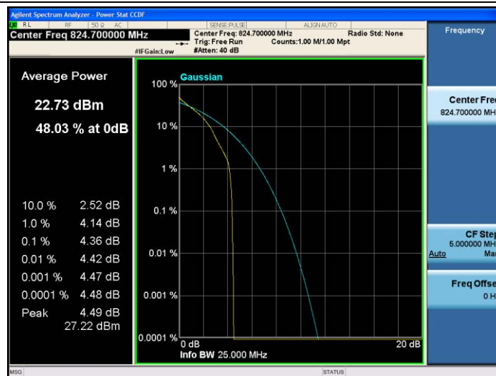
Band26-1.4MHz-QPSK-26797-1RB#0
