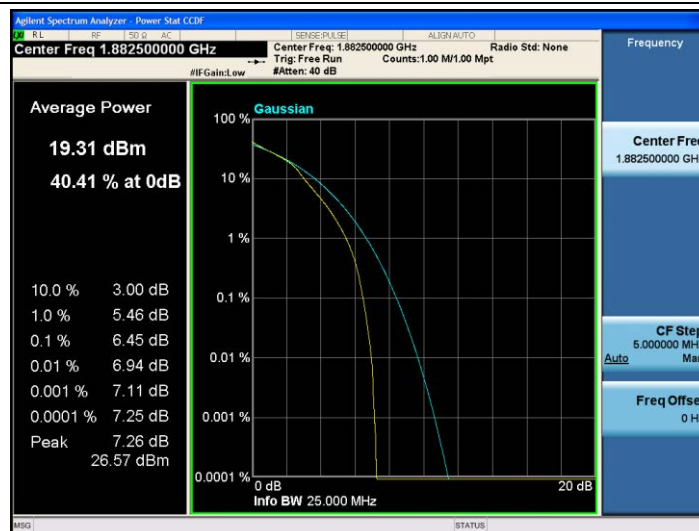
Band25-5MHz-16QAM-26365-25RB#0
