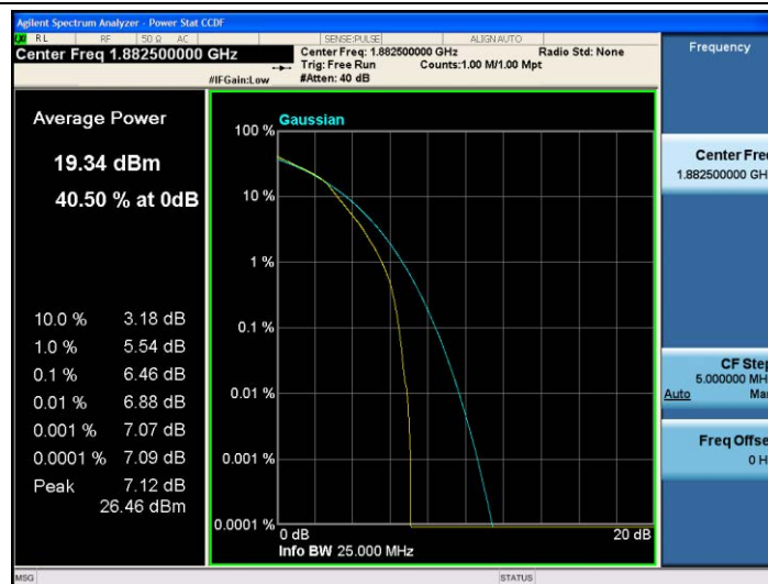
Band25-1.4MHz-16QAM-26365-6RB#0
