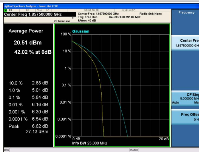
Band25-15MHz-QPSK-26115-75RB#0
