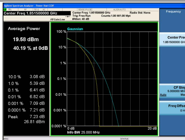
Band25-3MHz-16QAM-26055-15RB#0
