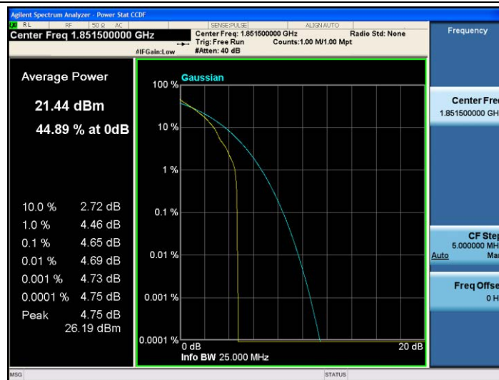
Band25-3MHz-QPSK-26055-1RB#0
