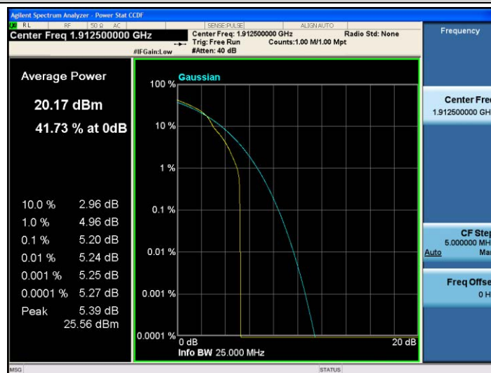
Band25-5MHz-16QAM-26665-1RB#0
