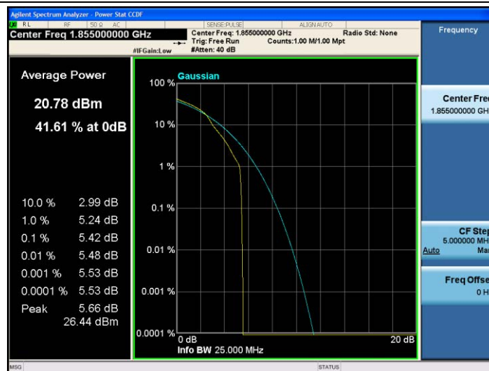
Band25-10MHz-16QAM-26090-1RB#0
