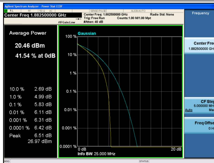
Band25-15MHz-QPSK-26365-75RB#0
