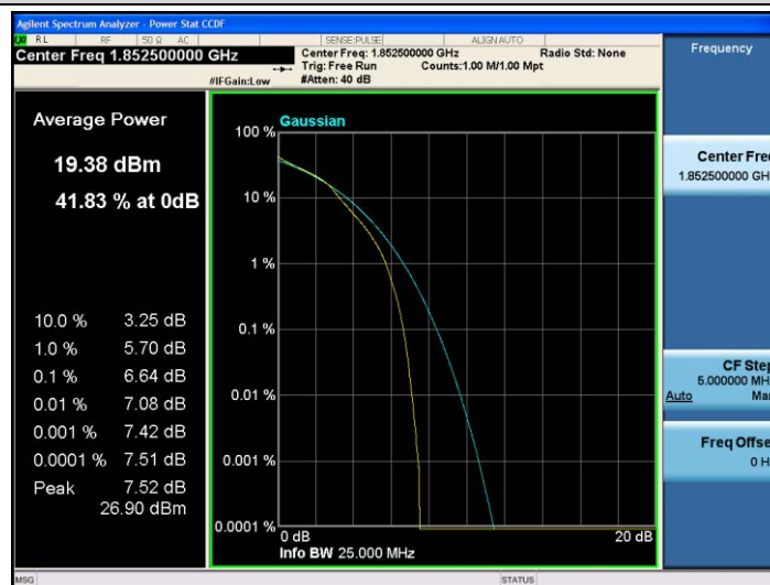
Band25-5MHz-16QAM-26065-25RB#0
