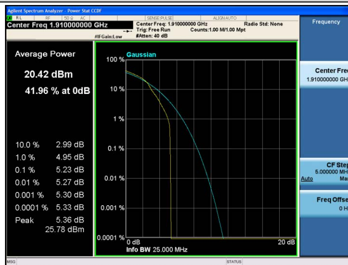
Band25-10MHz-16QAM-26640-1RB#0
