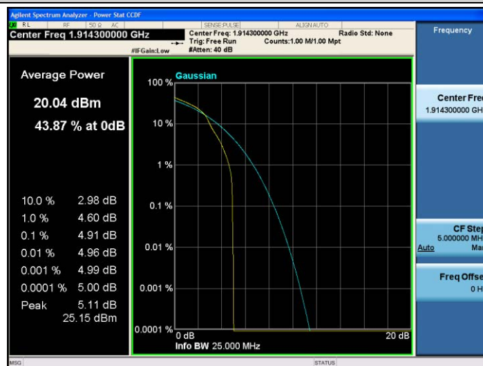
Band25-1.4MHz-16QAM-26683-1RB#0
