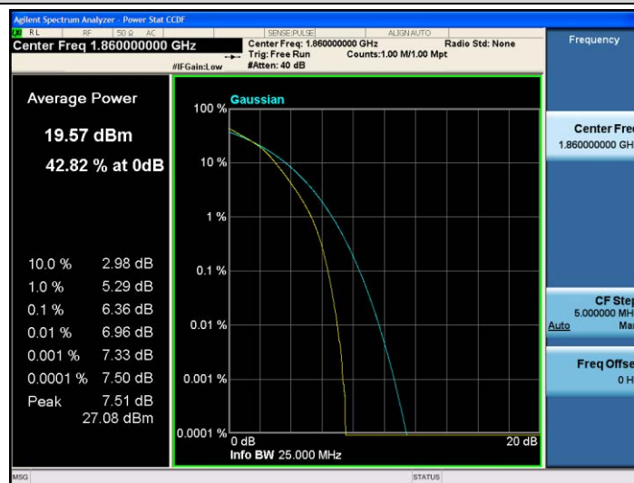
Band25-20MHz-16QAM-26140-100RB#0
