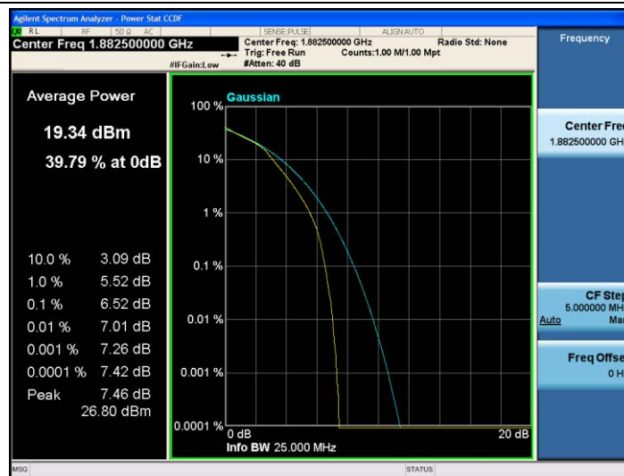
Band25-3MHz-16QAM-26365-15RB#0
