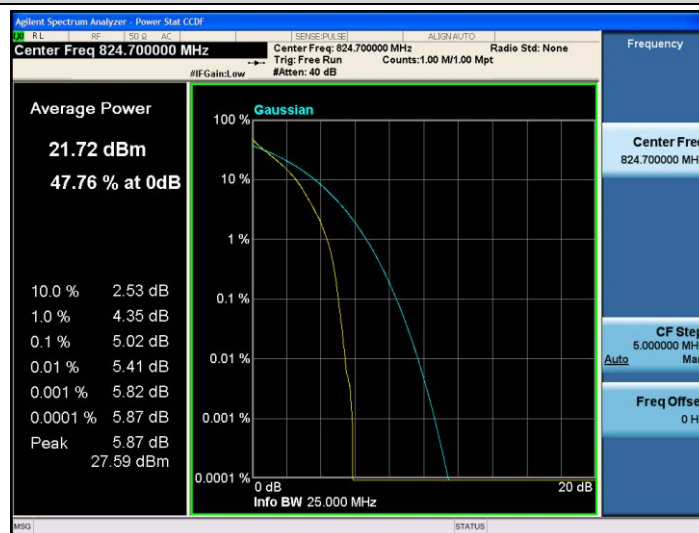
Band26-1.4MHz-QPSK-26797-6RB#0
