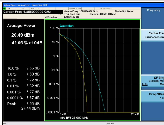
Band25-10MHz-QPSK-26090-50RB#0
