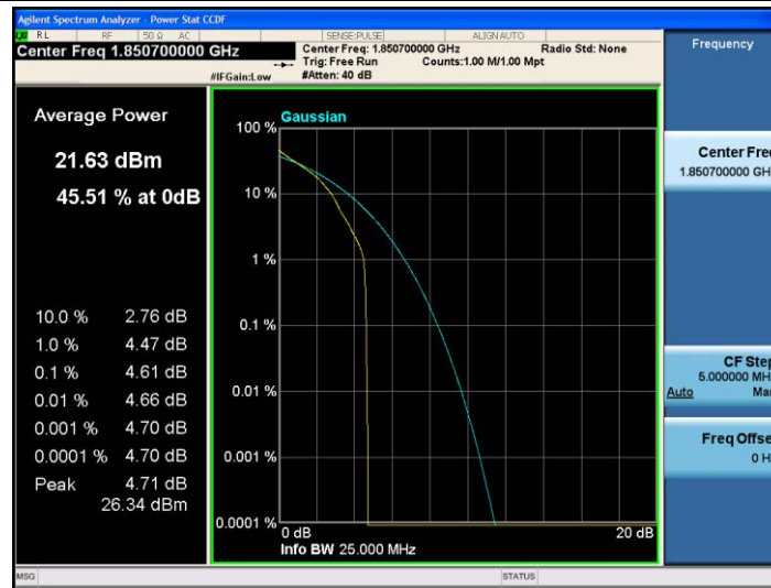
Band25-1.4MHz-QPSK-26047-1RB#0
