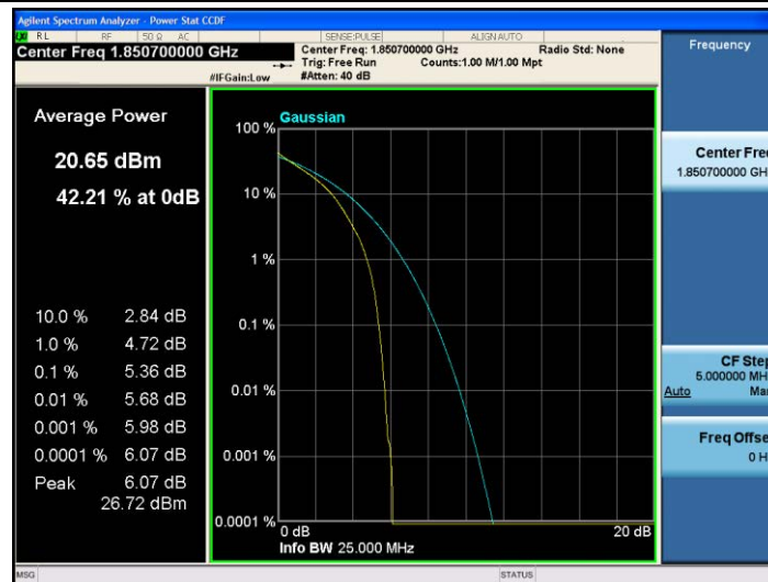
Band25-1.4MHz-QPSK-26047-6RB#0
