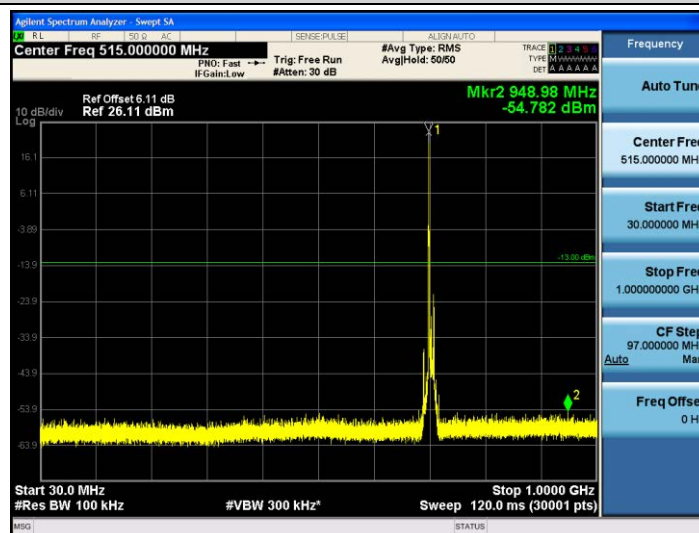
Band17-10MHz-QPSK-23800-1RB#0-30~1000MHz
