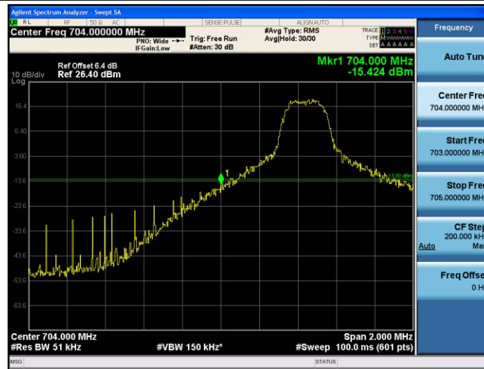
Band17-5MHz-QPSK-23755-1RB#0
