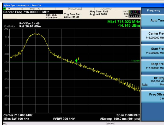
Band17-10MHz-16QAM-23800-1RB#49
