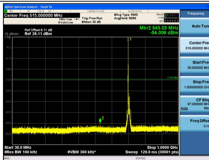
Band17-10MHz-16QAM-23790-1RB#0-30~1000MHz
