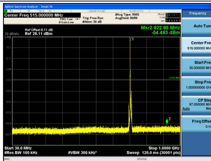
Band17-5MHz-16QAM-23825-1RB#0-30~1000MHz
