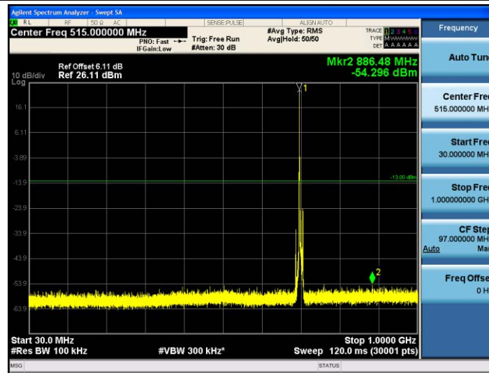
Band17-5MHz-QPSK-23755-1RB#0-30~1000MHz
