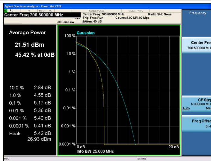
Band17-5MHz-16QAM-23755-1RB#0
