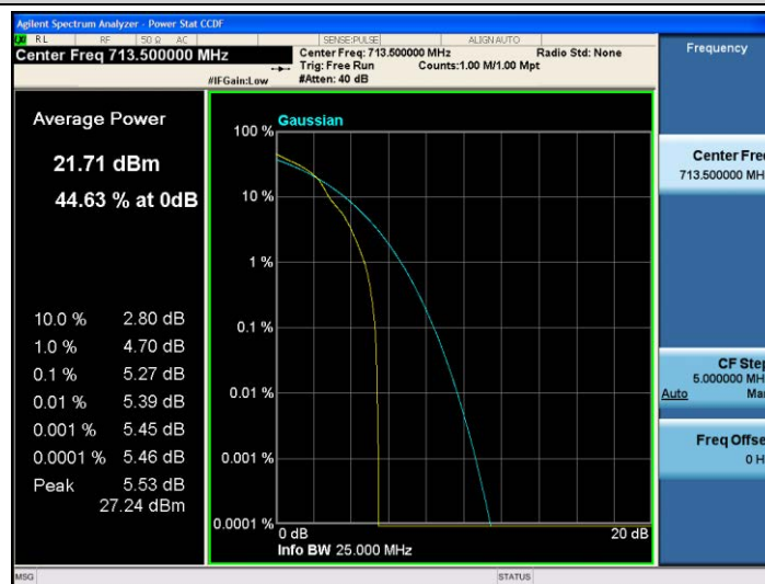
Band17-5MHz-16QAM-23825-1RB#0
