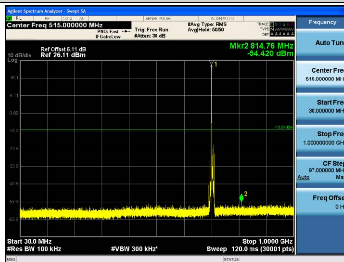
Band17-5MHz-16QAM-23790-1RB#0-30~1000MHz
