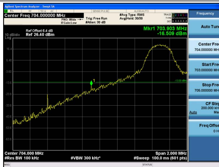
Band17-10MHz-16QAM-23780-1RB#0
