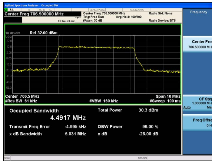
Band17-5MHz-QPSK-23755-25RB#0-4.4917
