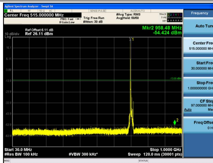
Band17-10MHz-16QAM-23780-1RB#0-30~1000MHz
