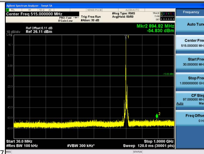
Band17-10MHz-16QAM-23800-1RB#0-30~1000MHz
