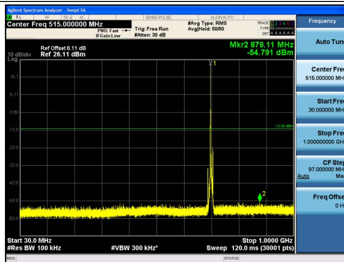
Band17-5MHz-16QAM-23755-1RB#0-30~1000MHz
