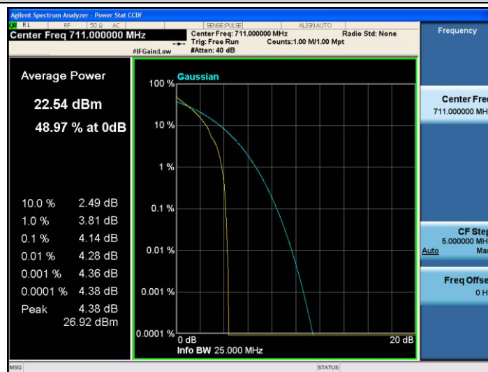
Band17-10MHz-QPSK-23800-1RB#0
