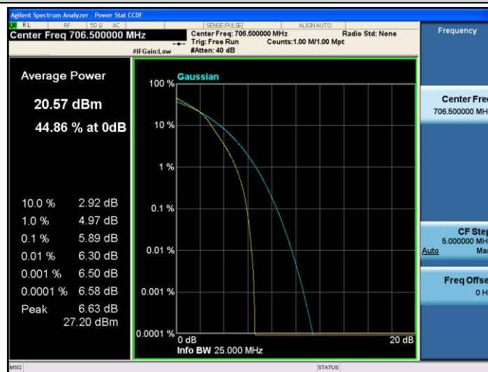
Band17-5MHz-16QAM-23755-25RB#0
