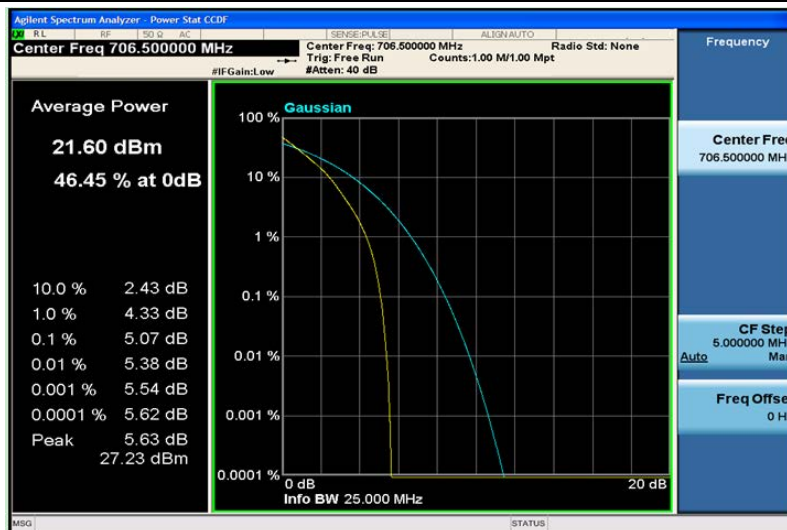
Band17-5MHz-QPSK-23755-25RB#0
