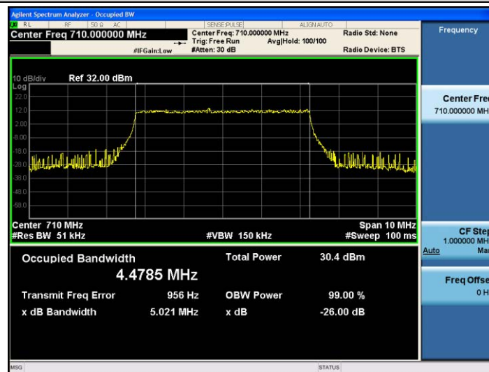
Band17-5MHz-QPSK-23790-25RB#0-4.4785
