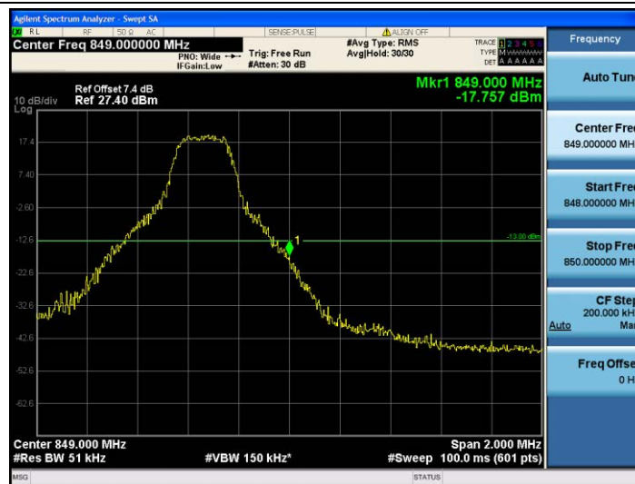
Band5-5MHz-QPSK-20625-1RB#24
