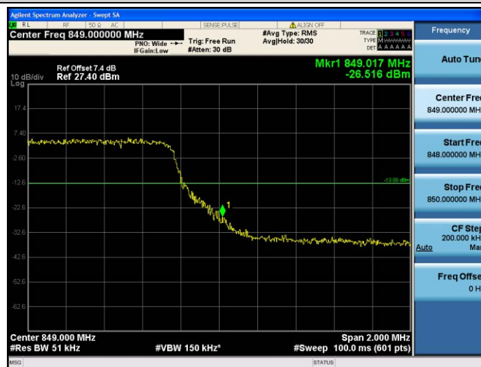
Band5-5MHz-QPSK-20625-25RB#0
