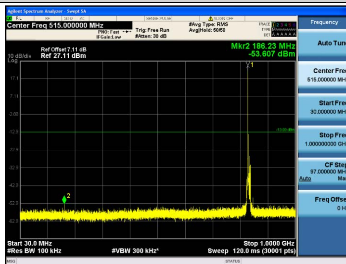
Band5-10MHz-QPSK-20525-1RB#0-30~1000MHz
