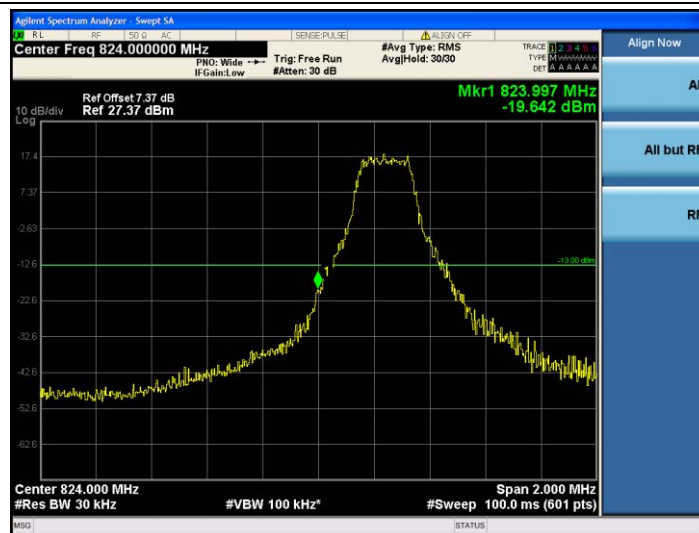
Band5-3MHz-16QAM-20415-1RB#0
