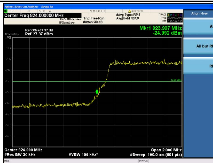
Band5-3MHz-16QAM-20415-15RB#0
