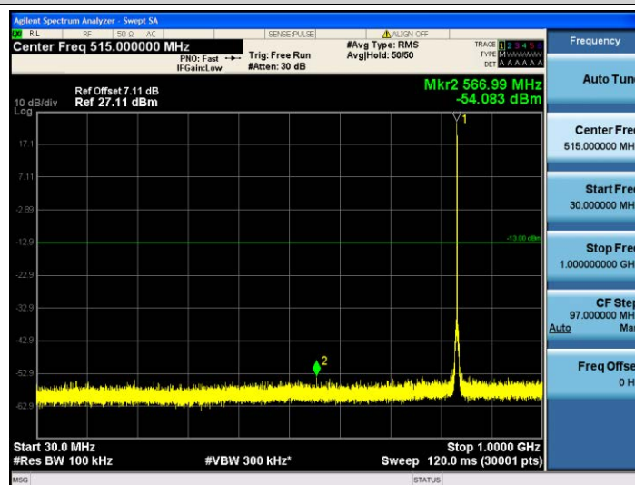
Band5-1.4MHz-16QAM-20525-1RB#0-30~1000MHz
