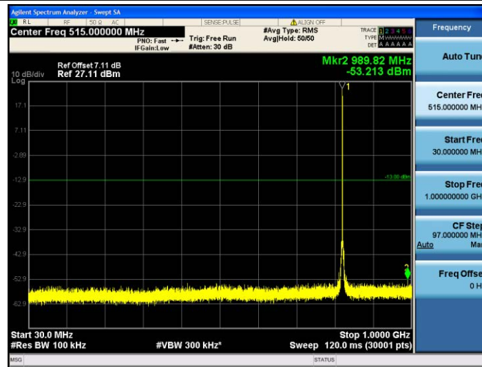
Band5-1.4MHz-QPSK-20407-1RB#0-30~1000MHz
