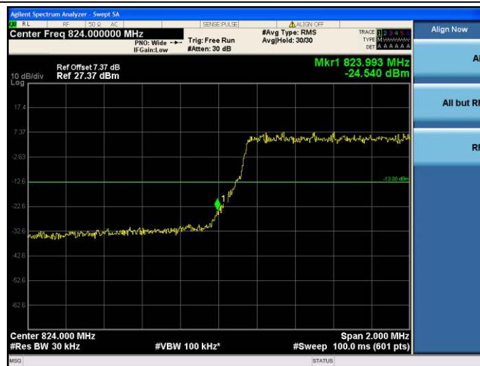
Band5-3MHz-QPSK-20415-15RB#0
