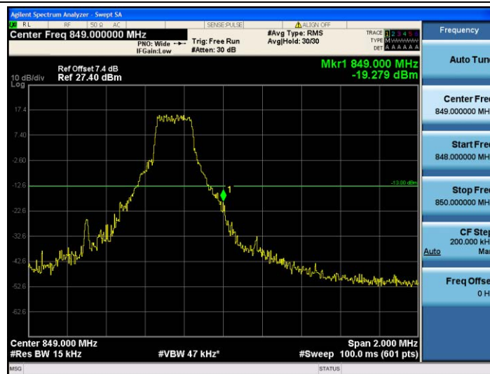
Band5-1.4MHz-16QAM-20643-1RB#5
