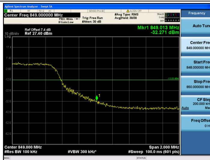
Band5-10MHz-16QAM-20600-50RB#0
