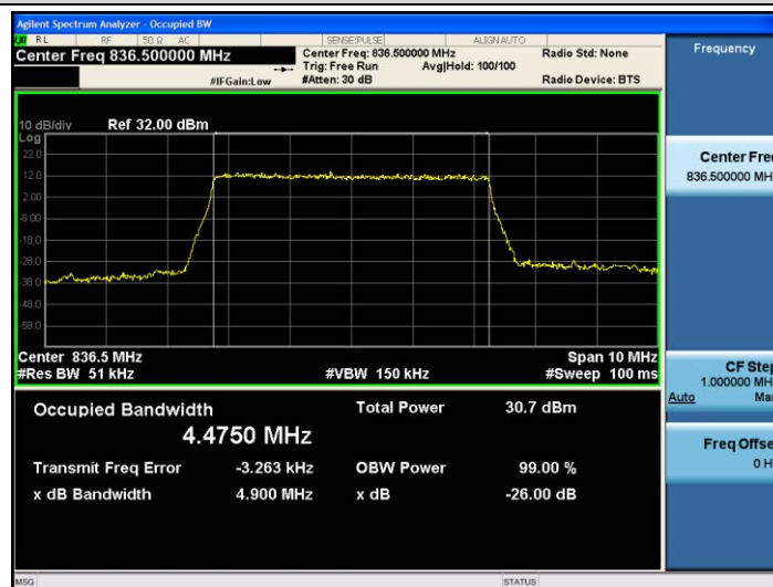
Band5-5MHz-QPSK-20525-25RB#0-4.4750
