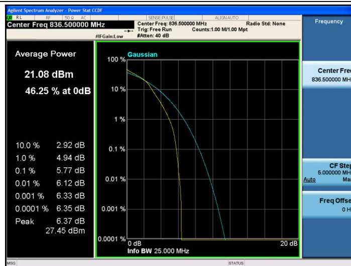
Band5-1.4MHz-16QAM-20525-6RB#0
