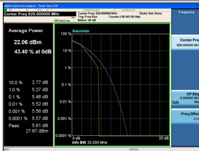
Band5-10MHz-16QAM-20450-1RB#0
