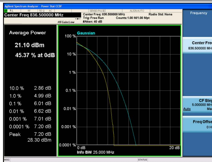
Band5-10MHz-16QAM-20525-50RB#0
