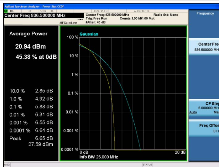
Band5-3MHz-16QAM-20525-15RB#0
