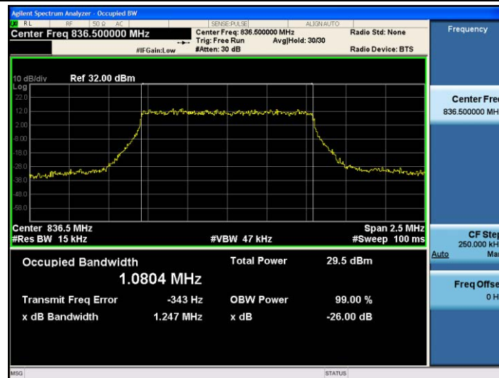
Band5-1.4MHz-QPSK-20525-6RB#0-1.0804
