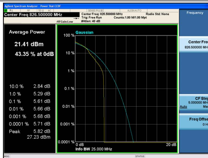
Band5-5MHz-16QAM-20425-1RB#0
