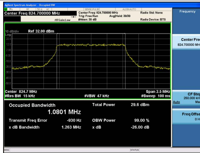
Band5-1.4MHz-QPSK-20407-6RB#0-1.0801
