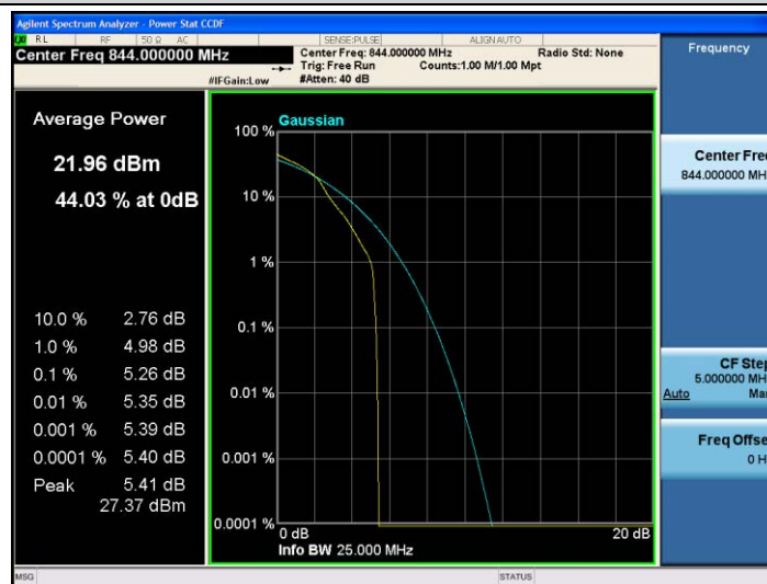
Band5-10MHz-16QAM-20600-1RB#0
