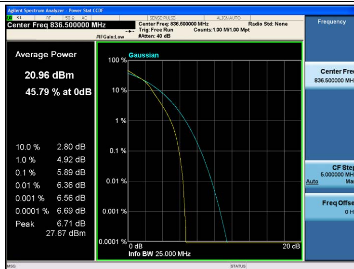
Band5-5MHz-16QAM-20525-25RB#0
