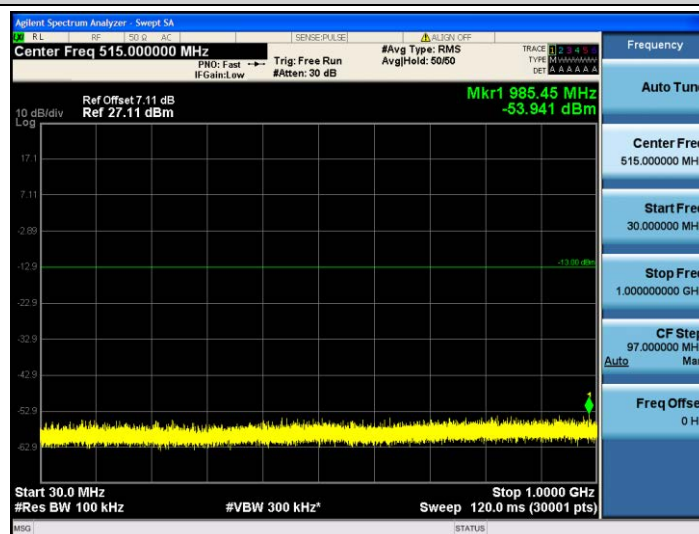
Band4-10MHz-16QAM-20175-1RB#0-30~1000MHz
