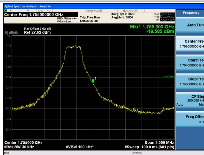
Band4-3MHz-QPSK-20385-1RB#14
