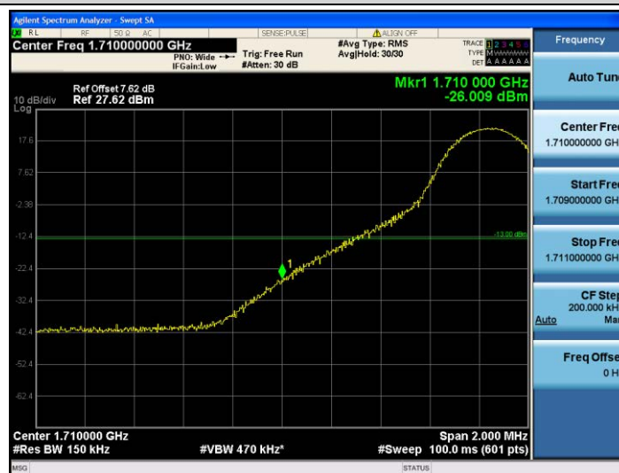
Band4-15MHz-QPSK-20025-1RB#0
