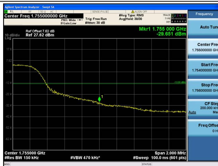
Band4-15MHz-QPSK-20325-75RB#0
