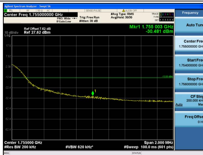
Band4-20MHz-QPSK-20300-100RB#0
