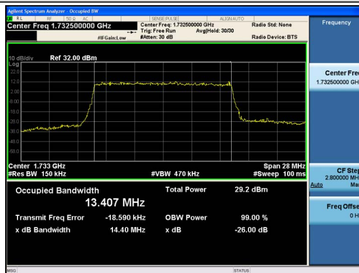
Band4-15MHz-16QAM-20175-75RB#0-13.407
