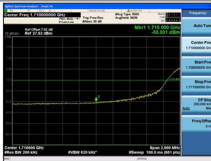
Band4-20MHz-16QAM-20050-100RB#0
