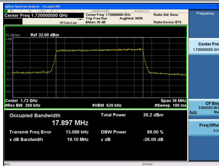
Band4-20MHz-QPSK-20050-100RB#0-17.897
