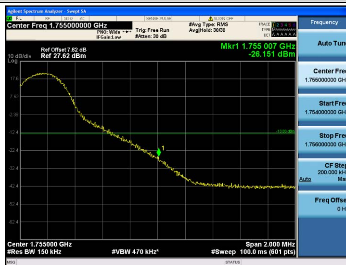
Band4-15MHz-16QAM-20325-1RB#74
