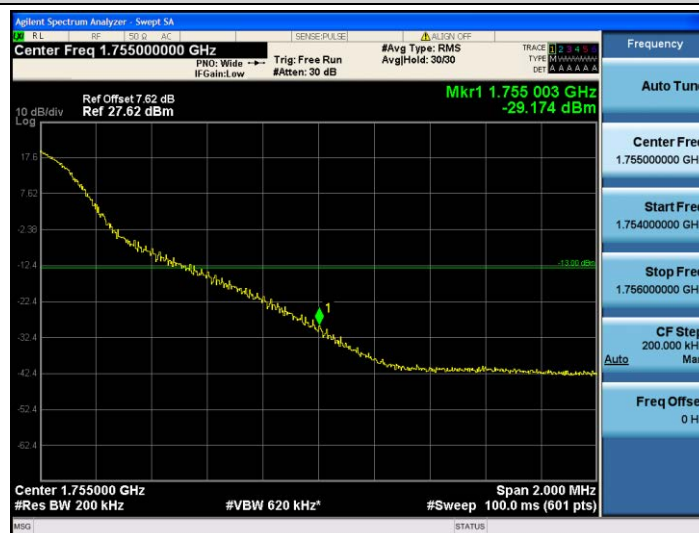
Band4-20MHz-16QAM-20300-1RB#99
