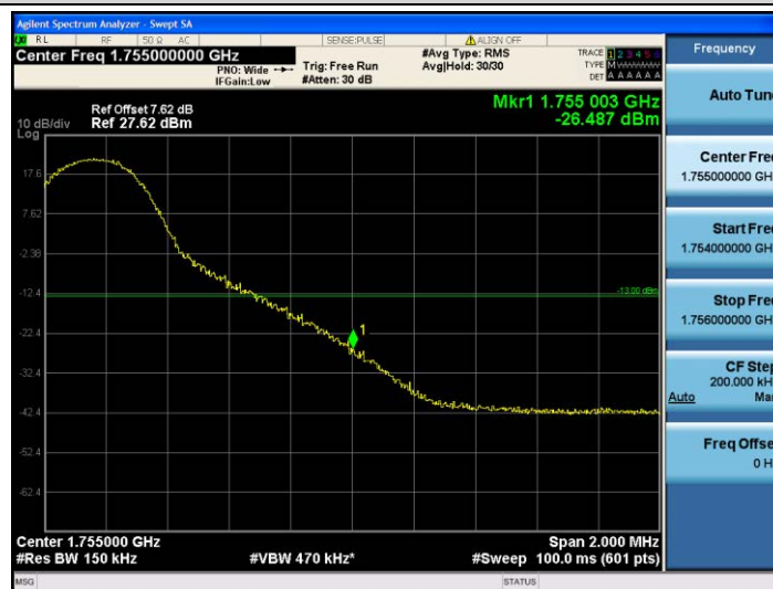
Band4-15MHz-QPSK-20325-1RB#74
