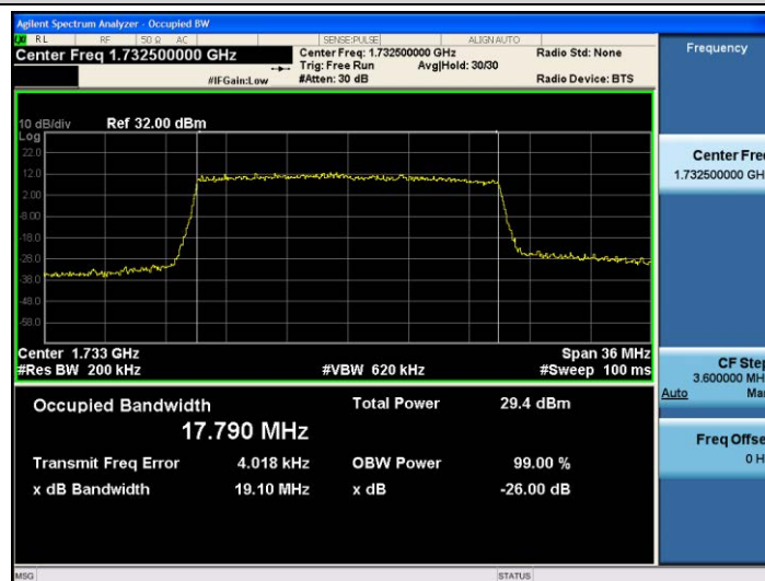
Band4-20MHz-QPSK-20175-100RB#0-17.790
