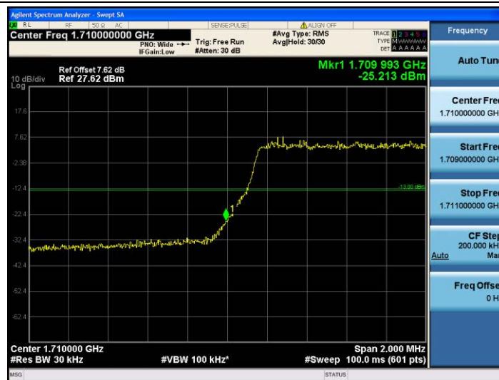
Band4-3MHz-QPSK-19965-15RB#0
