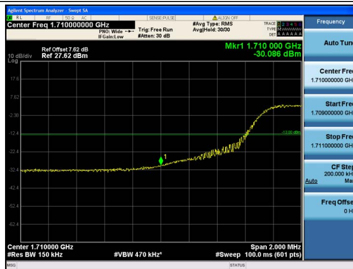
Band4-15MHz-QPSK-20025-75RB#0
