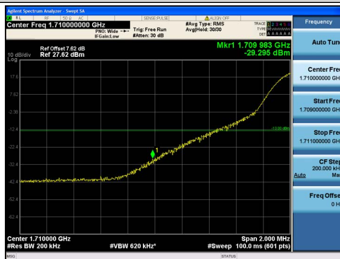
Band4-20MHz-16QAM-20050-1RB#0
