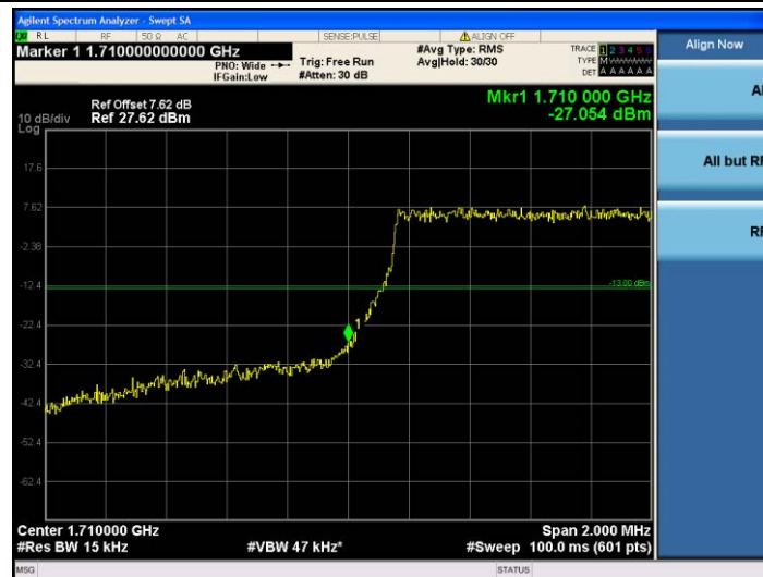
Band4-1.4MHz-QPSK-19957-6RB#0
