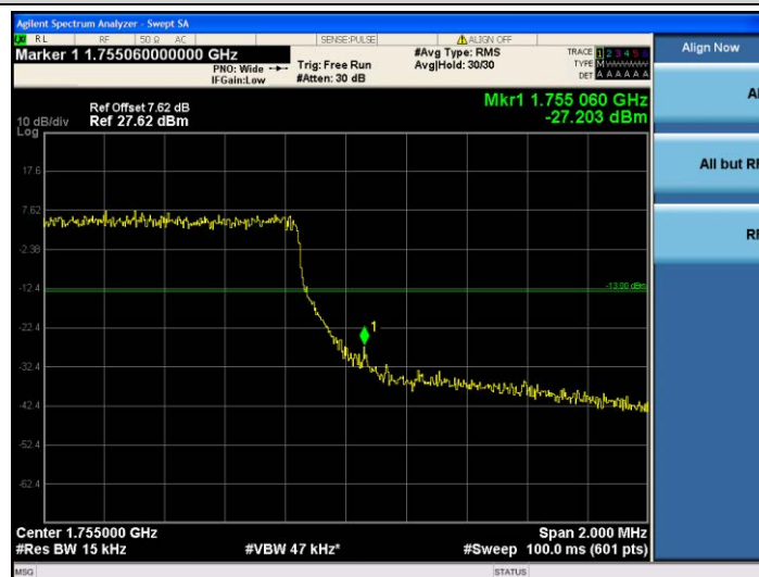
Band4-1.4MHz-16QAM-20393-6RB#0
