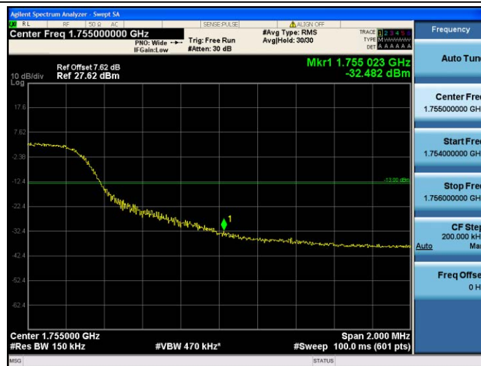
Band4-15MHz-16QAM-20325-75RB#0
