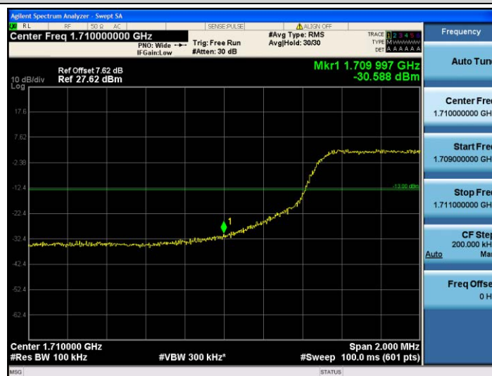
Band4-10MHz-16QAM-20000-50RB#0
