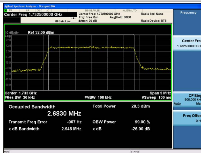
Band4-3MHz-16QAM-20175-15RB#0-2.6830
