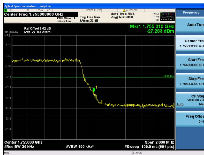
Band4-3MHz-16QAM-20385-15RB#0
