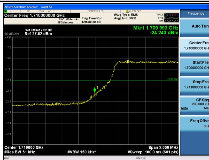
Band4-5MHz-QPSK-19975-25RB#0
