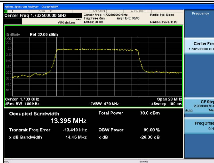
Band4-15MHz-QPSK-20175-75RB#0-13.395
