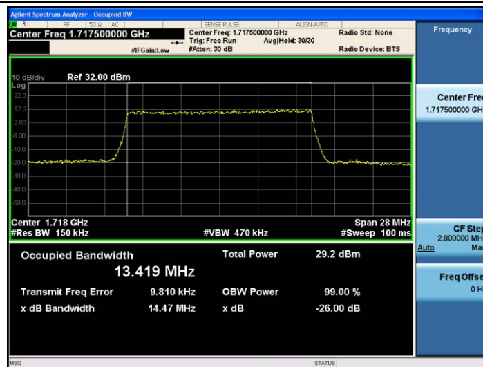
Band4-15MHz-16QAM-20025-75RB#0-13.419
