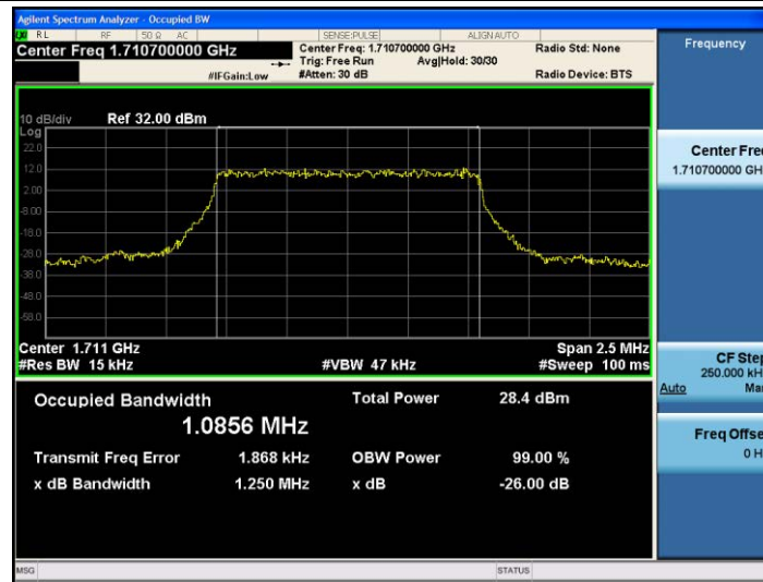
Band4-1.4MHz-QPSK-19957-6RB#0-1.0856
