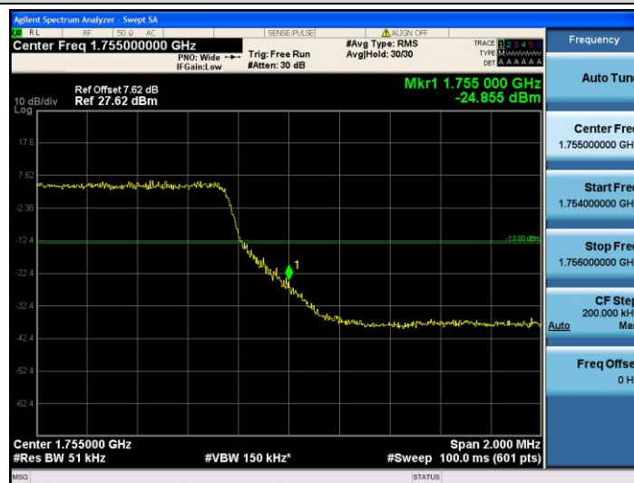
Band4-5MHz-QPSK-20375-25RB#0
