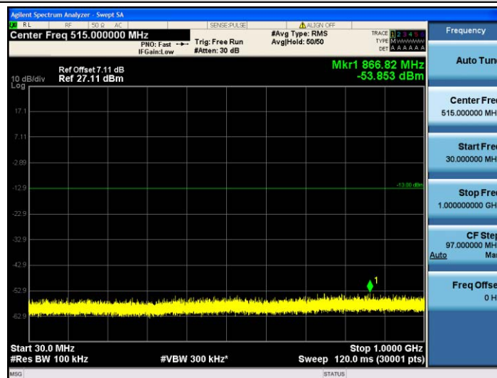
Band4-1.4MHz-16QAM-20175-1RB#0-30~1000MHz
