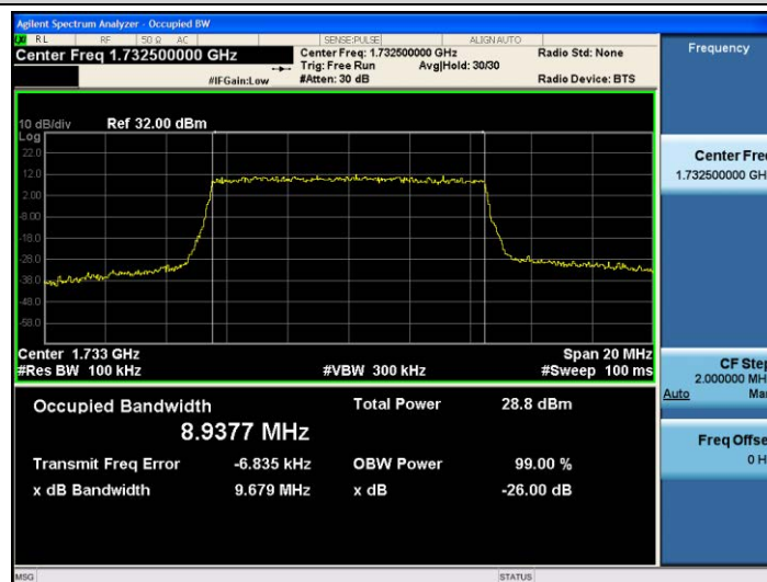
Band4-10MHz-16QAM-20175-50RB#0-8.9377
