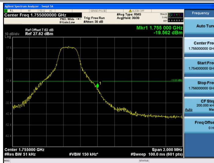
Band4-5MHz-QPSK-20375-1RB#24
