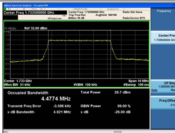
Band4-5MHz-QPSK-20175-25RB#0-4.4774
