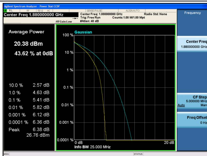
Band2-3MHz-QPSK-18900-15RB#0
