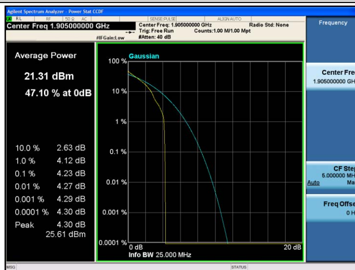
Band2-10MHz-QPSK-19150-1RB#0
