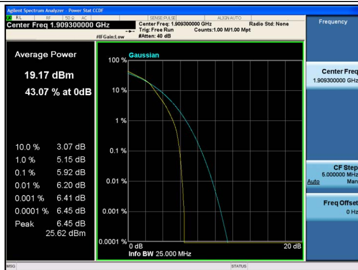
Band2-1.4MHz-16QAM-19193-6RB#0
