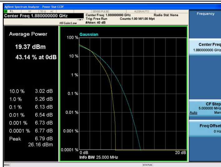
Band2-1.4MHz-16QAM-18900-6RB#0
