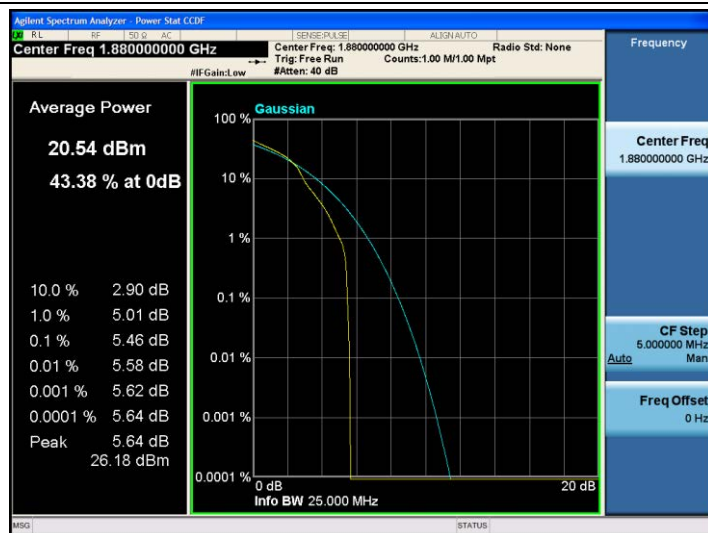
Band2-3MHz-16QAM-18900-1RB#0
