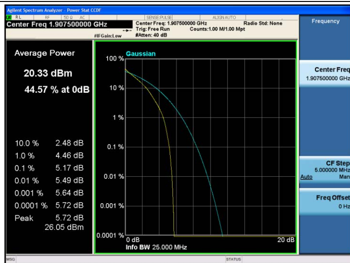
Band2-5MHz-QPSK-19175-25RB#0
