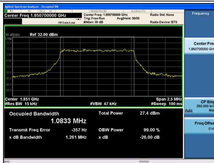
Band2-1.4MHz-16QAM-18607-6RB#0-1.0833
