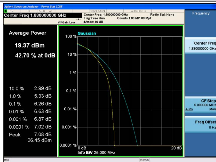
Band2-15MHz-16QAM-18900-75RB#0
