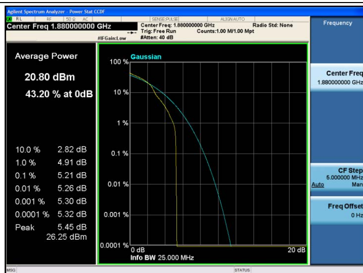
Band2-10MHz-16QAM-18900-1RB#0
