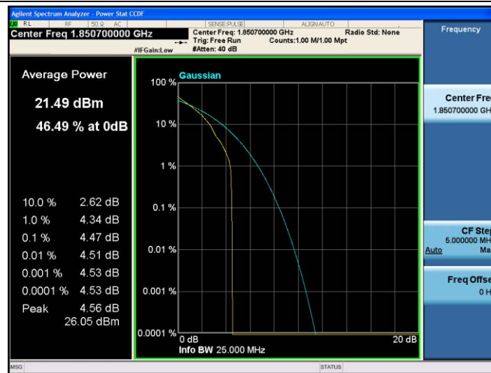
Band2-1.4MHz-QPSK-18607-1RB#0
