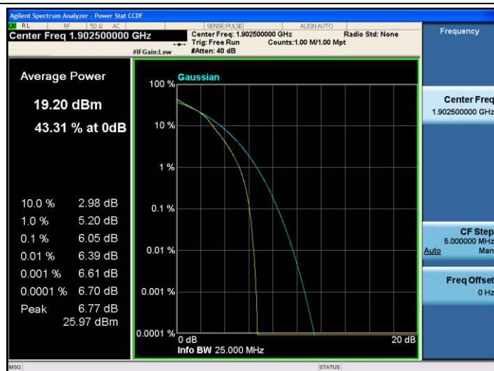
Band2-15MHz-16QAM-19125-75RB#0
