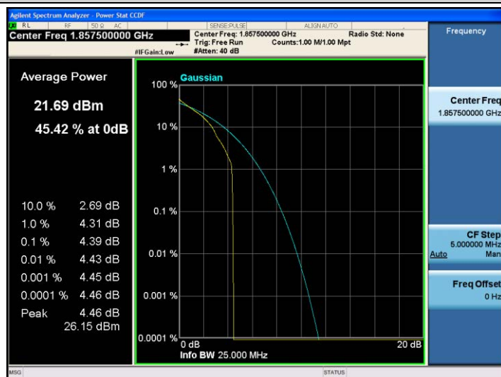
Band2-15MHz-QPSK-18675-1RB#0
