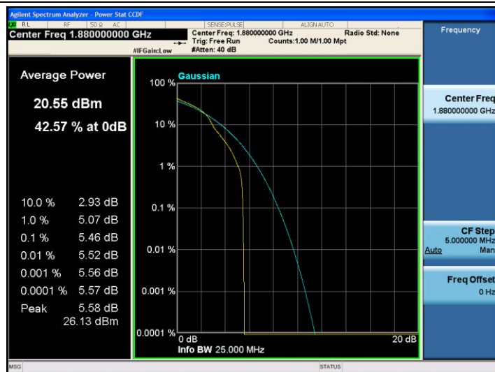
Band2-1.4MHz-16QAM-18900-1RB#0
