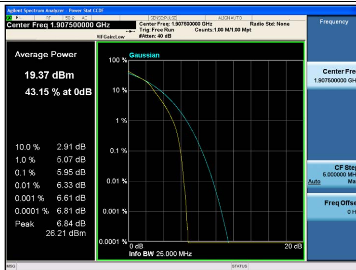
Band2-5MHz-16QAM-19175-25RB#0
