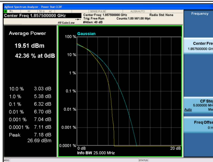
Band2-15MHz-16QAM-18675-75RB#0
