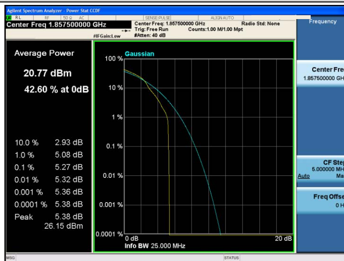
Band2-15MHz-16QAM-18675-1RB#0
