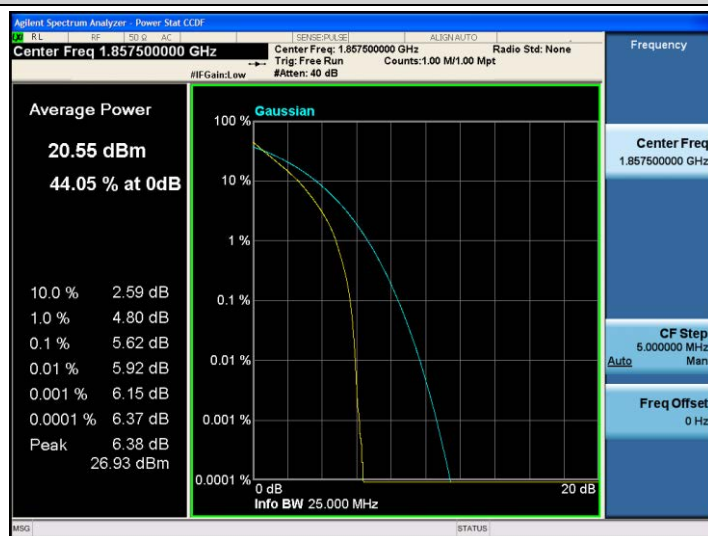
Band2-15MHz-QPSK-18675-75RB#0
