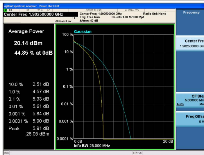
Band2-15MHz-QPSK-19125-75RB#0
