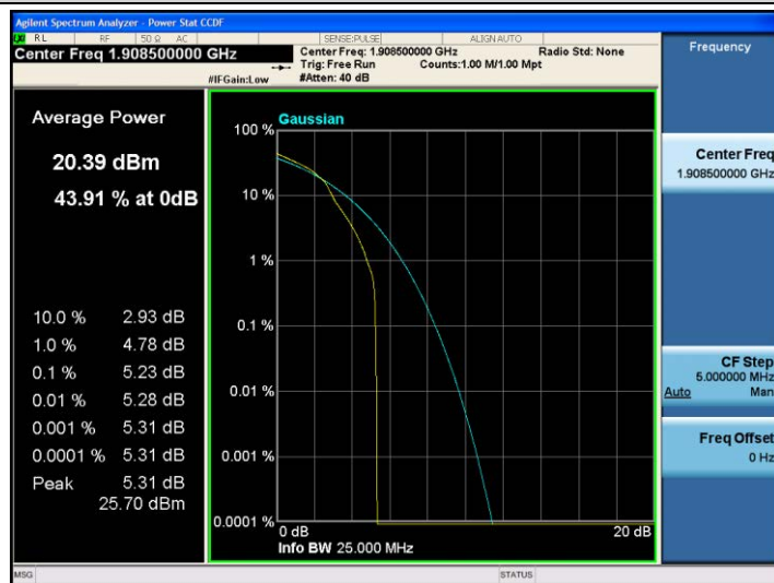
Band2-3MHz-16QAM-19185-1RB#0
