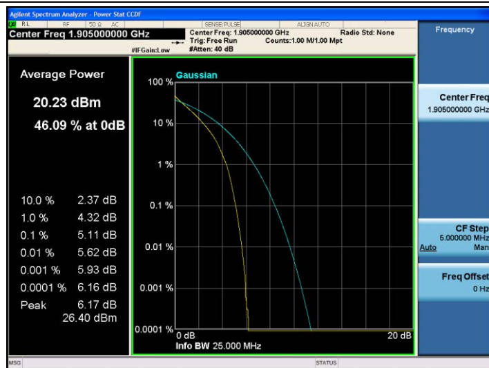
Band2-10MHz-QPSK-19150-50RB#0
