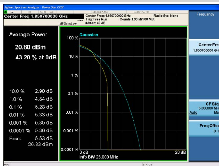
Band2-1.4MHz-16QAM-18607-1RB#0
