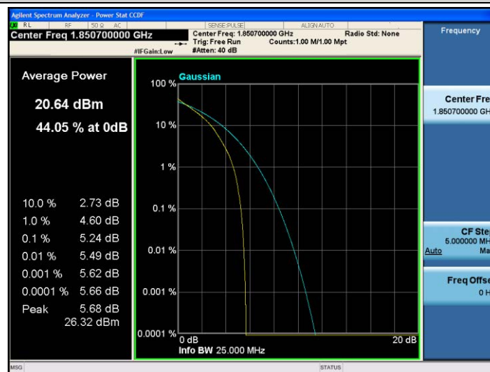
Band2-1.4MHz-QPSK-18607-6RB#0
