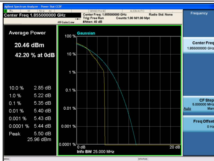
Band2-10MHz-16QAM-18650-1RB#0
