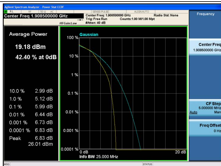
Band2-3MHz-16QAM-19185-15RB#0
