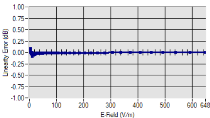
Linearity
