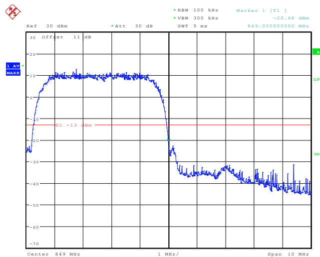
Higher Band Edge Plot on Channel 4233
