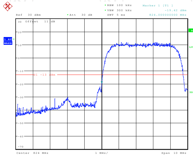
Lower Band Edge Plot on Channel 4132
