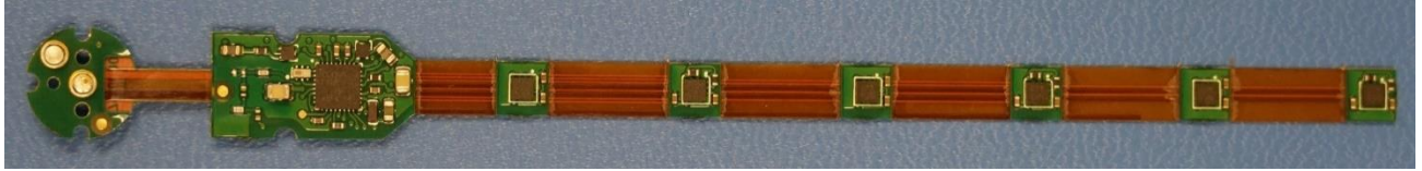
Device PCBA bottom:
