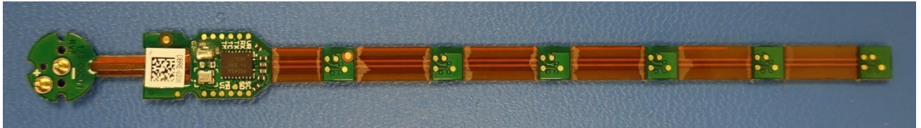
Device PCBA top:
