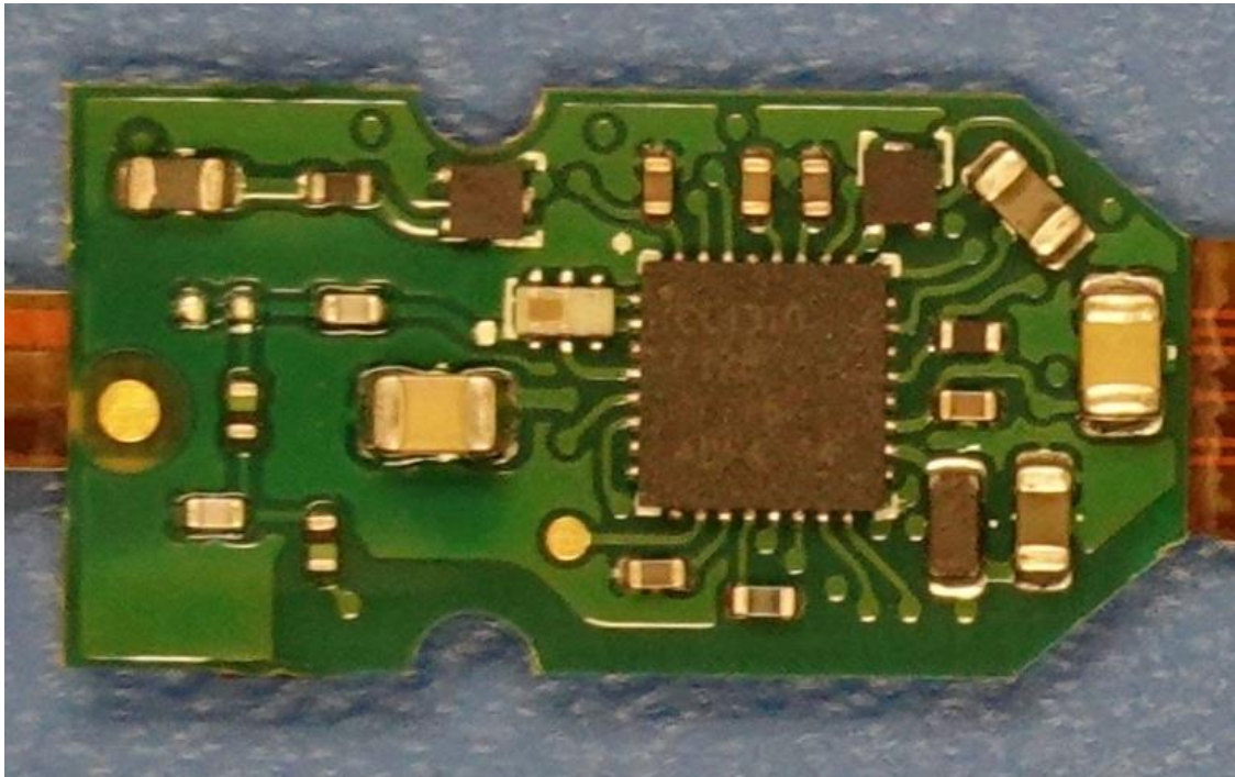
Device transmitter closeup:
