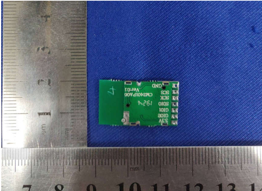
Figure 3 Inside of the EUT
