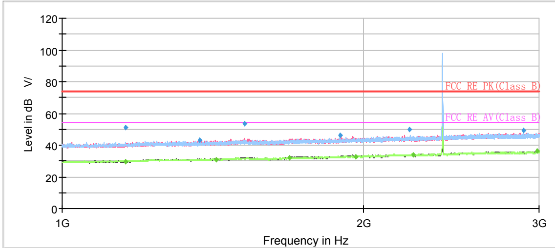
Note: The signal beyond the limit is carrier. Radiates Emission from 1GHz to 3GHz
