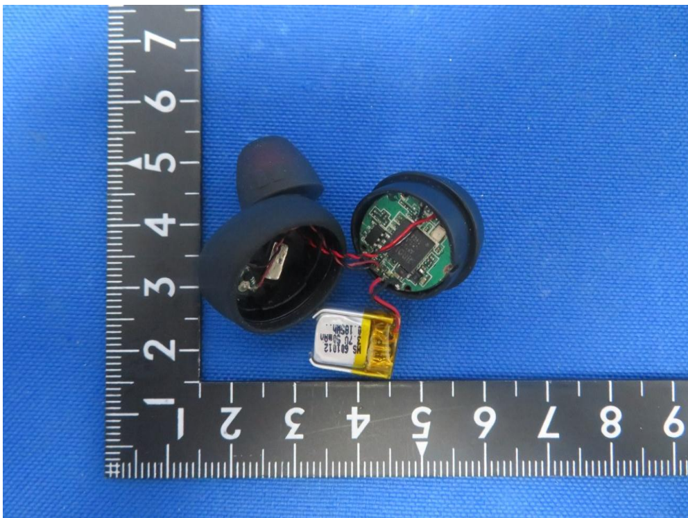
(4) EUT Photo (Right Headphone)
