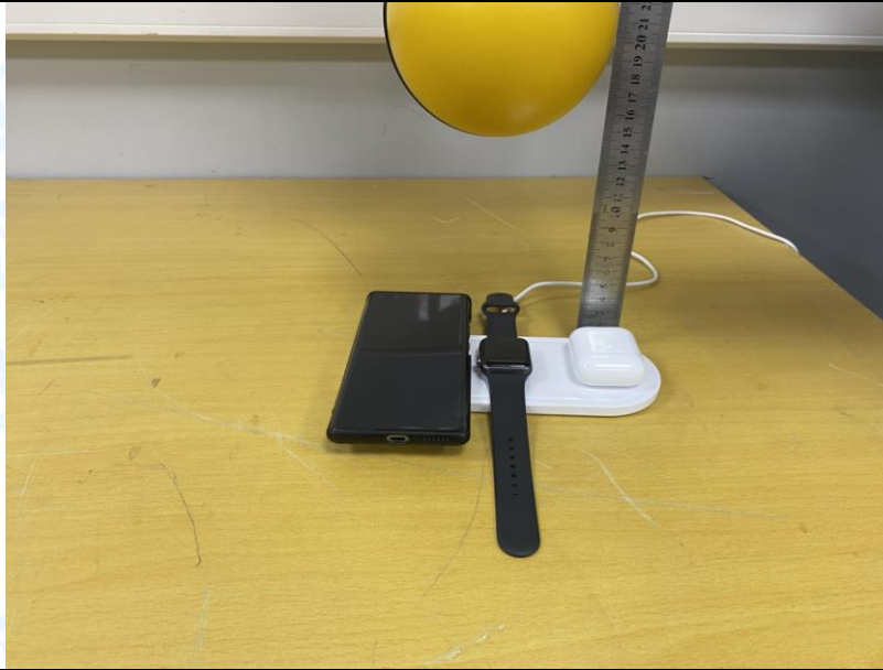
H-Field Strength-20cm (Phone Ant2)
