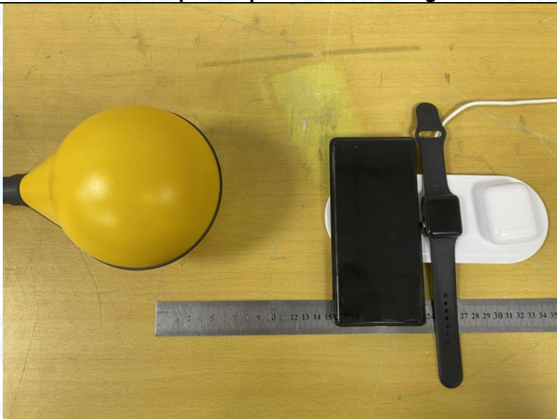
H-Field Strength-15cm Test Position A - Exposure photo from side edge surface-Rear
