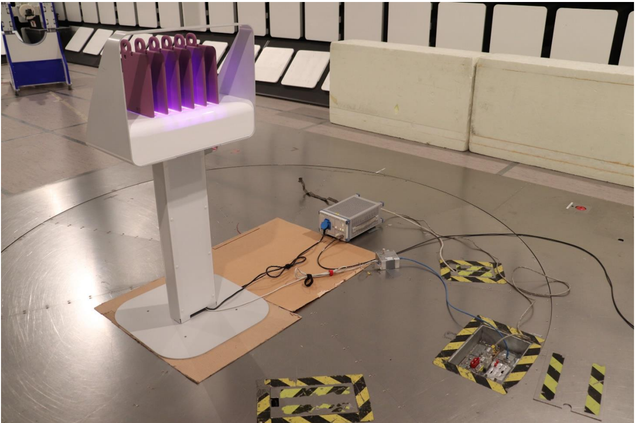
Photograph 3: Conducted emissions AC port (0.150 – 30 MHz)
