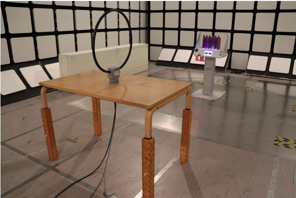
Photograph 1: Transmitter spurious emissions (9 kHz – 30 MHz)
