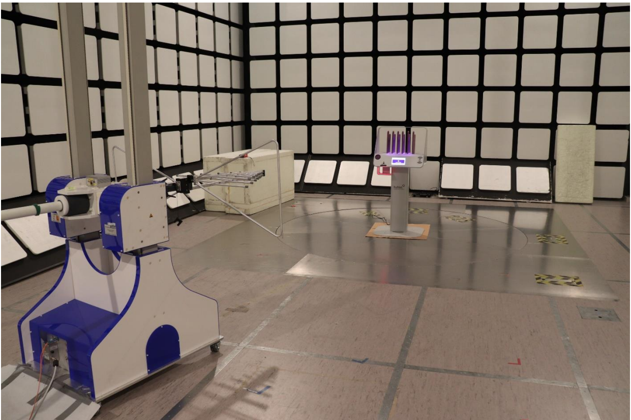
Photograph 2: Transmitter spurious emissions (30 – 1000 MHz)
