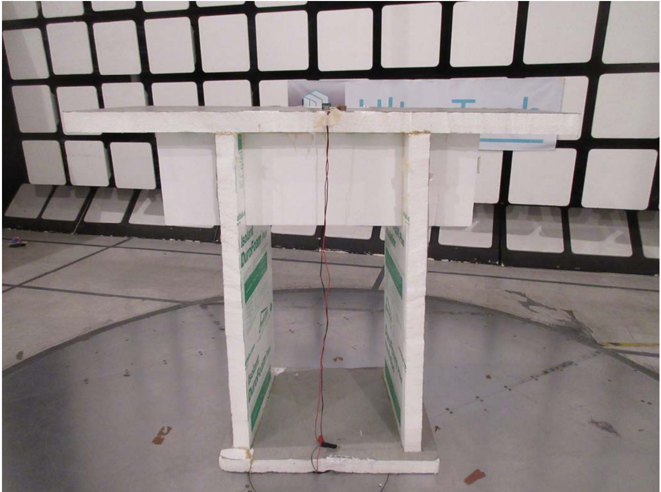
Radiated Emissions at 3 m EUT with 0 dBi \frac{1}{4} Wave Monopole Antenna, Orthogonal Position 2
