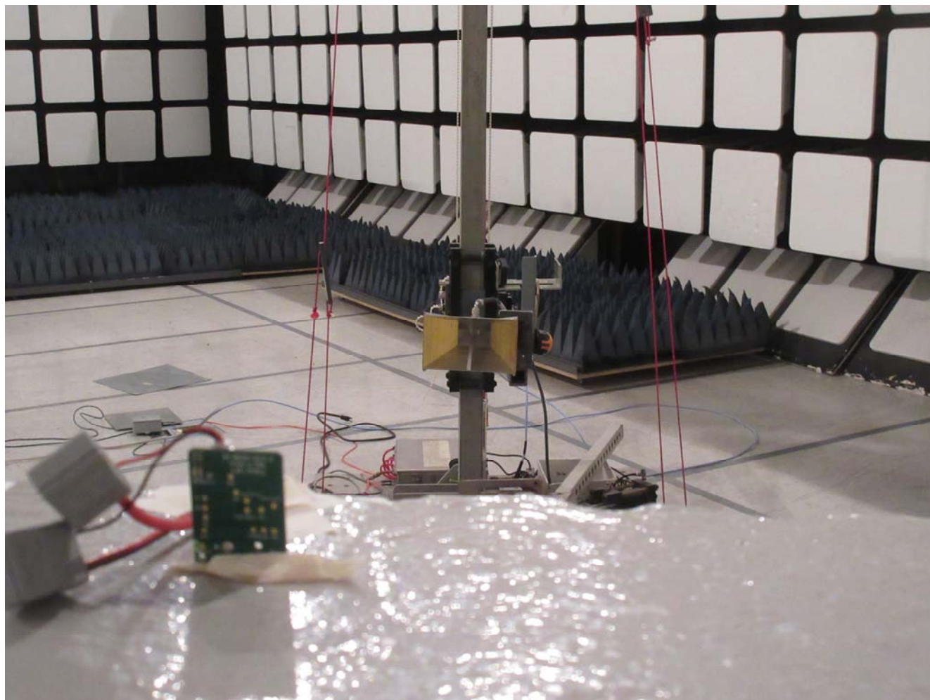
Radiated Emissions at 3 m EUT with 0 dBi \frac{1}{4} Wave Monopole Antenna, Orthogonal Position 3
