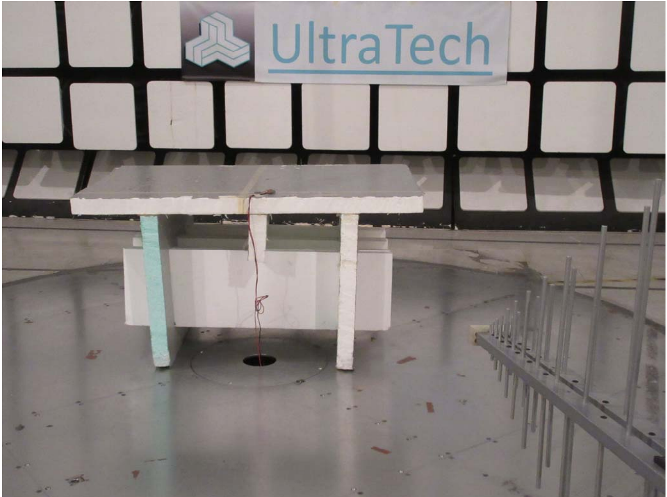
Radiated Emissions at 3 m EUT with 0 dBi \frac{1}{4} Wave Monopole Antenna, Orthogonal Position 1
