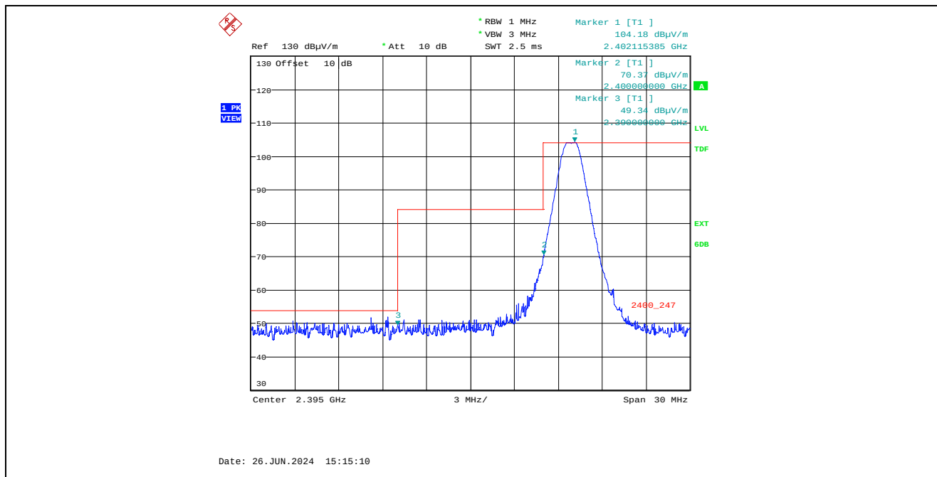
Plot 5.4.4.1.2.1. Radiated Band-Edge Emission at 3 m, Vertical Polarization, Peak Low End of Frequency Band, 2402 MHz, GFSK Modulation, 1M, 1 Mb/s
