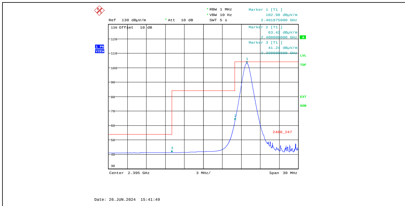
Plot 5.4.4.2.2.2. Radiated Band-Edge Emission at 3 m, Vertical Polarization, Average Low End of Frequency Band, 2402 MHz, GFSK Modulation, Coded PHY, 125 kb/s
