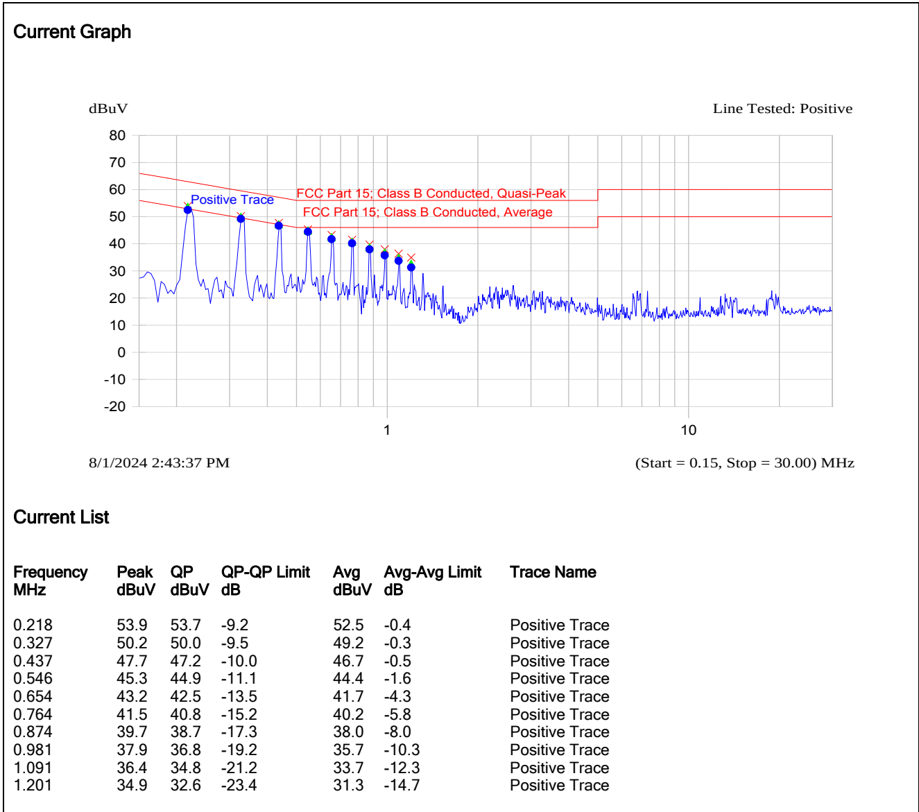
Plot 5.1.4.1. Power Line Conducted Emissions (BLE Tx Mode) Line Voltage: 3.6 VDC; Line Tested: Positive Trace
