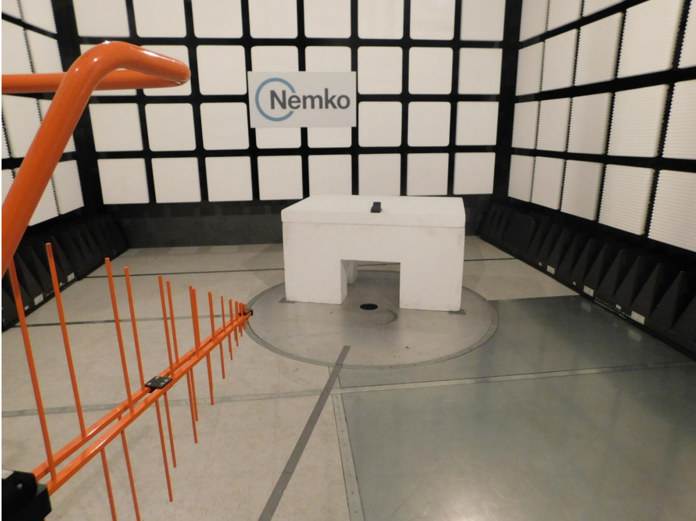
Figure 1.1-1: Below 1 GHz setup
