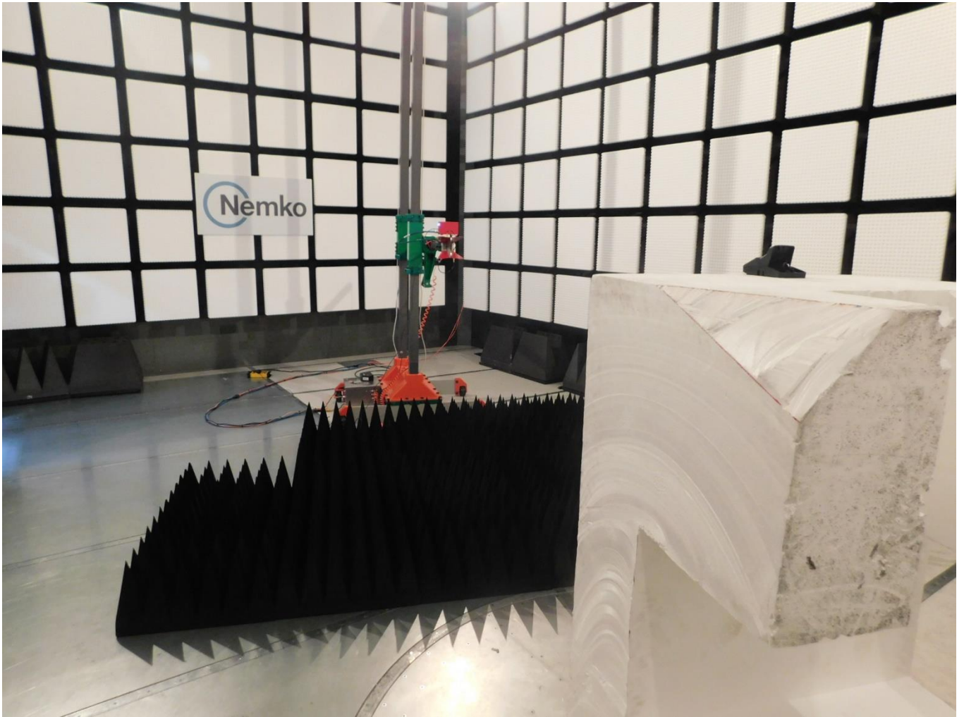
Figure 1.1-2: Above 1 GHz setup
