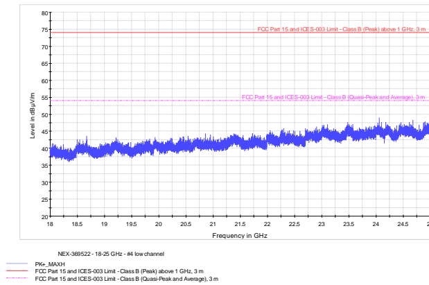
Figure 8.6-7: Radiated spurious emissions low channel 18-25 GHz
