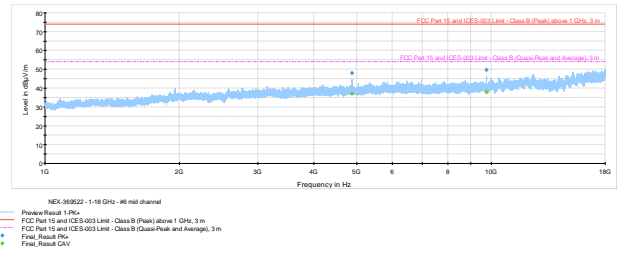
Figure 8.6-9: Radiated spurious emissions mid channel 1-18 GHz
