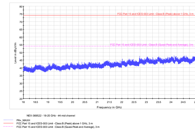
Figure 8.6-10: Radiated spurious emissions mid channel 18-25 GHz
