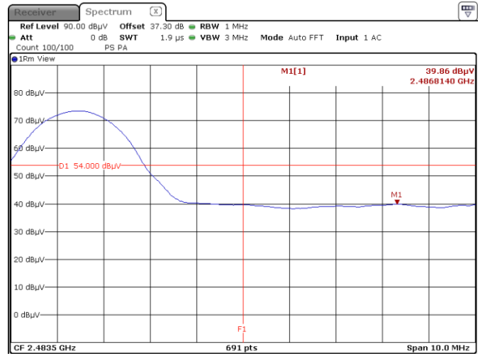
Figure 8.6-4: Radiated spurious emissions upper edge avg
