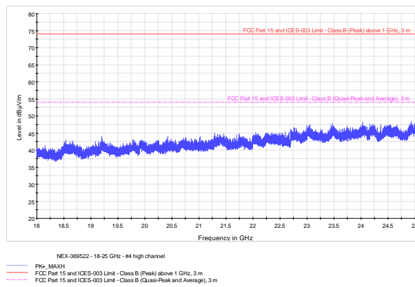
Figure 8.6-13: Radiated spurious emissions high channel 18-25 GHz
