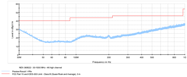
Figure 8.6-11: Radiated spurious emissions high channel 30-1000 MHz
