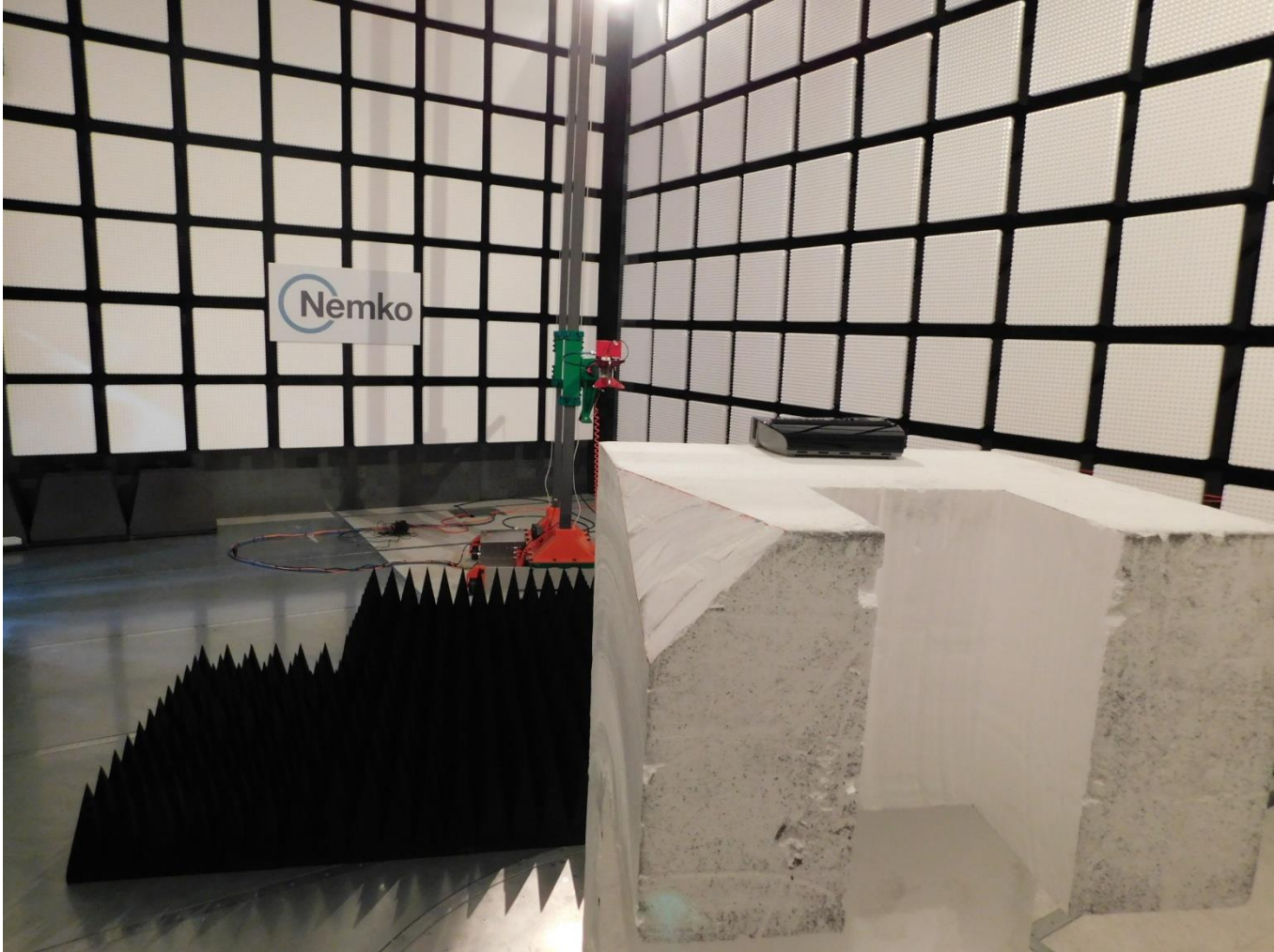
Figure 1.1-1: Above 1 GHz setup
