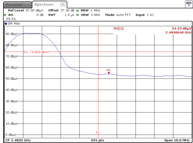
Figure 8.6-2: Radiated spurious emissions upper edge peak
