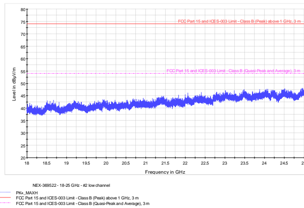
Figure 8.6-7: Radiated spurious emissions low channel 18-25 GHz
