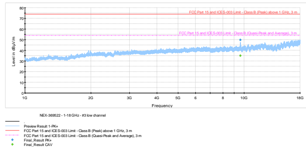
Figure 8.6-6: Radiated spurious emissions low channel 1-18 GHz
