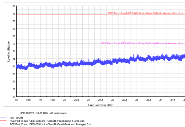
Figure 8.6-10: Radiated spurious emissions mid channel 18-25 GHz
