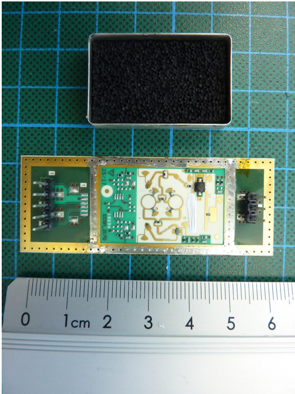
181709_c.jpg: K_LC6, rear view (shielding removed)
