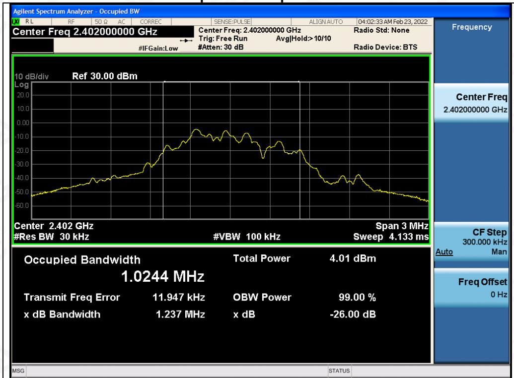
Test_Graph_LE1M_ANT1_2402_1Mbps_OBW
