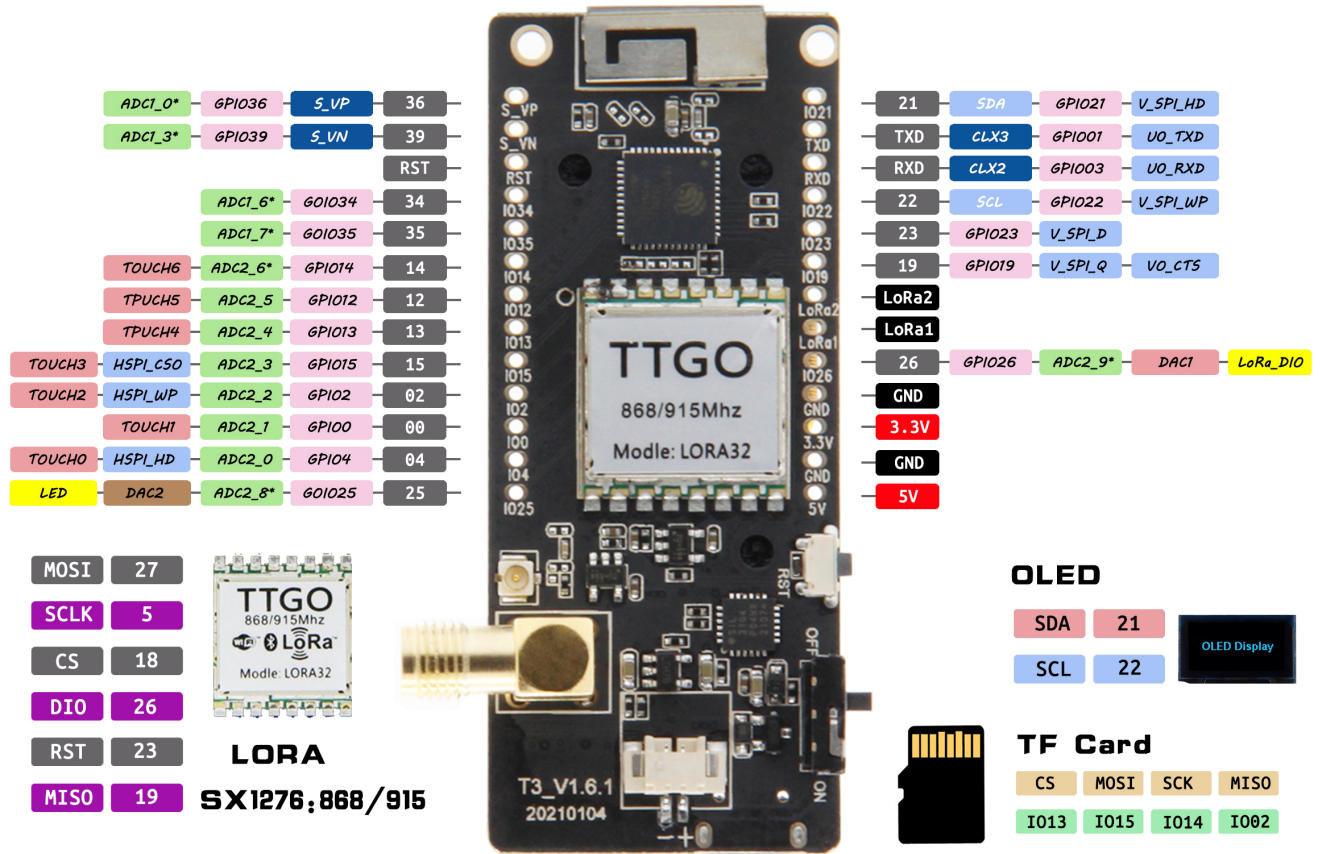
WiFi+Buletooth Lora Board LILYGO T3_V1.6.1
