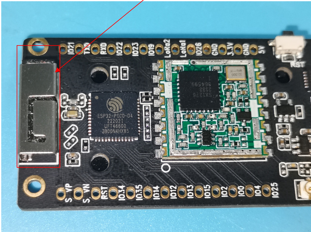
BT/Wi-Fi Antenna
